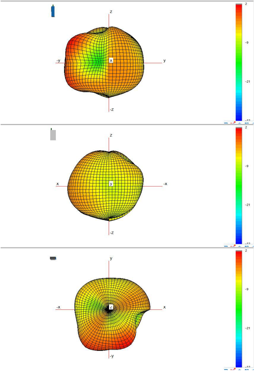
3D Radiation Pattern @ 2440 MHz
