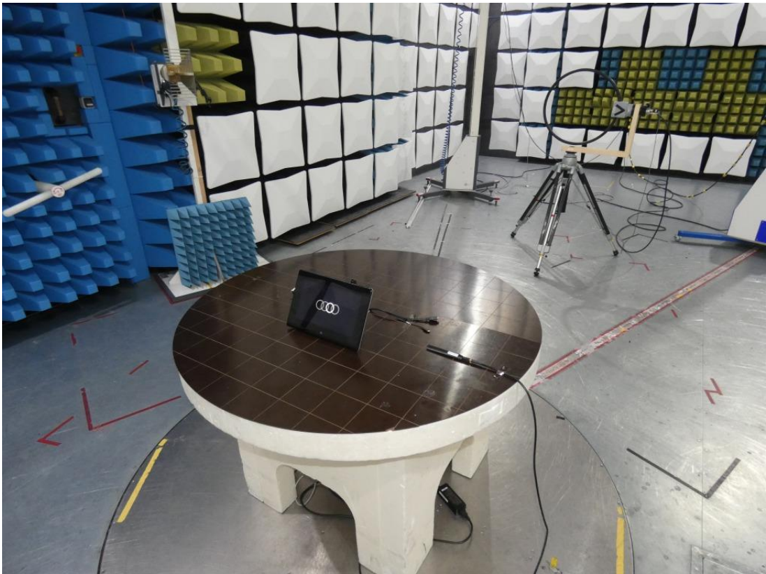
Photo 1: Test setup for H-field measurements below 30 MHz
