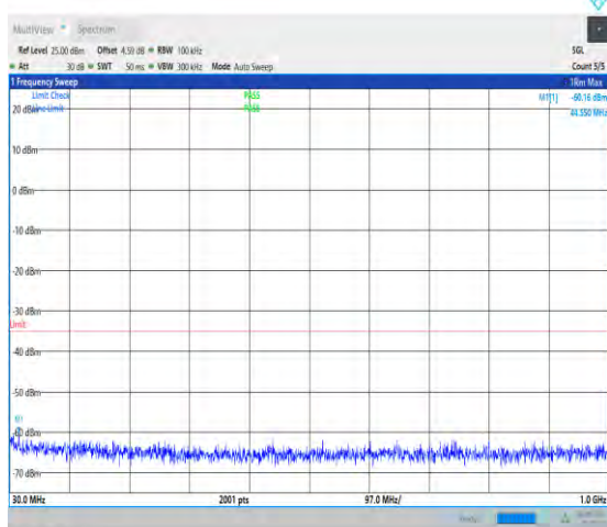
1-N41-PC2-30-100-H-1-DFT-PI2BPSK-Inner_1RB_L eft-1@1-30-1000-Ant1--60.16--35-PASS
