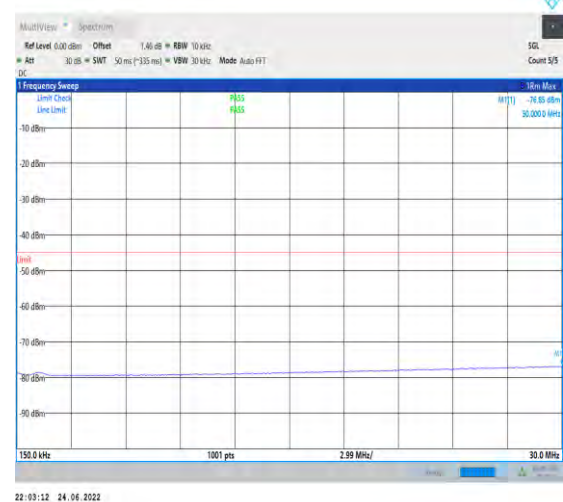
1-N41-PC2-30-100-M-1-DFT-PI2BPSK-Inner_1RB_L eft-1@1-0.15-30-Ant1--76.85--45-PASS
