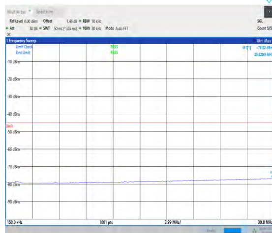
1-N41-PC2-30-100-H-1-DFT-PI2BPSK-Inner_1RB_L eft-1@1-0.15-30-Ant1--76.82--45-PASS
