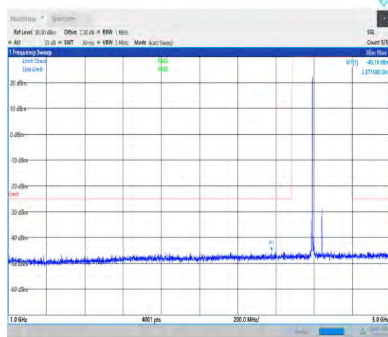
1-N41-PC2-30-100-H-1-DFT-PI2BPSK-Inner_1RB_L eft-1@1-1000-3000-Ant1--45.19--25-PASS
