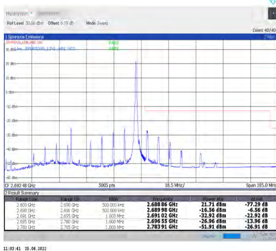
1-N41-PC2-30-90-H-5-CP-QPSK-Edge_1RB_Right-1@244-Ant1-PASS-see graph
