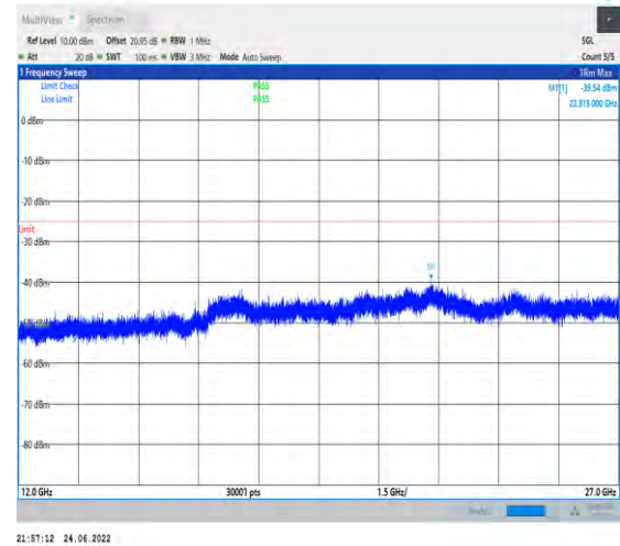
1-N41-PC2-30-100-L-1-DFT-PI2BPSK-Inner_1RB_L eft-1@1-12000-27000-Ant1--39.54--25-PASS
