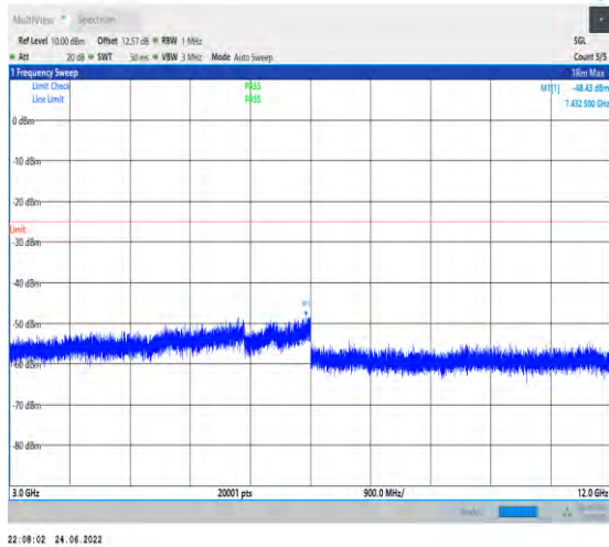
1-N41-PC2-30-100-H-1-DFT-PI2BPSK-Inner_1RB_L eft-1@1-3000-12000-Ant1--48.43--25-PASS
