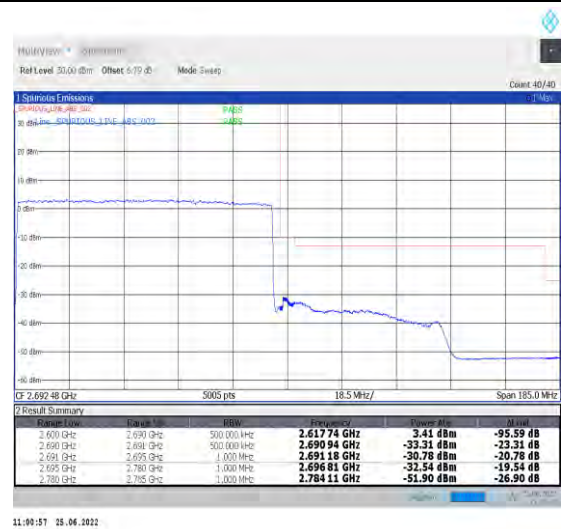
1-N41-PC2-30-90-H-3-DFT-PI2BPSK-Outer_Full-240@0-Ant1-PASS-see graph
