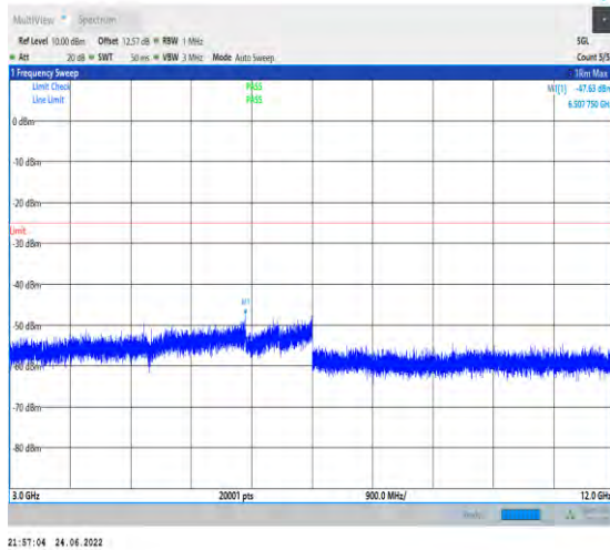
1-N41-PC2-30-100-L-1-DFT-PI2BPSK-Inner_1RB_L eft-1@1-3000-12000-Ant1--47.63--25-PASS
