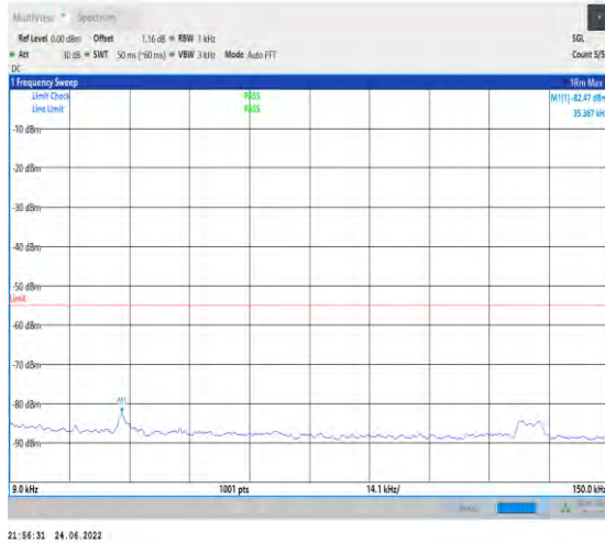
1-N41-PC2-30-100-L-1-DFT-PI2BPSK-Inner_1RB_L eft-1@1-0.009-0.15-Ant1--82.47--55-PASS
