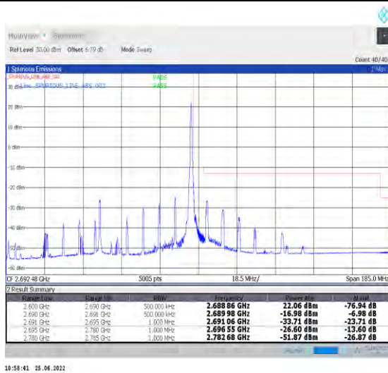
1-N41-PC2-30-90-H-2-DFT-PI2BPSK-Edge_1RB_Right-t1@244-Ant1-PASS-see graph
