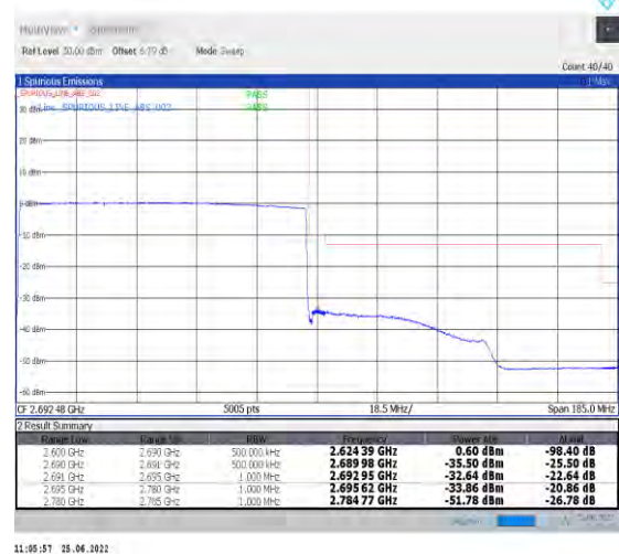
1-N41-PC2-30-90-H-6-CP-QPSK-Outer_Full-245@0-Ant1-PASS-see graph
