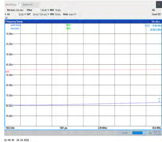
1-N41-PC2-30-100-L-1-DFT-PI2BPSK-Inner_1RB_L eft-1@1-0.15-30-Ant1--76.86--45-PASS
