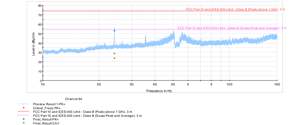
Figure 8.8-13: Radiated spurious emissions 1 - 18 GHz high channel, 802.11a
