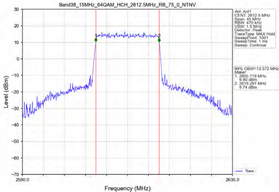
Band38_15MHz_64QAM_HCH_2612.5MHz_RB_75_0_NTNV
