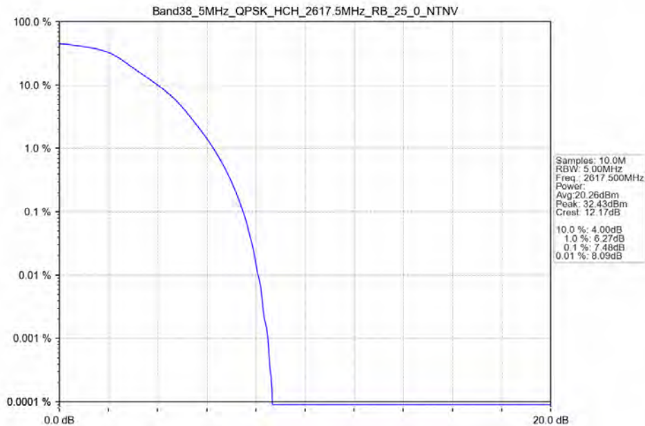
Band38_5MHz_QPSK_HCH_2617.5MHz_RB_25_0_NTNV
