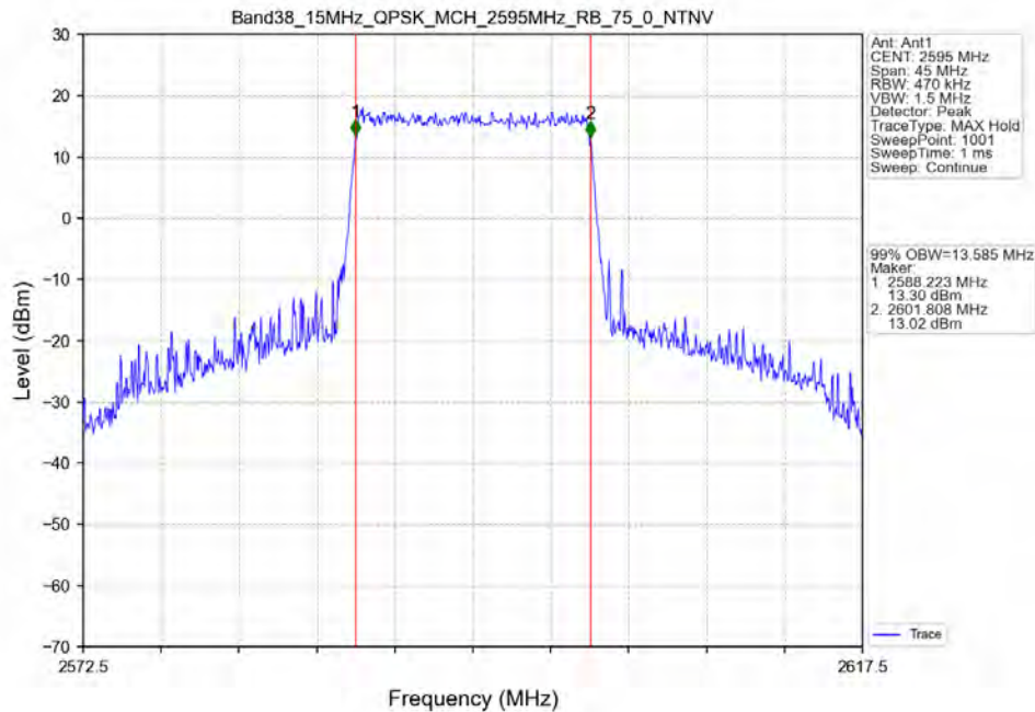
Band38_15MHz_QPSK_MCH_2595MHz_RB_75_0_NTNV
