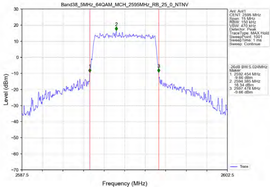
Band38_5MHz_64QAM_MCH_2595MHz_RB_25_0_NTNV
