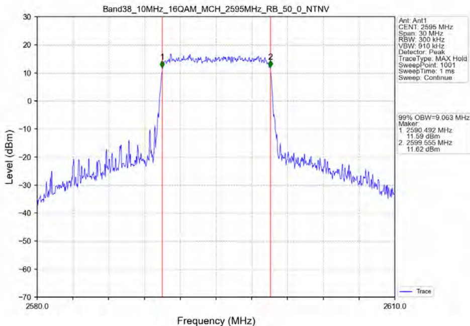
Band38_10MHz_16QAM_MCH_2595MHz_RB_50_0_NTNV
