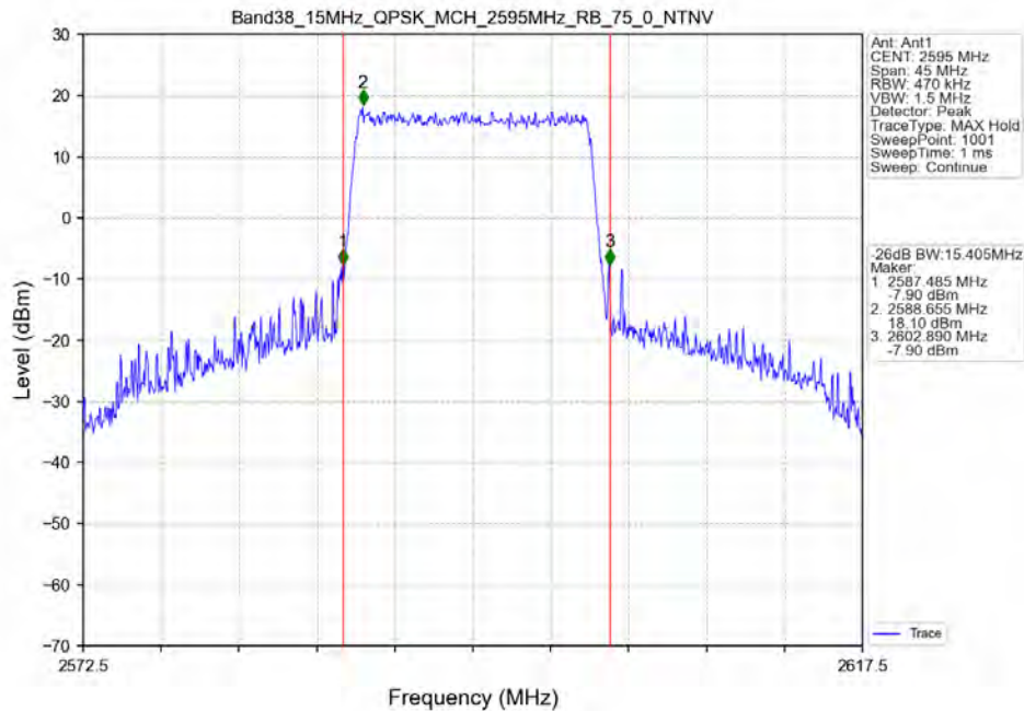
Band38_15MHz_QPSK_MCH_2595MHz_RB_75_0_NTNV
