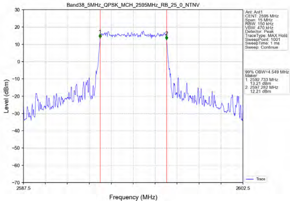
Band38_5MHz_QPSK_MCH_2595MHz_RB_25_0_NTNV
