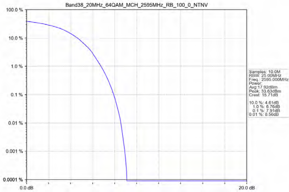
Band38_20MHz_64QAM_MCH_2595MHz_RB_100_0_NTNV
