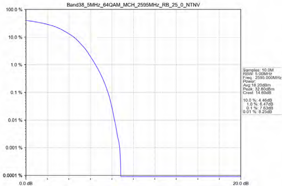
Band38_5MHz_64QAM_MCH_2595MHz_RB_25_0_NTNV
