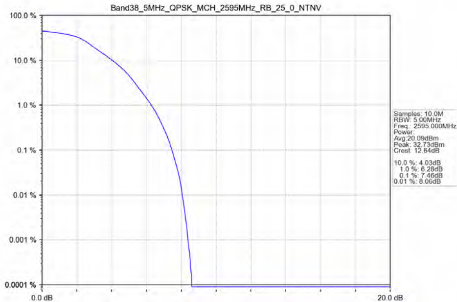
Band38_5MHz_QPSK_MCH_2595MHz_RB_25_0_NTNV
