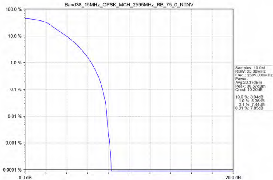
Band38_15MHz_QPSK_MCH_2595MHz_RB_75_0_NTNV
