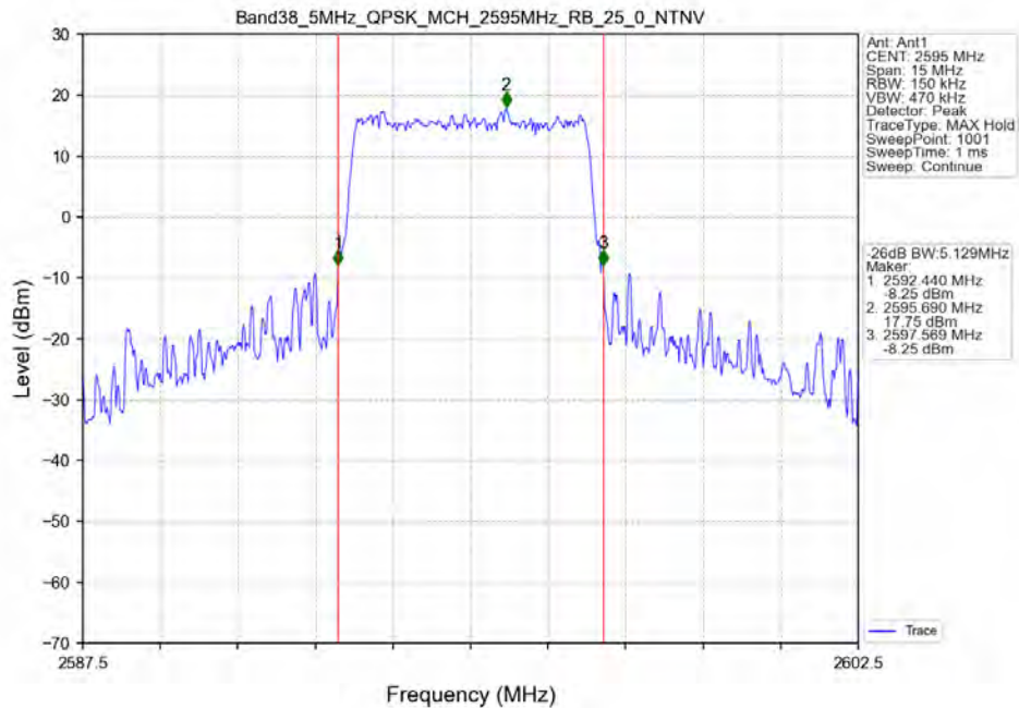
Band38_5MHz_QPSK_MCH_2595MHz_RB_25_0_NTNV
