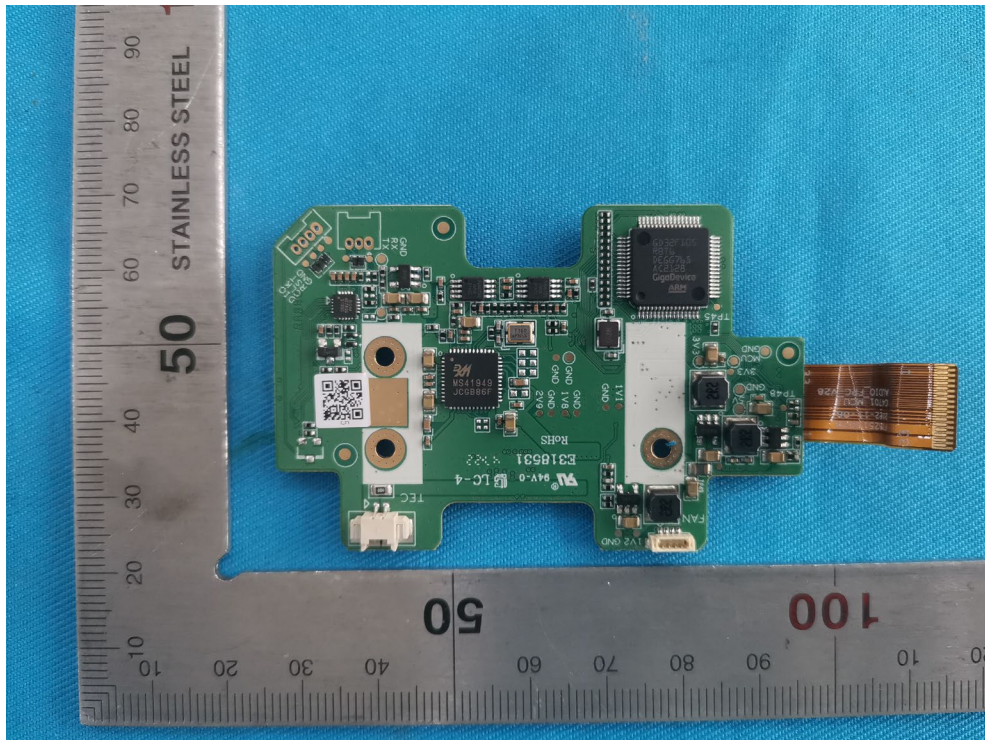
LENS Motor Board Front
