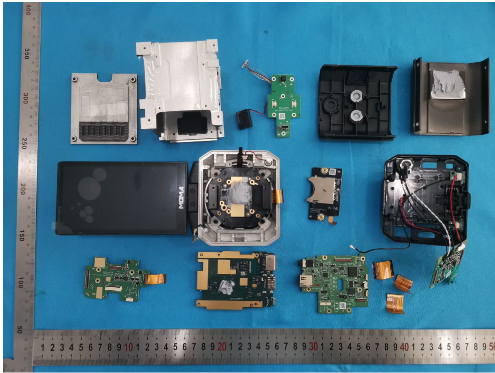
Internal Structure
