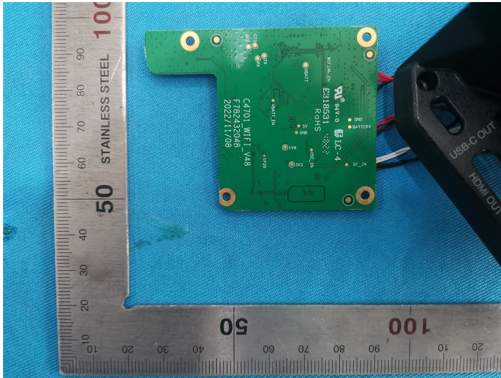
DC Power Board Back
