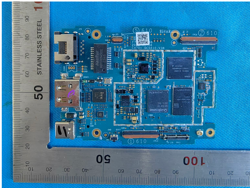
Mainboard Front
