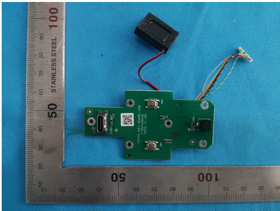
KEY Board Front
