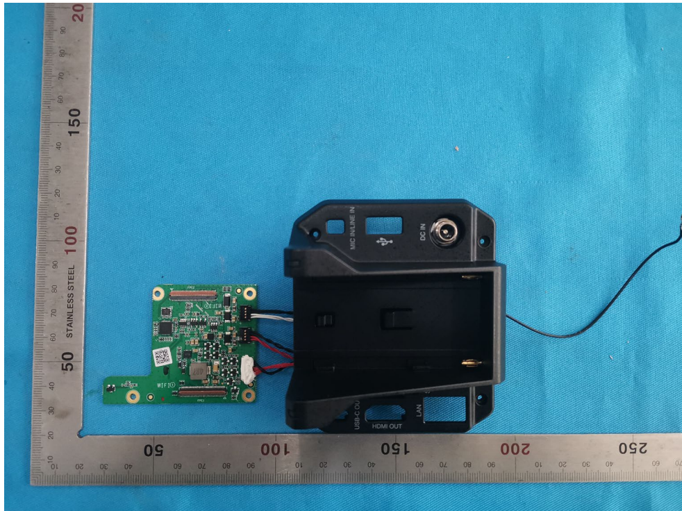
DC Power Board Front
