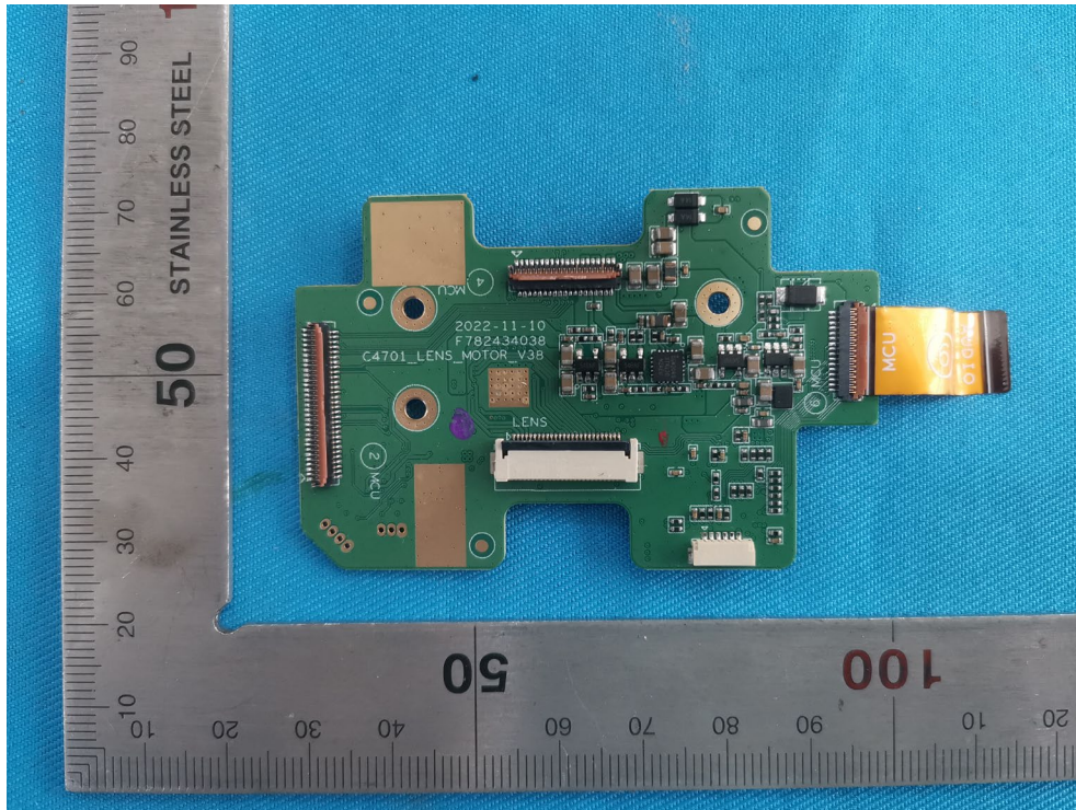
LENS Motor Board Back
