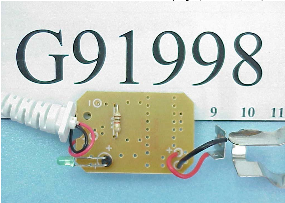
Photos 11 (Plug #2) PC Board, Component Side
