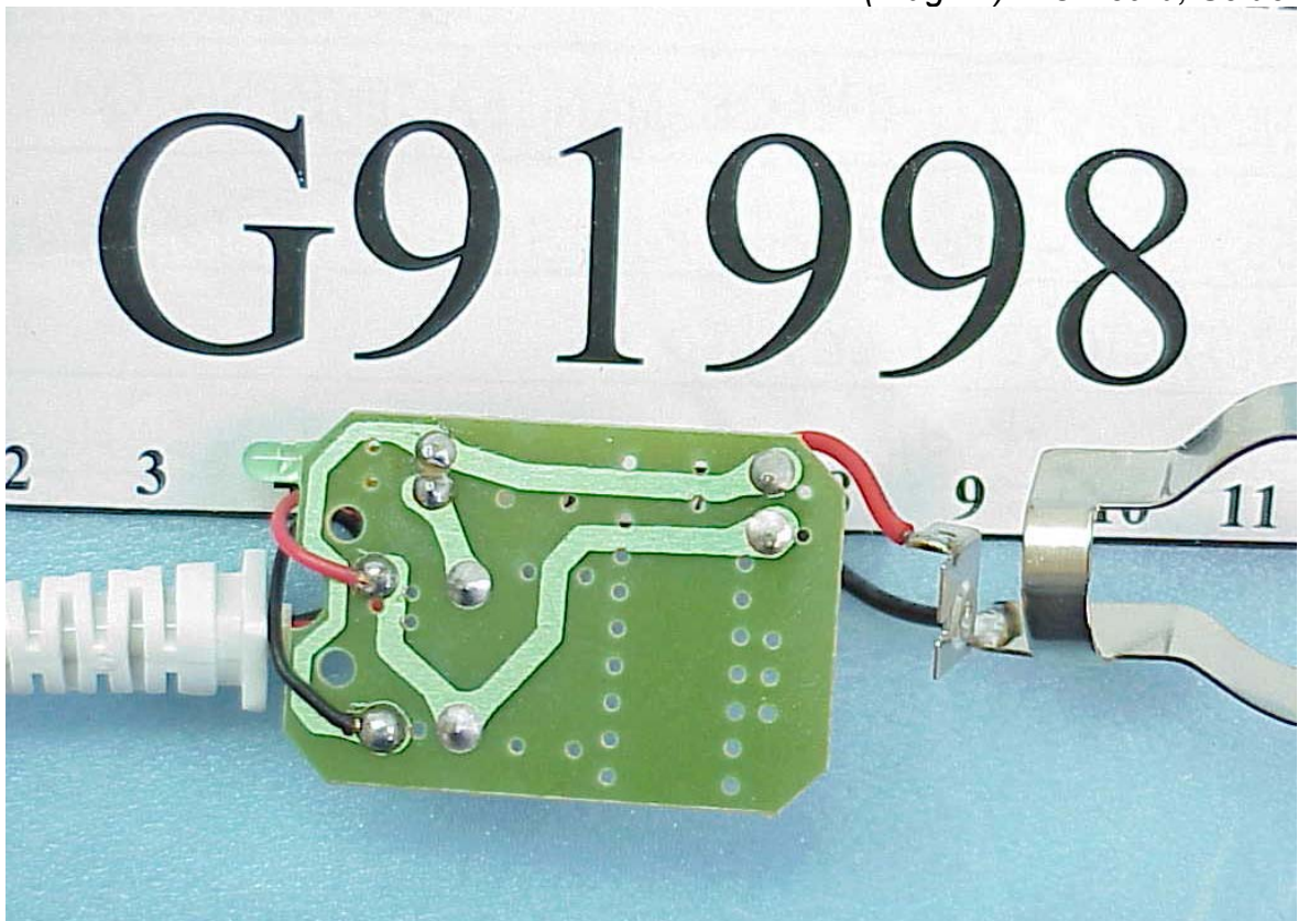
Photos 12 (Plug #2) PC Board, Solder Side
