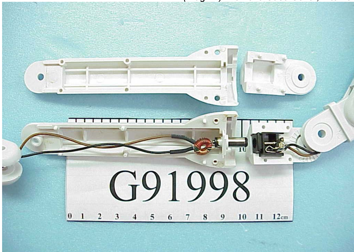
Photos 4 (Plug #1) Remove Case Cover, Internal View
