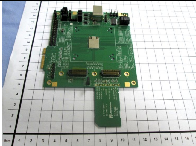
Front Face
