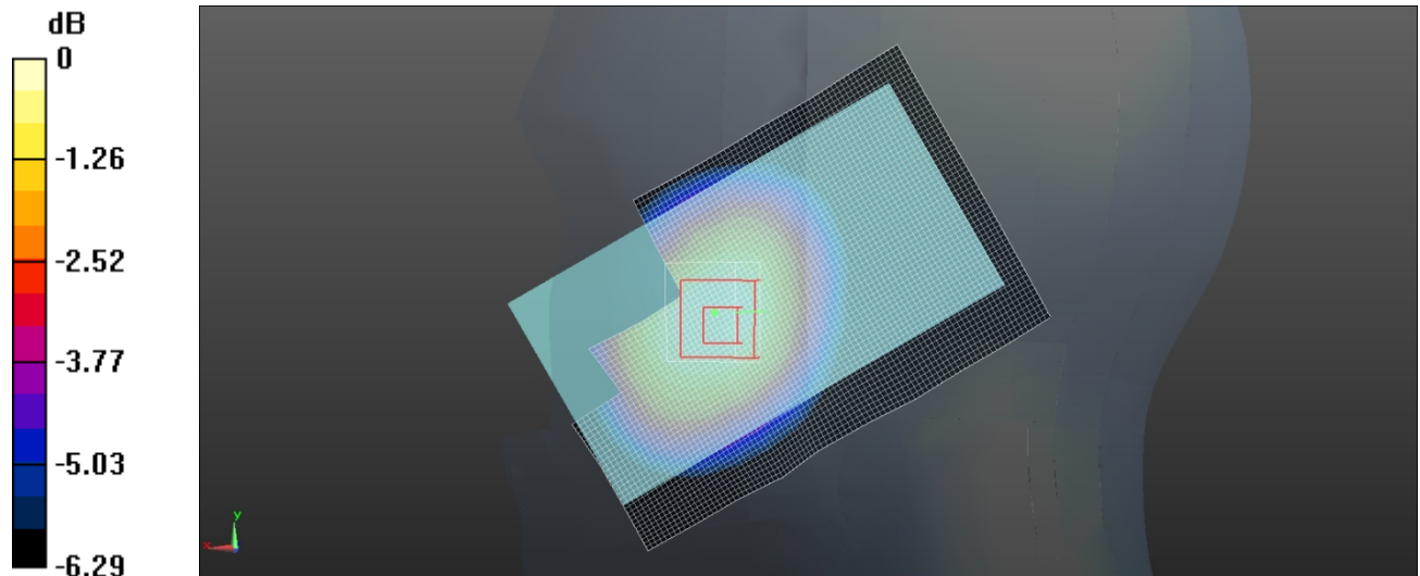
Left Head Cheek (LTE Band 17 Middle Channel)
