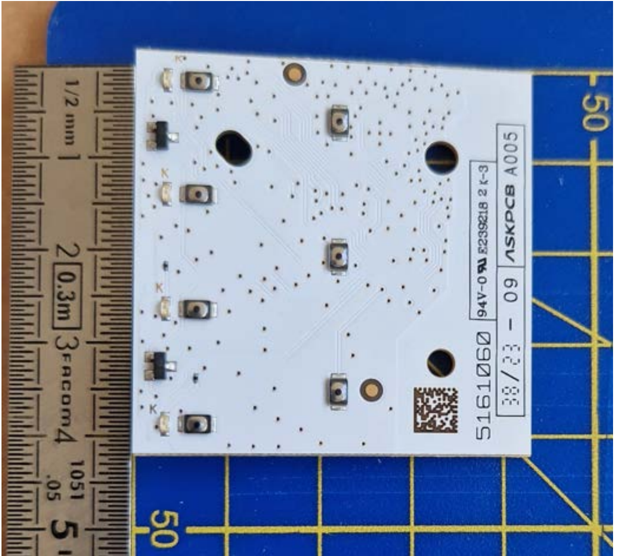
Smoove 4, PCBA, components side 2
