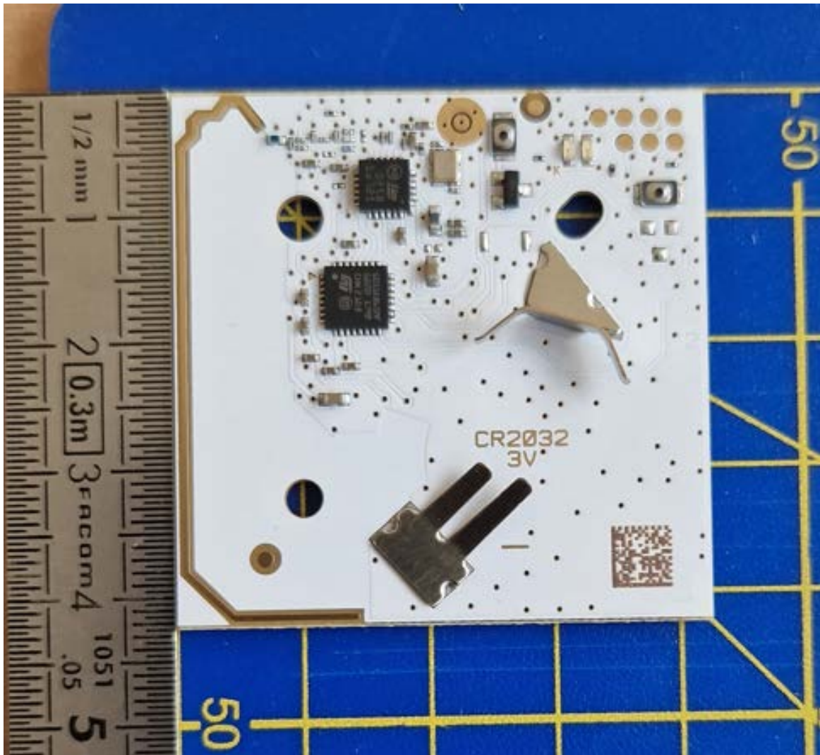
Smoove 1 RTS, PCBA, components side 1
