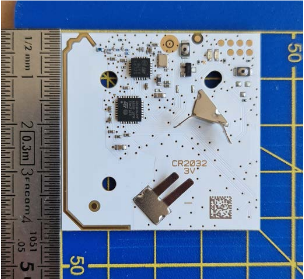
Smoove 4 , PCBA, components side 1
