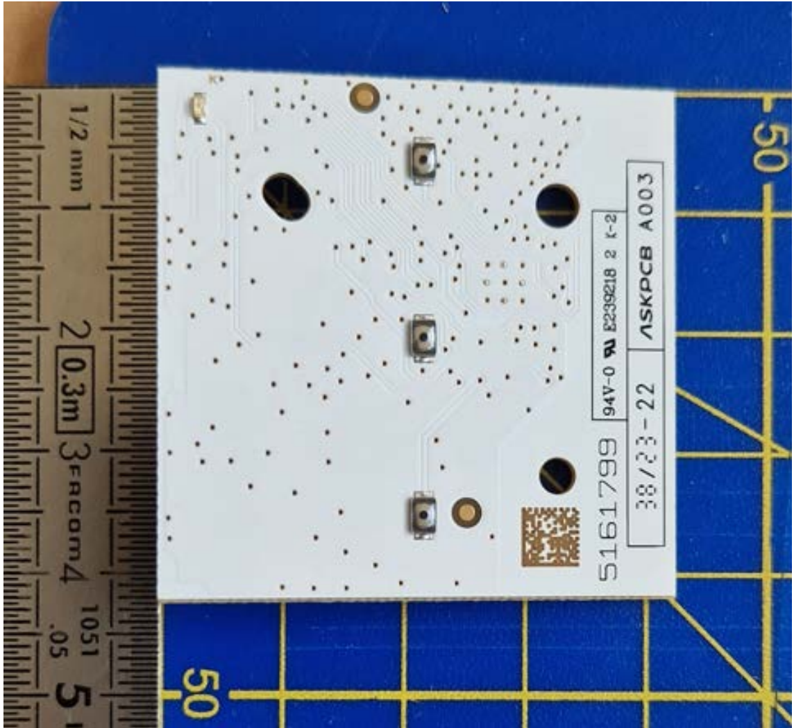
Smoove 1 RTS, PCBA, components side 2
