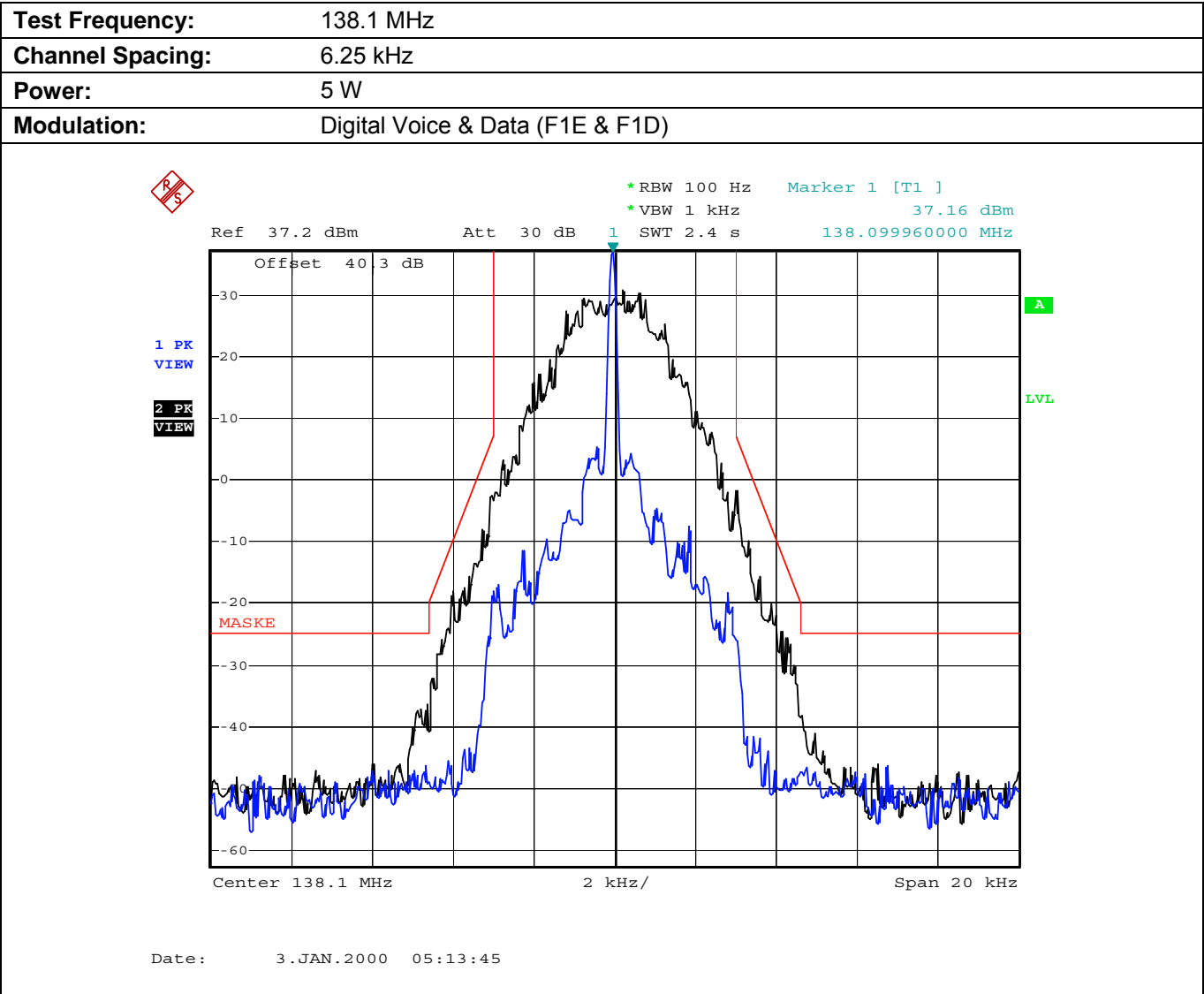
Plot 5.8.4.4. Emission Mask E, Low Power
