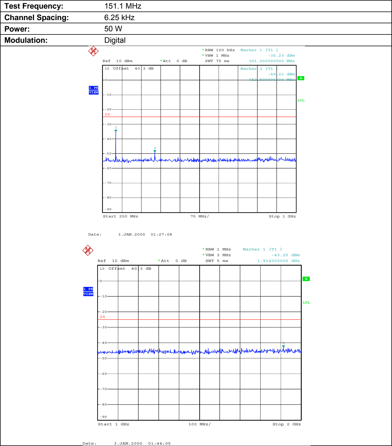
Plot 5.9.4.2.2. Conducted Transmitter Spurious Emissions for 151.1 MHz, High Power, 250 MHz - 2 GHz
