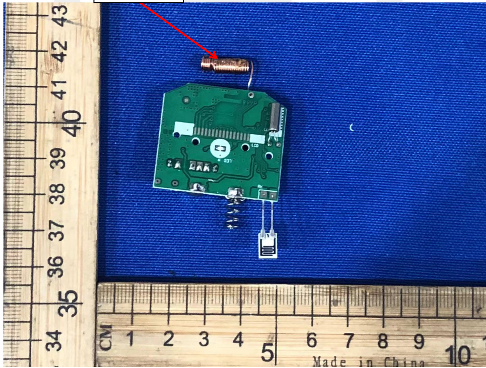
Coil ANT
