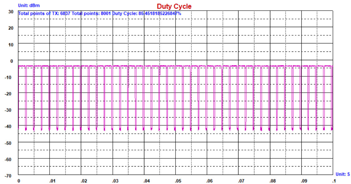
Duty Cycle_BLE_2402_Ant1
