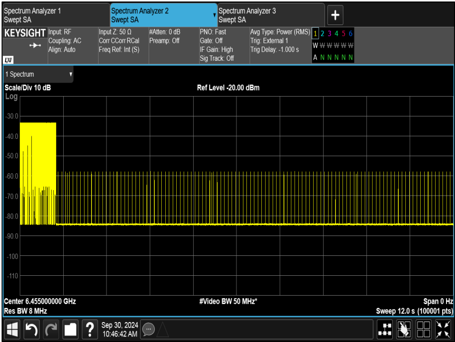
Figure 384 - U-NII-6, Maximum Bandwidth (AWGN High)
