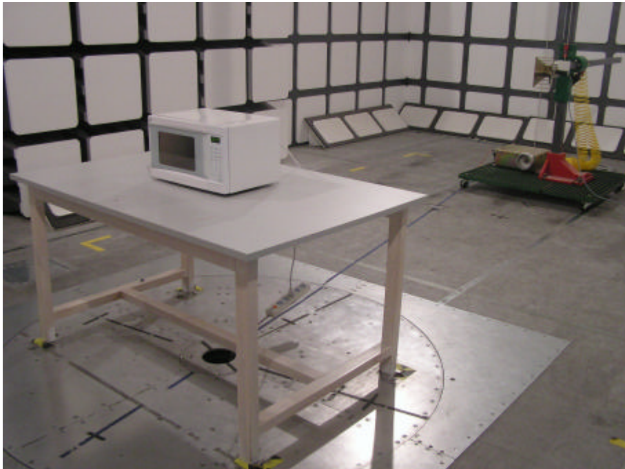
Radiated Emission – Side View (Above 1 GHz)
