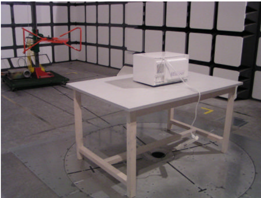
Radiated Emission – Side View (30 MHz-1000MHz)
