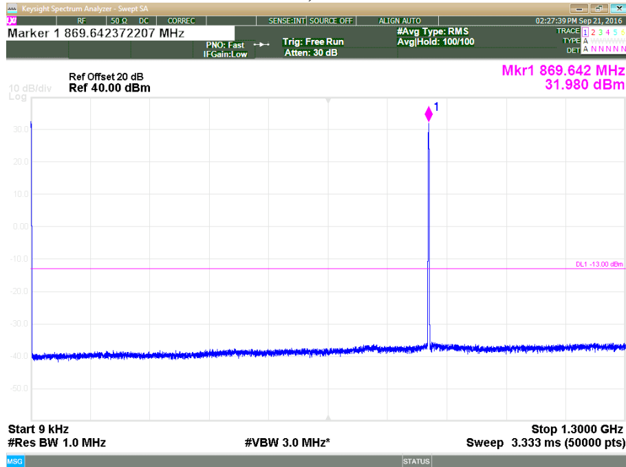
Plot 3.5.1: Spurious Emission Conducted Measurement, MSK Gaussian filter 0.3 data rate 270kbps, F_c = 869.200 MHz, 9 kHz – 1.3 GHz
