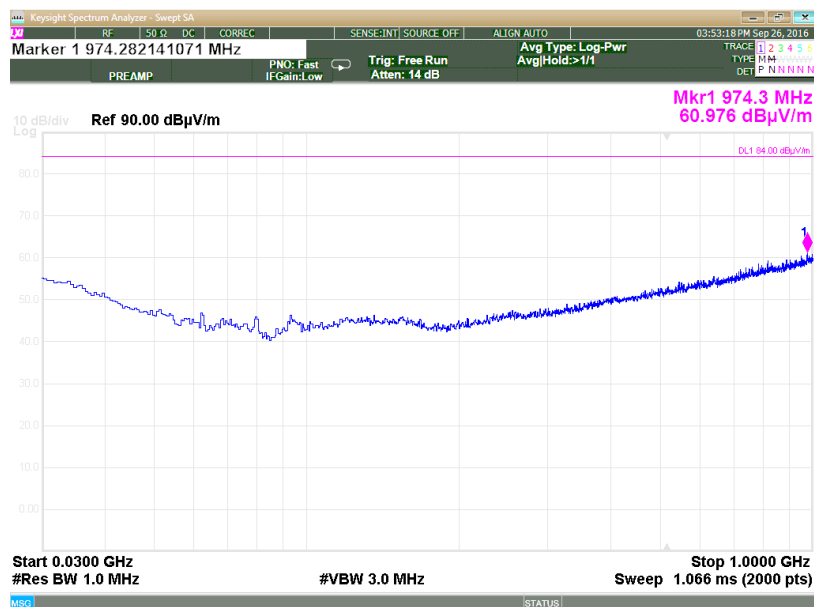
Plot 3.7.10: Spurious Emissions test results, 30 MHz – 1GHz range, Vertical polarization, High Frequency
