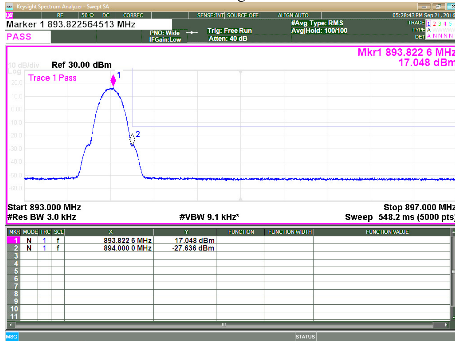
Plot 3.4.3: Band Edge test results, MSK Gaussian filter 0.3 data rate 270kbps, F_c = 893.8 MHz, single test signal
