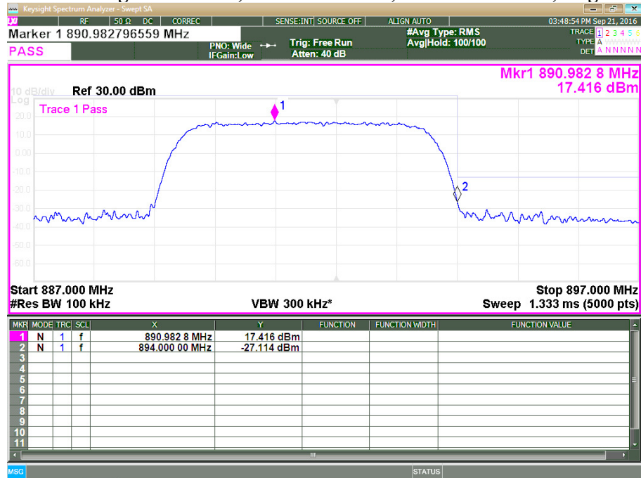
Plot 3.4.7: Band Edge test results, AWGN 4.1MHz, Fc = 891.50 MHz, single test signal
