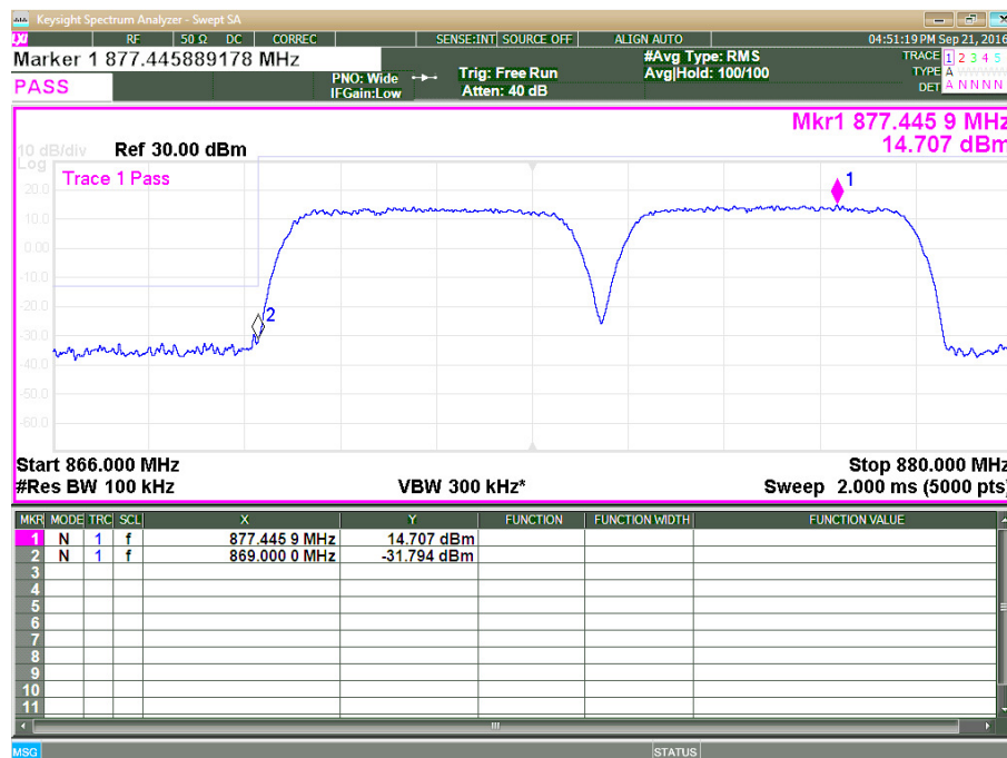
Plot 3.4.6: Band Edge test results, AWGN 4.1MHz, F_c = 871.5 + 876.5 MHz, two test signals
