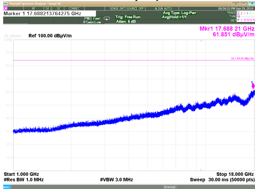
Plot 3.6.15: Spurious Emissions test results, 1 GHz – 18 GHz range, Horizontal polarization, Low Frequency
