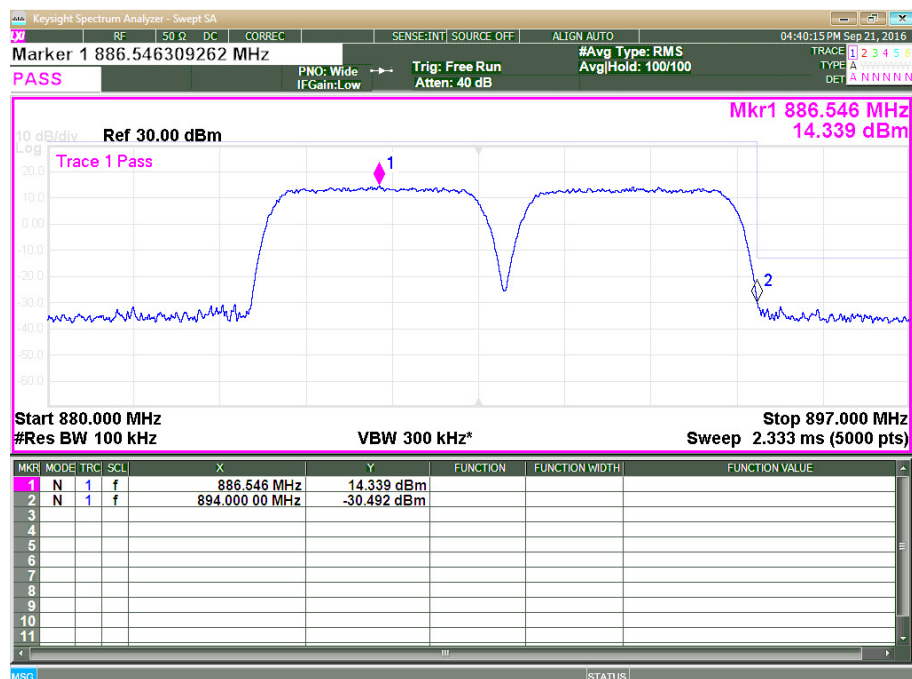
Plot 3.4.8: Band Edge test results, AWGN 4.1MHz, Fc = 891.5 + 886.5 MHz, two test signals
