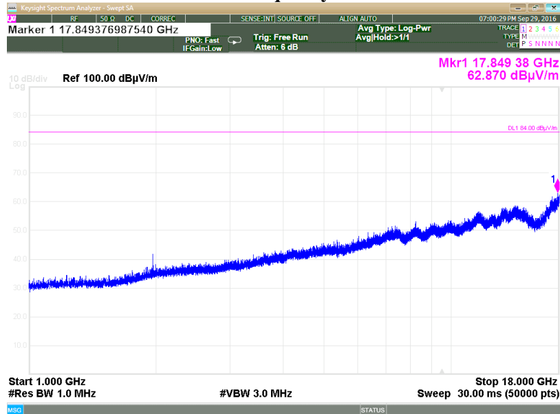
Plot 3.6.19: Spurious Emissions test results, 1 GHz – 18 GHz range, Horizontal polarization, Middle Frequency
