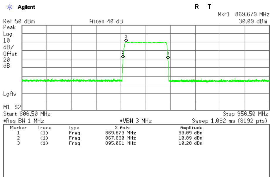
Plot 3.1: Out-of-Band rejection, CW
