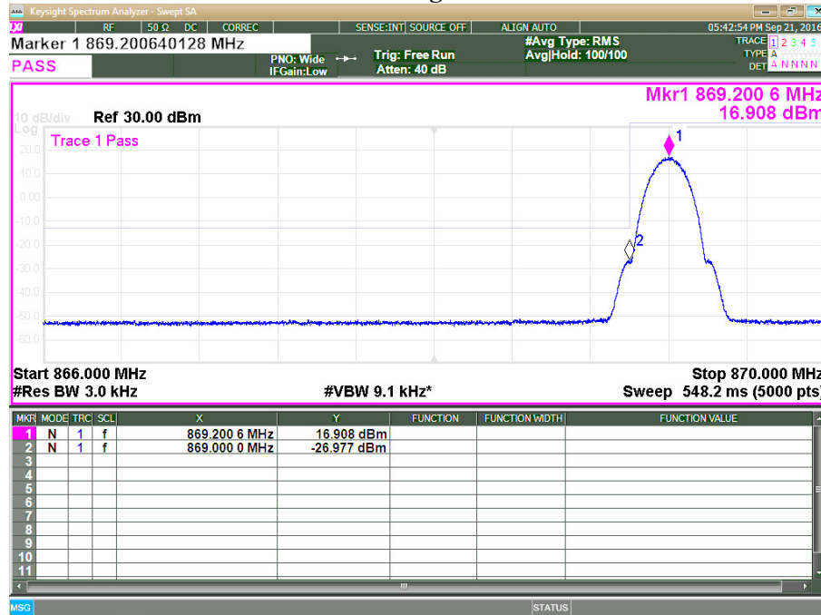
Plot 3.4.1: Band Edge test results, MSK Gaussian filter 0.3 data rate 270kbps, F_c = 869.2 MHz, single test signal
