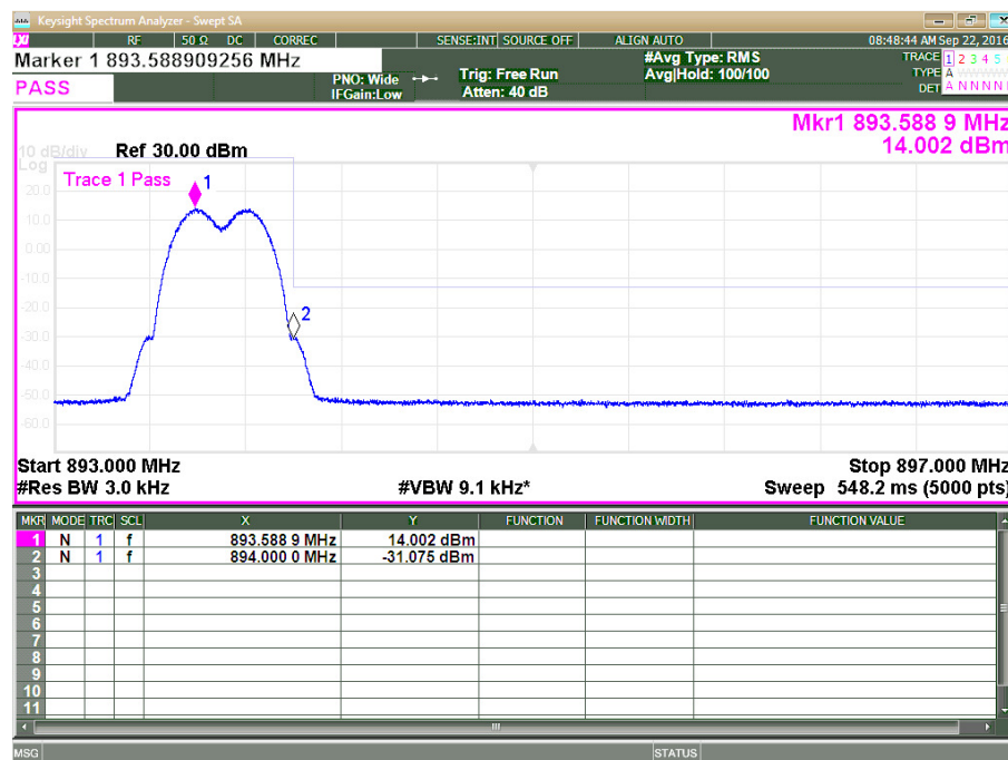
Plot 3.4.4: Band Edge test results, MSK Gaussian filter 0.3 data rate 270kbps, F_c = 893.8 + 893.6 MHz, two test signals
