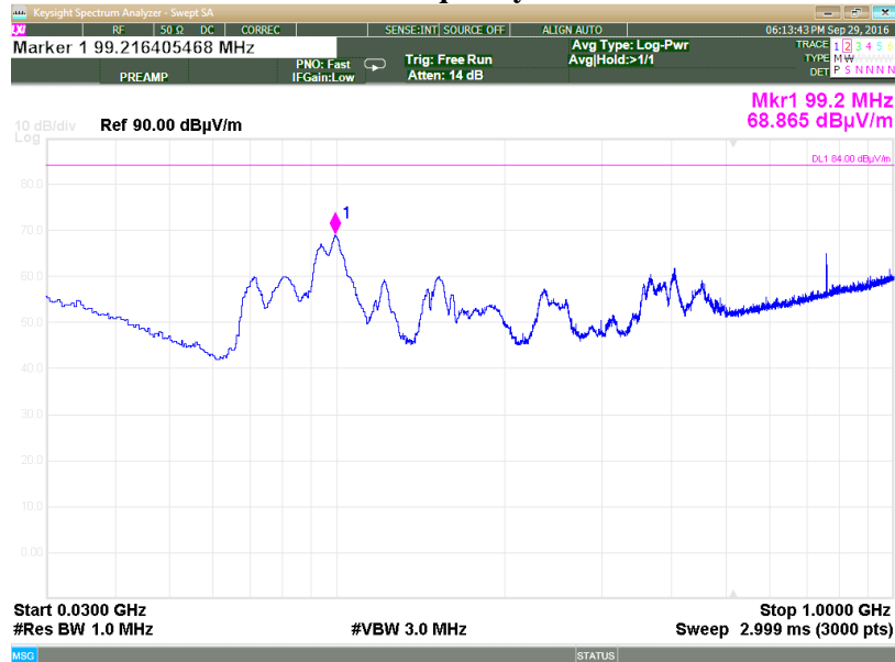
Plot 3.6.21: Spurious Emissions test results, 30 MHz – 1 GHz range, Horizontal polarization, High Frequency
