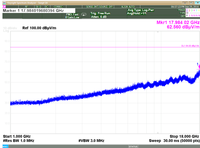
Plot 3.6.23: Spurious Emissions test results, 1 GHz – 18 GHz range, Horizontal polarization, High Frequency
