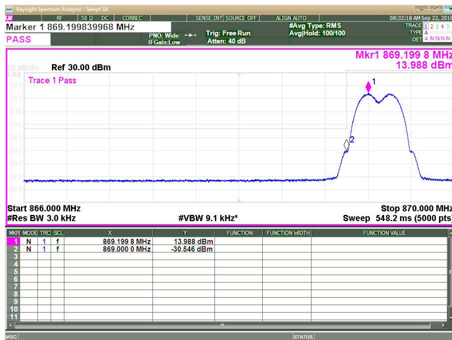
Plot 3.4.2: Band Edge test results, MSK Gaussian filter 0.3 data rate 270kbps, F_c = 869.2 + 869.4 MHz, two test signals
