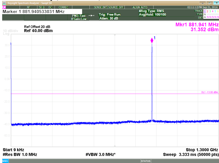
Plot 3.5.3: Spurious Emission Conducted Measurement, MSK Gaussian filter 0.3 data rate 270kbps, Fc = 881.500, 9 kHz – 1.3 GHz
