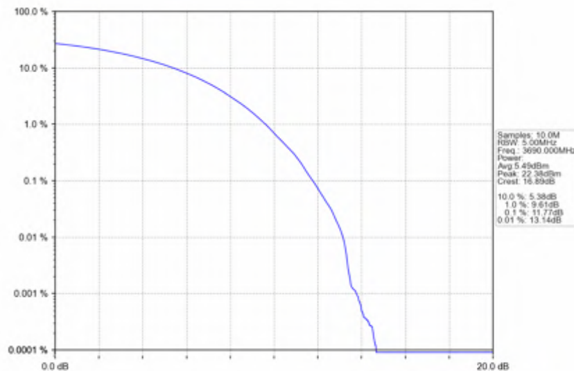
n78d_15kHz_SISO_NTNV_20MHz_CP-OFDM QPSK_3690MHz_Outer_Full
