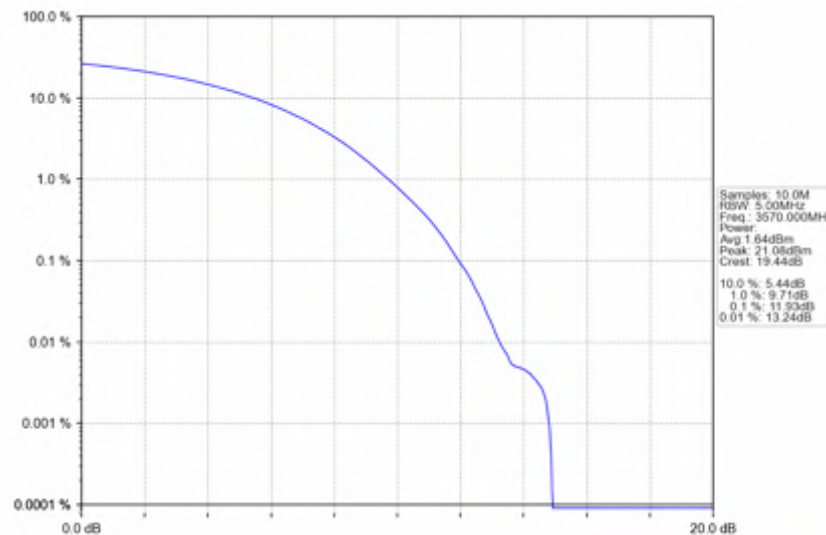
n78d_30kHz_SISO_NTNV_40MHz_CP-OFDM_16_QAM_3570MHz_Outer_Full
