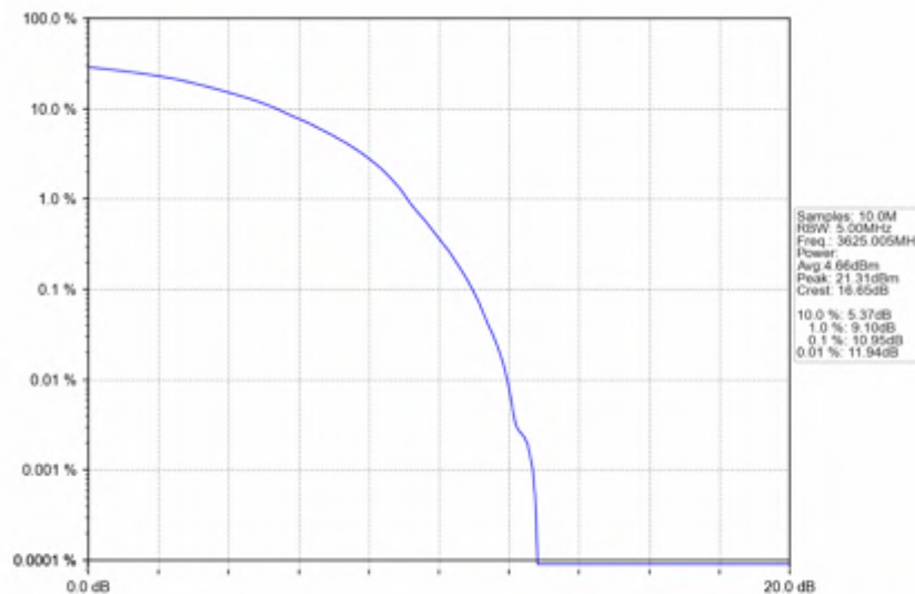
n78d_15kHz_SISO_NTNV_25MHz_DFT-s-OFDM_16_QAM_3625.005MHz_Outer_Full
