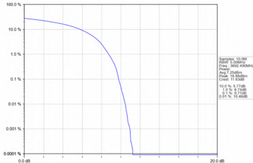
n78d_30kHz_SISO_NTNV_15MHz_DFT-s-OFDM_QPSK_3692.49MHz_Outer_Full
