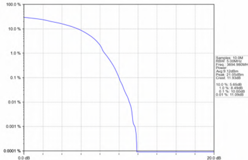
n78d_30kHz_SISO_NTV_10MHz_DFT-s-OFDM_64_QAM_3694.98MHz_Outer_Full
