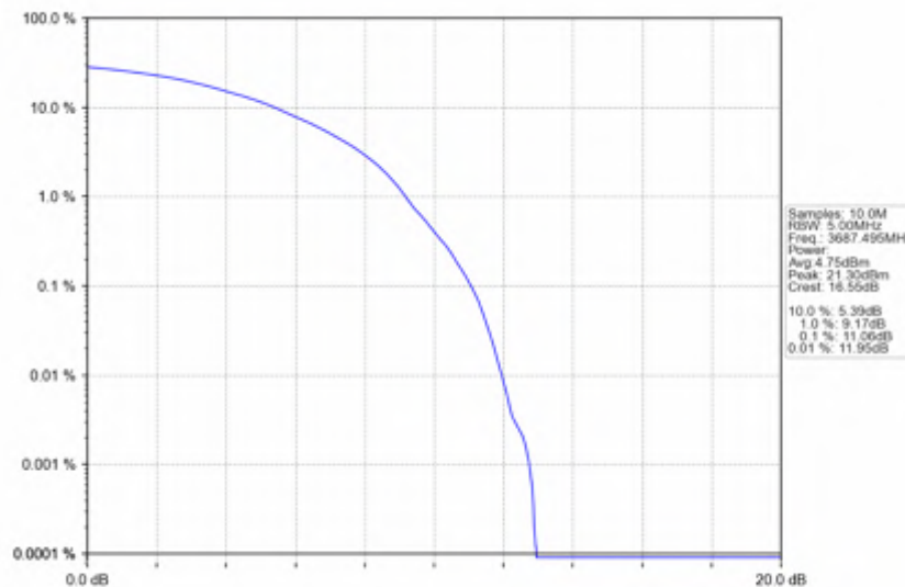
n78d_15kHz_SISO_NTNV_25MHz_DFT-s-OFDM 16 QAM_3687.495MHz_Outer_Full
