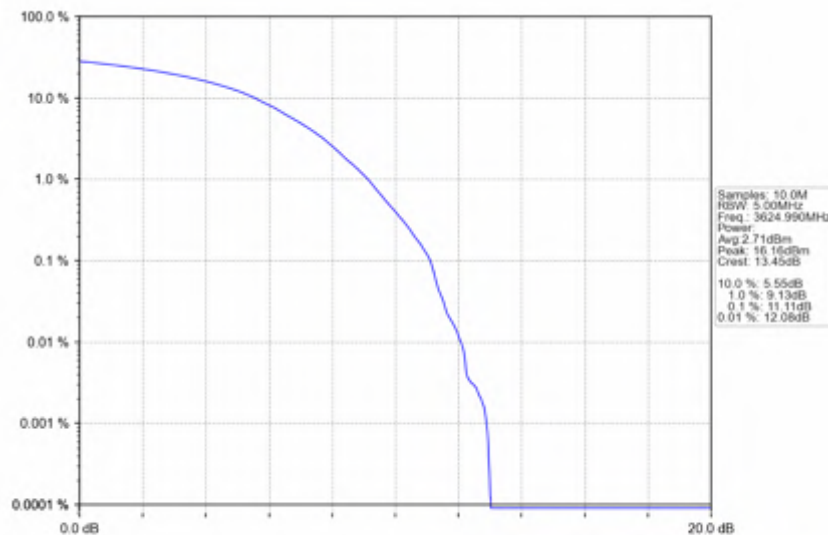
n78d_30kHz_SISO_NTNV_40MHz_DFT-s-OFDM_QPSK_3624.99MHz_Outer_Full
