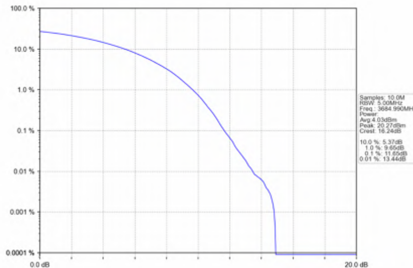
n78d_30kHz_SISO_NTNV_30MHz_CP-OFDM 64 QAM_3684.99MHz_Outer_Full
