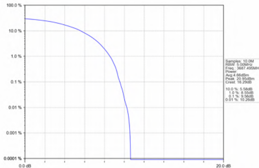
n78d_15kHz_SISO_NTNV_25MHz_DFT-s-OFDM PI/2 BPSK_3687.495MHz_Outer_Full
