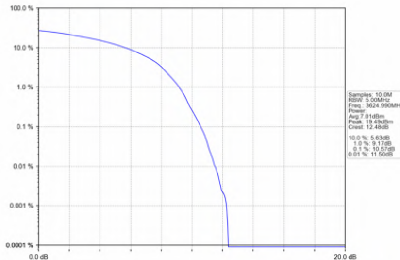
n78d_30kHz_SISO_NTNV_15MHz_DFT-s-OFDM_256_QAM_3624.99MHz_Outer_Full
