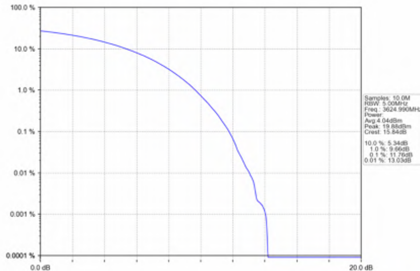
n78d_30kHz_SISO_NTNV_30MHz_CP-OFDM_256_QAM_3624.99MHz_Outer_Full
