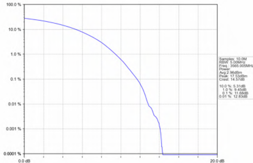
n78d_15kHz_SISO_NTNV_30MHz_CP-OFDM_16_QAM_3565.005MHz_Outer_Full
