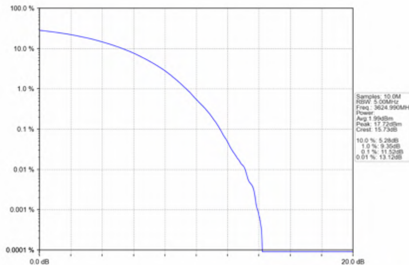
n78d_30kHz_SISO_NTNV_50MHz_CP-OFDM 64 QAM_3624.99MHz_Outer_Full
