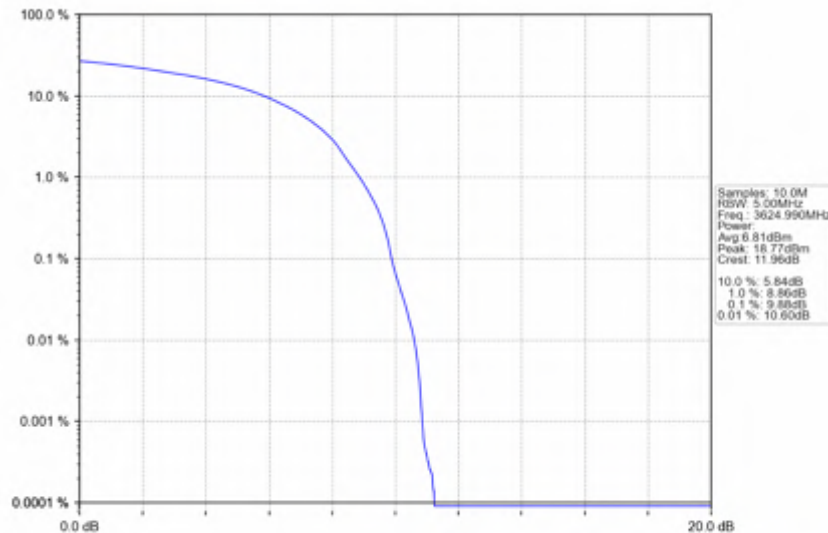
n78d_30kHz_SISO_NTNV_15MHz_DFT-s-OFDM_QPSK_3624.99MHz_Outer_Full
