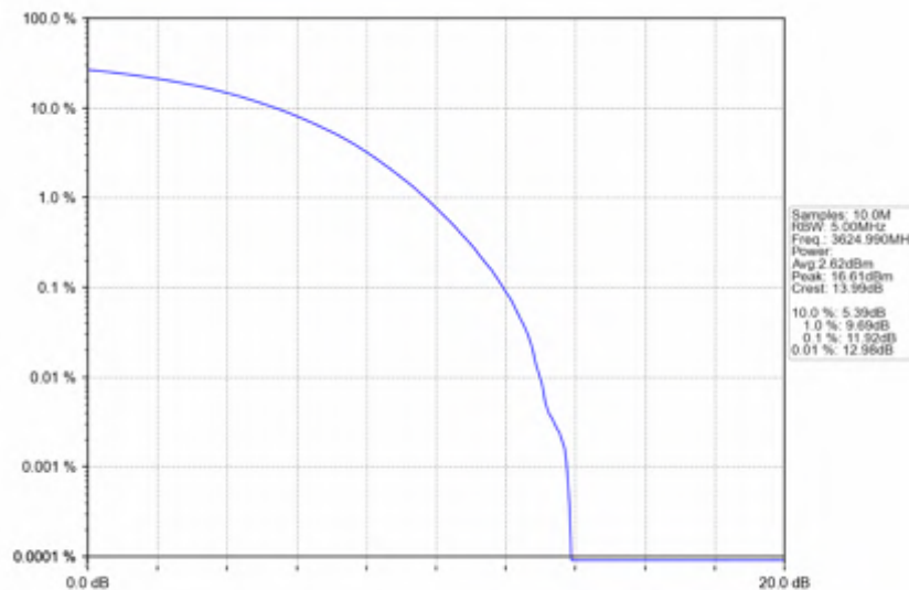
n78d_30kHz_SISO_NTNV_40MHz_CP-OFDM 64 QAM_3624.99MHz_Outer_Full
