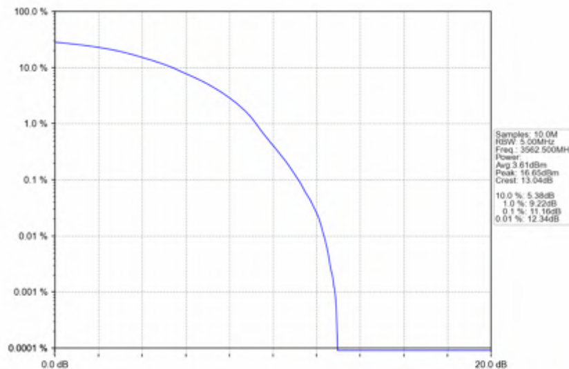
n78d_15kHz_SISO_NTNV_25MHz_DFT-s-OFDM 64 QAM_3562.5MHz_Outer_Full
