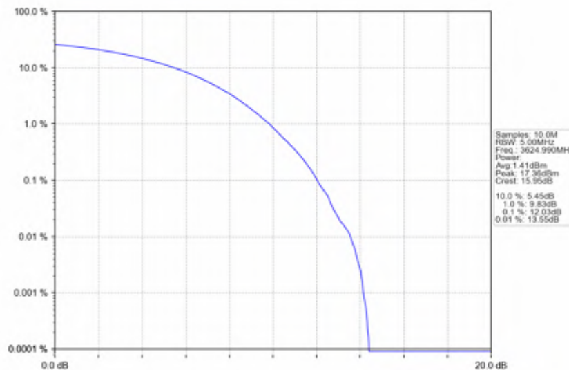
n78d_30kHz_SISO_NTNV_50MHz_CP-OFDM QPSK_3624.99MHz_Outer_Full
