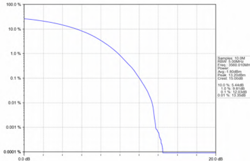
n78d_15kHz_SISO_NTNV_20MHz_CP-OFDM_QPSK_3560.01MHz_Outer_Full
