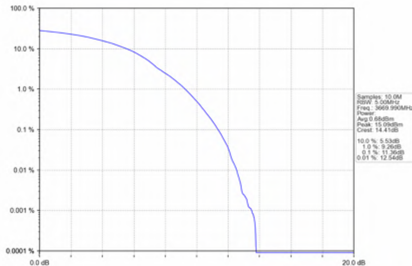
n78d_30kHz_SISO_NTNV_60MHz_DFT-s-OFDM_QPSK_3669.99MHz_Outer_Full
