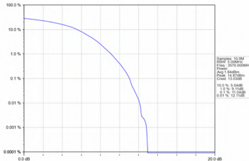
n78d_30kHz_SISO_NTNV_40MHz_DFT-s-OFDM_QPSK_3570MHz_Outer_Full
