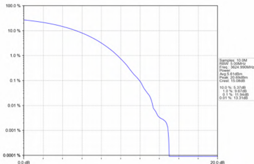
n78d 30kHz SISO NTNV 20MHz CP-OFDM 256 QAM 3624.99MHz Outer Full
