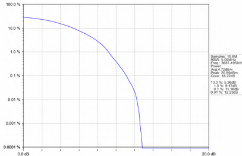
n78d_15kHz_SISO_NTNV_25MHz_DFT-s-OFDM_64_QAM_3687.495MHz_Outer_Full
