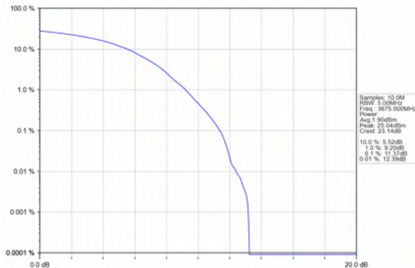
n78d_30kHz_SISO_NTV_50MHz_DFT-s-OFDM 64 QAM_3675MHz_Outer_Full
