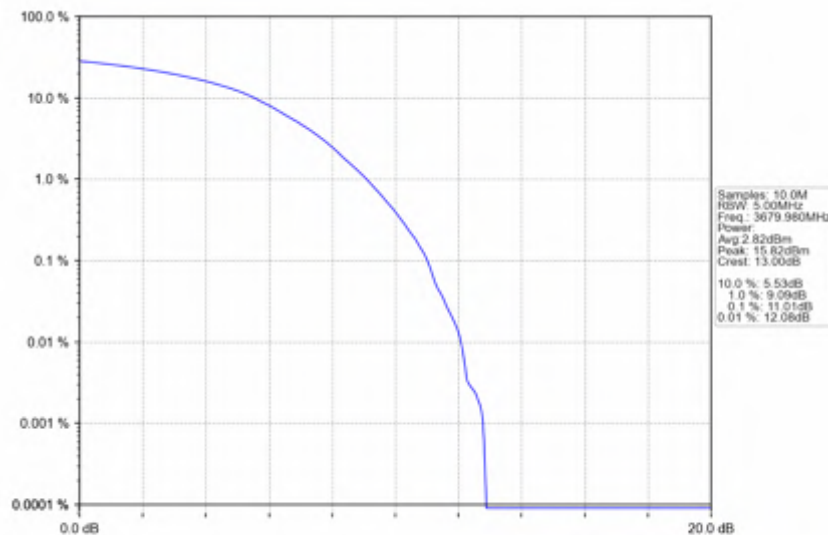
n78d_30kHz_SISO_NTNV_40MHz_DFT-s-OFDM_QPSK_3679.98MHz_Outer_Full
