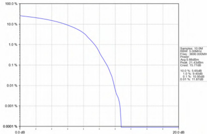
n78d_15kHz_SISO_NTNV_20MHz_DFT-s-OFDM_256_QAM_3690MHz_Outer_Full
