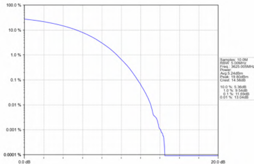
n78d_15kHz_SISO_NTNV_20MHz_CP-OFDM QPSK_3625.005MHz_Outer_Full
