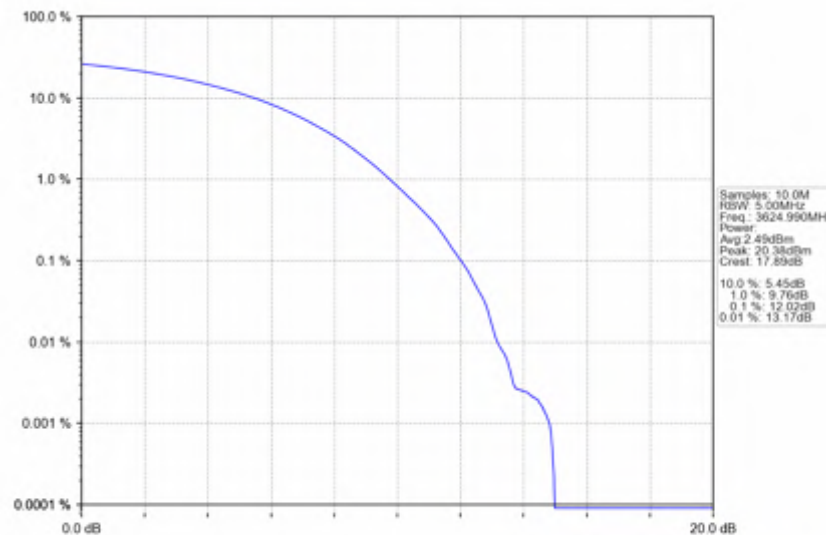
n78d_30kHz_SISO_NTNV_40MHz_CP-OFDM_16_QAM_3624.99MHz_Outer_Full
