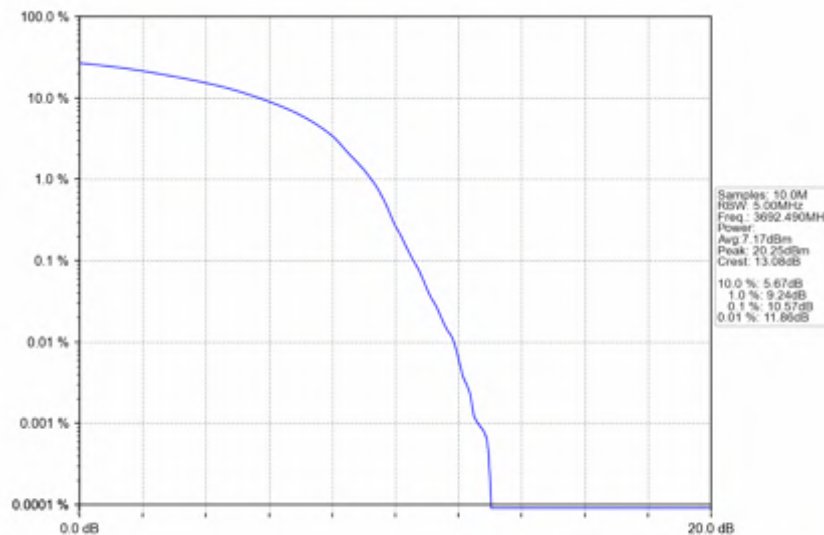
n78d_30kHz_SISO_NTV_15MHz_DFT-s-OFDM_16_QAM_3692.49MHz_Outer_Full
