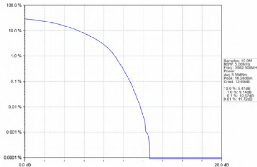
n78d_15kHz_SISO_NTNV_25MHz_DFT-s-OFDM QPSK_3562.5MHz_Outer_Full
