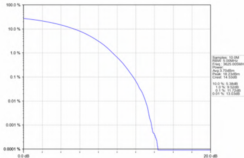
n78d_15kHz_SISO_NTNV_30MHz_CP-OFDM 64 QAM_3625.005MHz_Outer_Full
