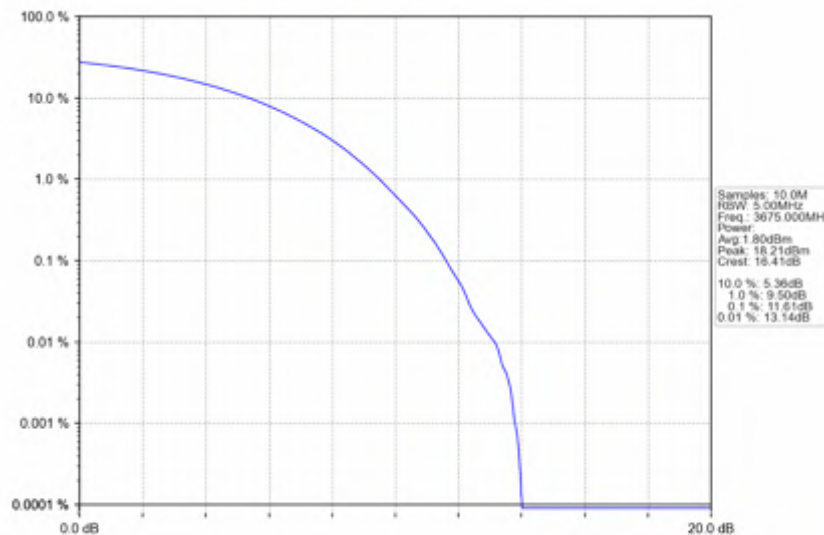
n78d_30kHz_SISO_NTNV_50MHz_CP-OFDM QPSK_3675MHz_Outer_Full
