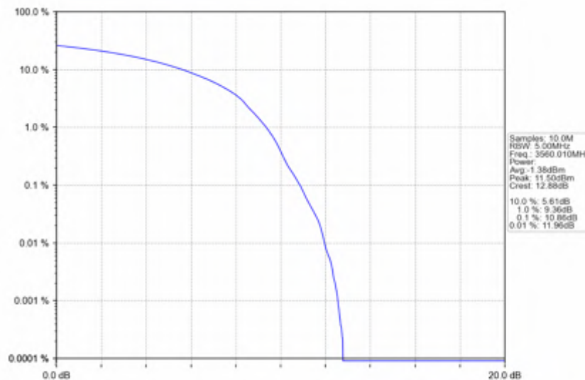
n78d_15kHz_SISO_NTNV_20MHz_DFT-s-OFDM 64 QAM_3560.01MHz_Outer_Full
