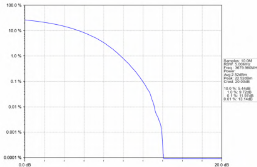
n78d_30kHz_SISO_NTNV_40MHz_CP-OFDM 64 QAM_3679.98MHz_Outer_Full
