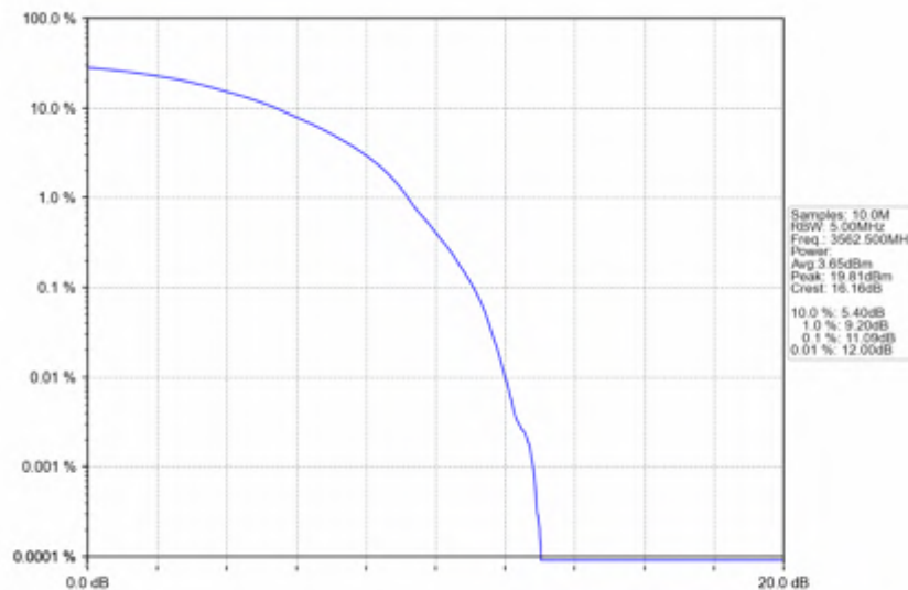
n78d_15kHz_SISO_NTNV_25MHz_DFT-s-OFDM_16_QAM_3562.5MHz_Outer_Full
