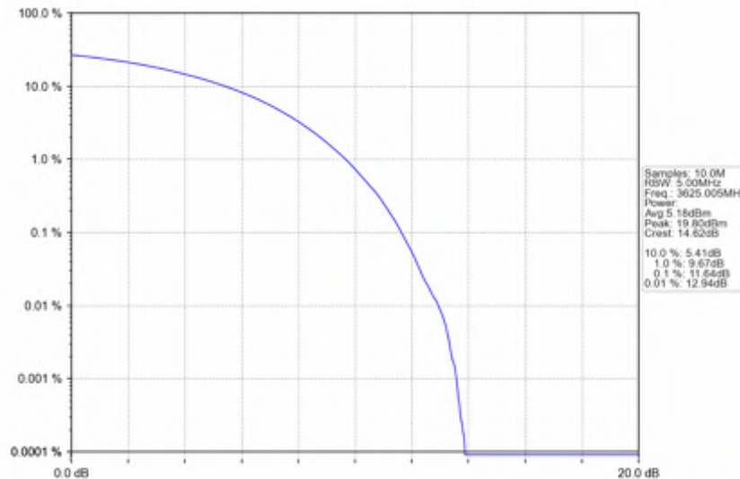
n78d_15kHz_SISO_NTNV_20MHz_CP-OFDM_256_QAM_3625.005MHz_Outer_Full
