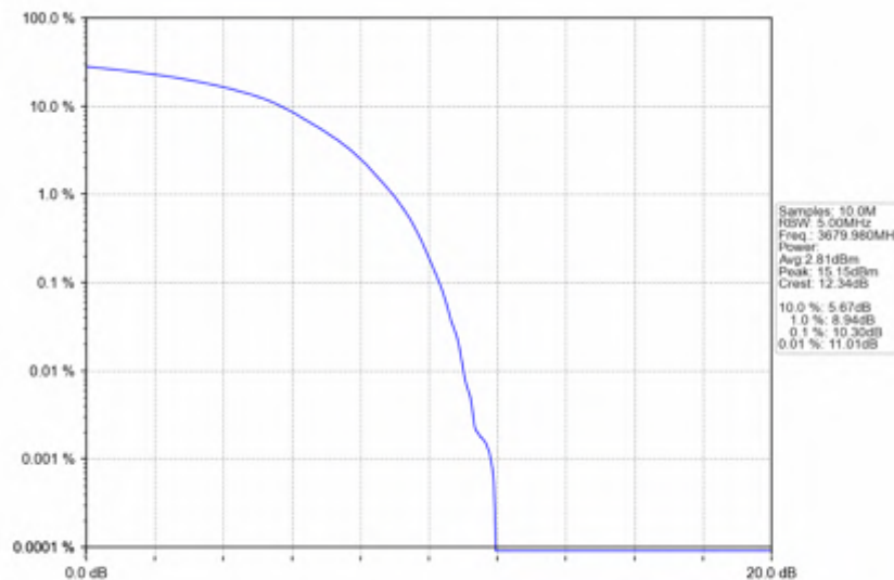
n78d_30kHz_SISO_NTNV_40MHz_DFT-s-OFDM_PI/2_BPSK_3679.98MHz_Outer_Full
