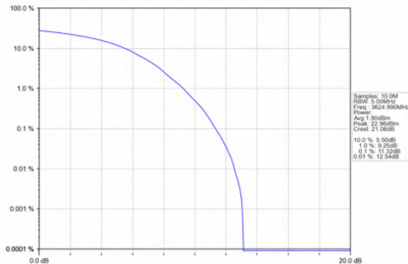
n78d_30kHz_SISO_NTV_50MHz_DFT-s-OFDM 64 QAM_3624.99MHz_Outer_Full
