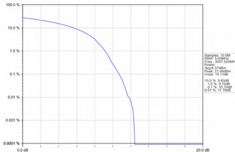
n78d_30kHz_SISO_NTNV_15MHz_DFT-s-OFDM_256_QAM_3557.52MHz_Outer_Full
