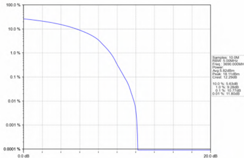
n78d_15kHz_SISO_NTNV_20MHz_DFT-s-OFDM 16 QAM_3690MHz_Outer_Full
