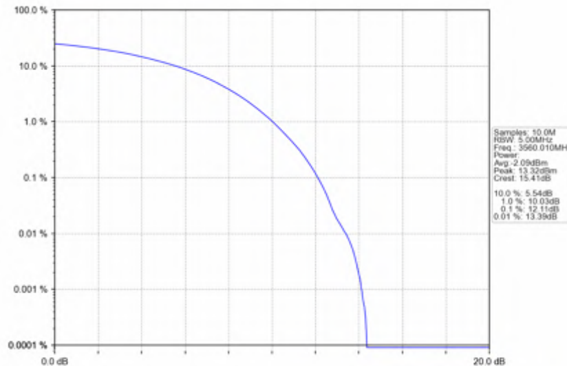
n78d_15kHz_SISO_NTNV_20MHz_CP-OFDM_256_QAM_3560.01MHz_Outer_Full
