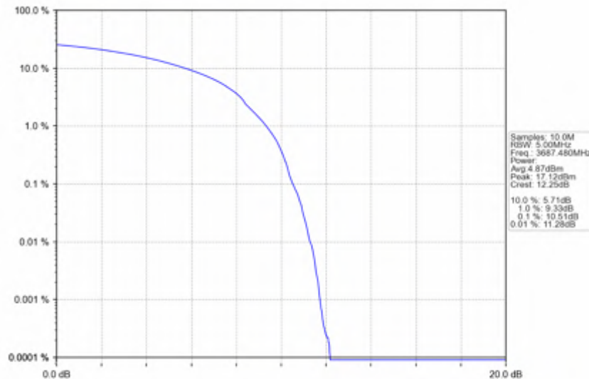
n78d_30kHz_SISO_NTNV_25MHz_DFT-s-OFDM_QPSK_3687.48MHz_Outer_Full
