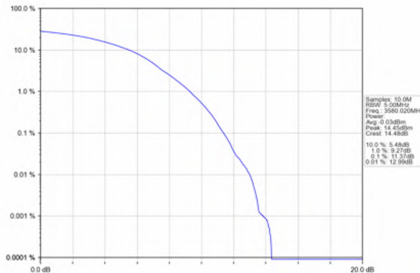
n78d_30kHz_SISO_NTNV_60MHz_DFT-s-OFDM_256_QAM_3580.02MHz_Outer_Full
