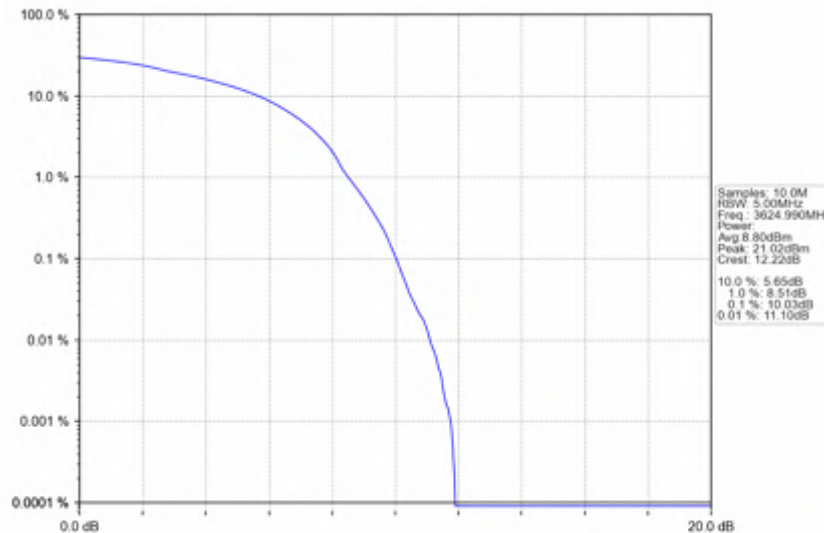
n78d_30kHz_SISO_NTV_10MHz_DFT-s-OFDM_64_QAM_3624.99MHz_Outer_Full
