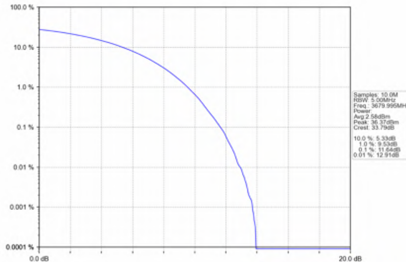
n78d_15kHz_SISO_NTNV_40MHz_CP-OFDM 64 QAM_3679.995MHz_Outer_Full
