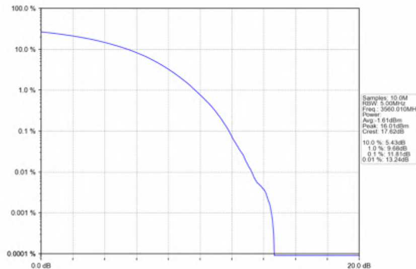
n78d_15kHz_SISO_NTNV_20MHz_CP-OFDM 64 QAM_3560.01MHz_Outer_Full
