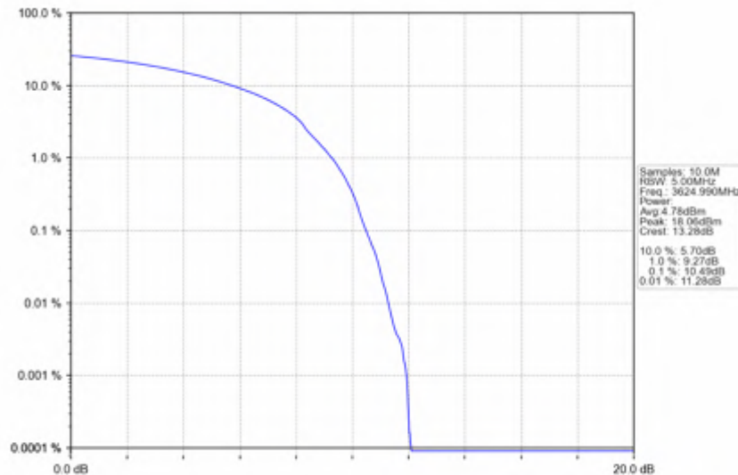
n78d_30kHz_SISO_NTNV_25MHz_DFT-s-OFDM_QPSK_3624.99MHz_Outer_Full
