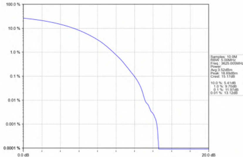
n78d_15kHz_SISO_NTNV_30MHz_CP-OFDM_16_QAM_3625.005MHz_Outer_Full
