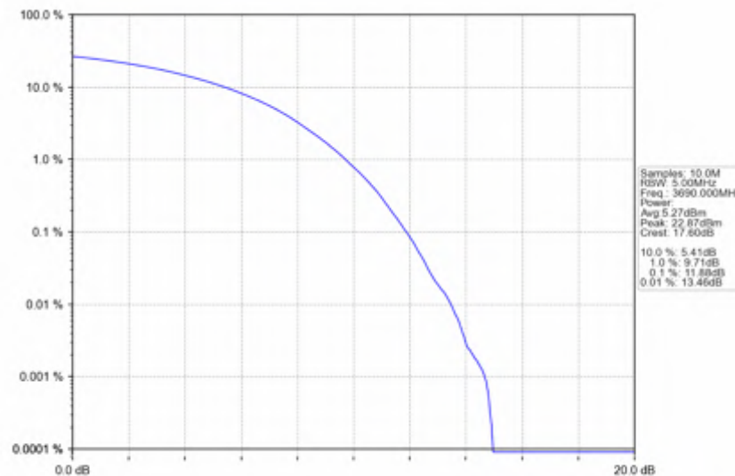
n78d_15kHz_SISO_NTNV_20MHz_CP-OFDM 16 QAM_3690MHz_Outer_Full
