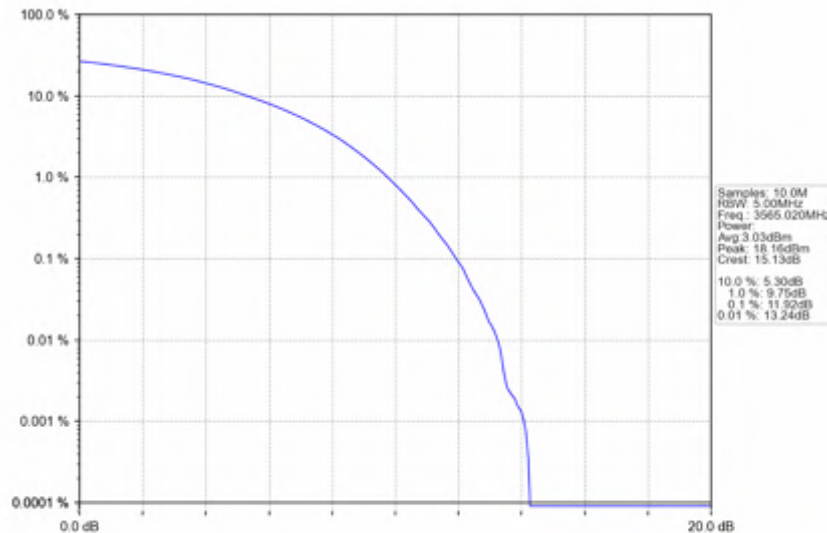
n78d_30kHz_SISO_NTNV_30MHz_CP-OFDM_256_QAM_3565.02MHz_Outer_Full
