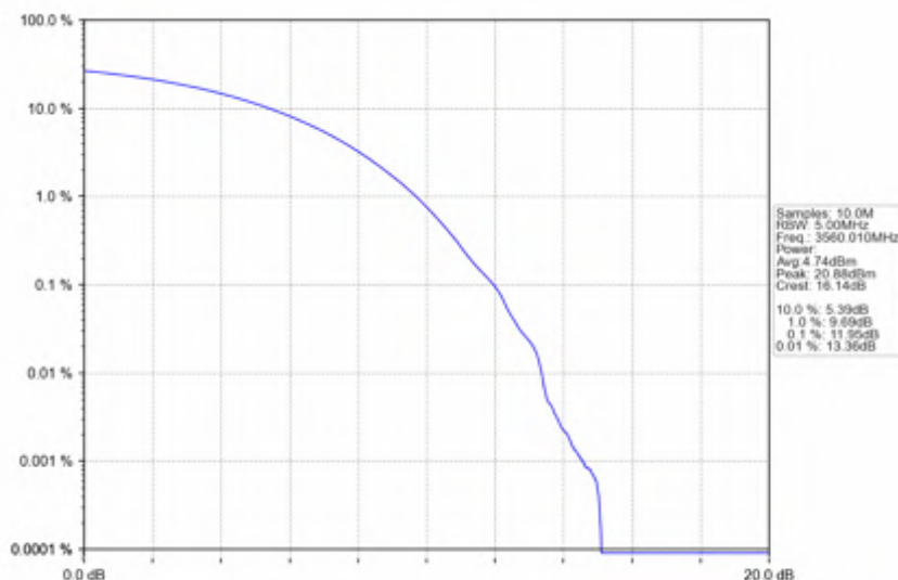
n78d 30kHz SISO NTNV 20MHz CP-OFDM 256 QAM 3560.01MHz Outer Full
