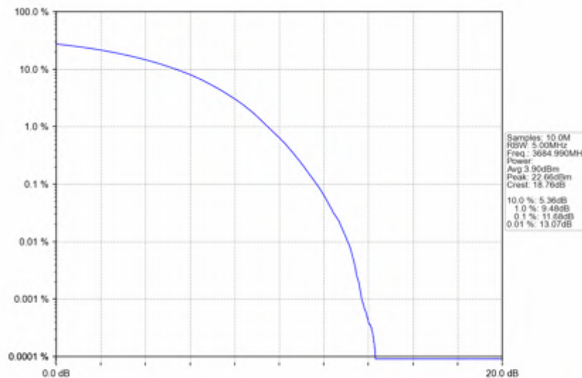
n78d_15kHz_SISO_NTNV_30MHz_CP-OFDM 64 QAM_3684.99MHz_Outer_Full
