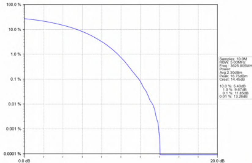
n78d_15kHz_SISO_NTNV_40MHz_CP-OFDM 64 QAM_3625.005MHz_Outer_Full
