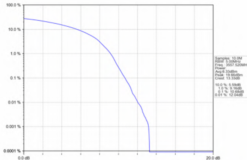
n78d_30kHz_SISO_NTV_15MHz_DFT-s-OFDM_64_QAM_3557.52MHz_Outer_Full
