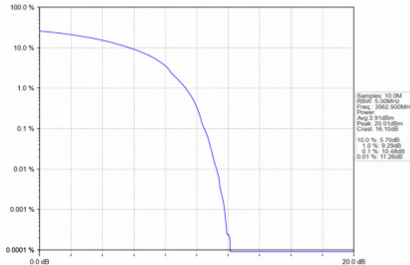
n78d_30kHz_SISO_NTNV_25MHz_DFT-s-OFDM QPSK_3562.5MHz_Outer_Full
