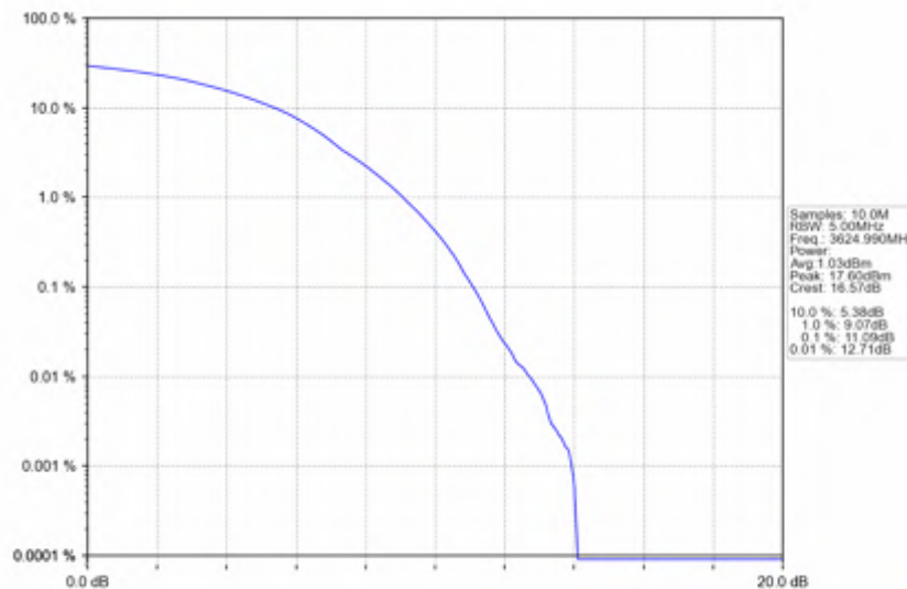
n78d_30kHz_SISO_NTNV_60MHz_DFT-s-OFDM_256_QAM_3624.99MHz_Outer_Full
