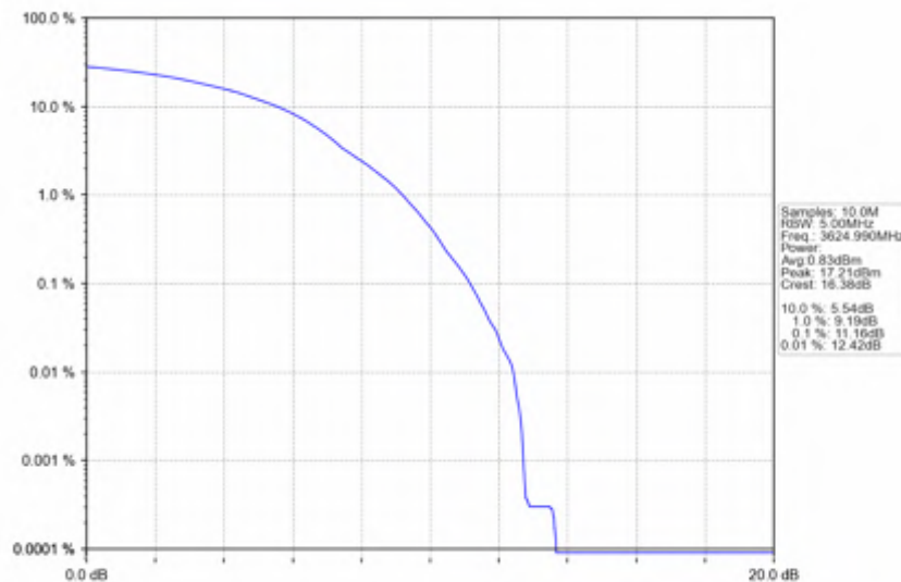
n78d_30kHz_SISO_NTNV_60MHz_DFT-s-OFDM_QPSK_3624.99MHz_Outer_Full
