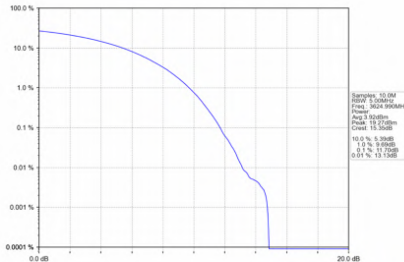
n78d_30kHz_SISO_NTNV_30MHz_CP-OFDM 64 QAM_3624.99MHz_Outer_Full
