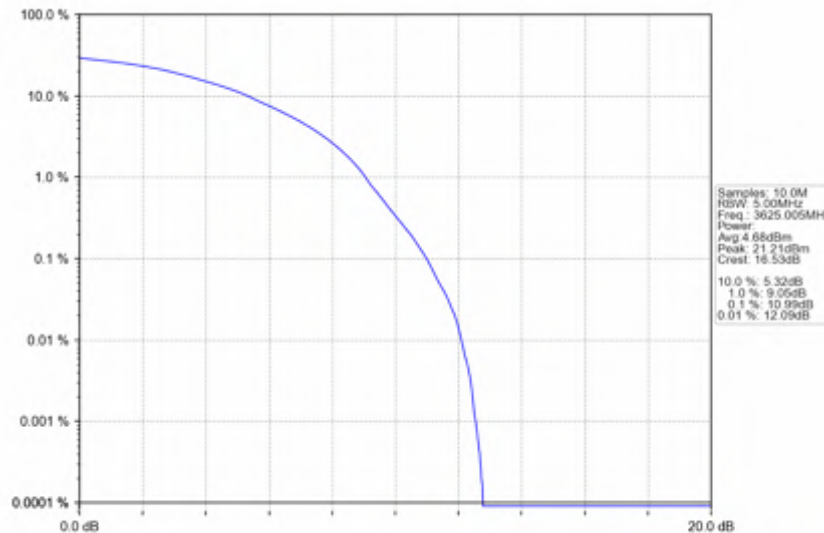
n78d_15kHz_SISO_NTNV_25MHz_DFT-s-OFDM_64_QAM_3625.005MHz_Outer_Full
