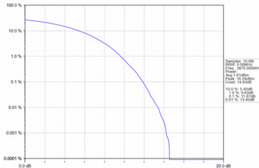
n78d_30kHz_SISO_NTNV_50MHz_CP-OFDM 64 QAM_3675MHz_Outer_Full
