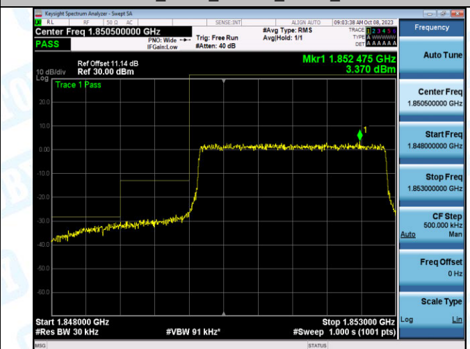
Band2_3MHz_16QAM_18615_15RB#0
