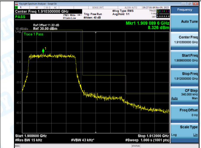
Band2_1.4MHz_QPSK_19193_6RB#0
