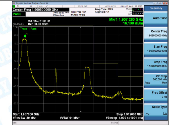
Band2_3MHz_16QAM_19185_1RB#0
