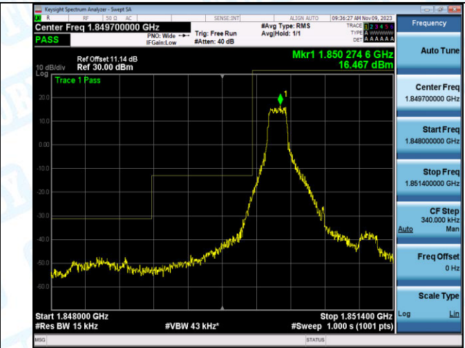
Band2_1.4MHz_QPSK_18607_1RB#0
