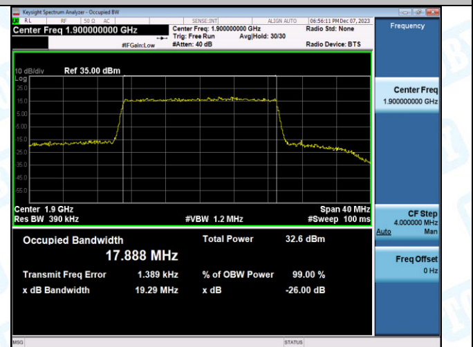
Band2-15MHz-16QAM-18900-27RB#0-PASS
