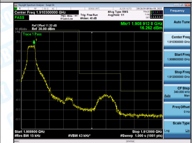
Band2_1.4MHz_QPSK_19193_1RB#0
