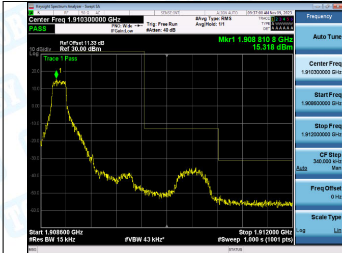
Band2_1.4MHz_16QAM_19193_1RB#0
