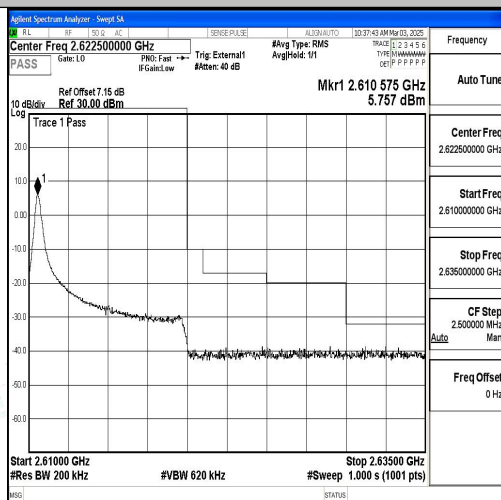
Band38_10MHz_QPSK_38200_1RB#0
