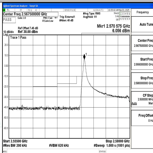
Band38_10MHz_QPSK_37800_1RB#0
