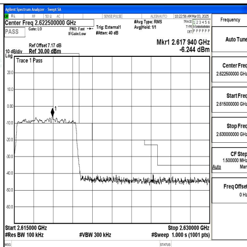
Band38_5MHz_16QAM_38225_25RB#0
