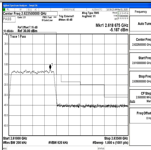
Band38_10MHz_QPSK_38200_50RB#0
