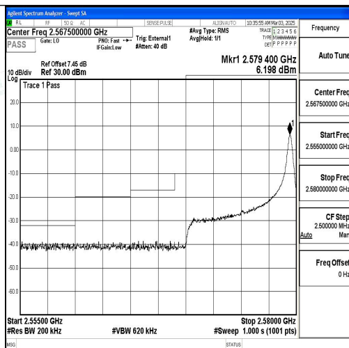
Band38_10MHz_QPSK_37800_1RB#49
