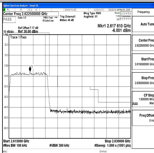
Band38_5MHz_QPSK_38225_25RB#0
