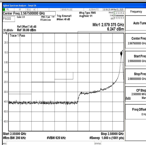
Band38_10MHz_16QAM_37800_1RB#49
