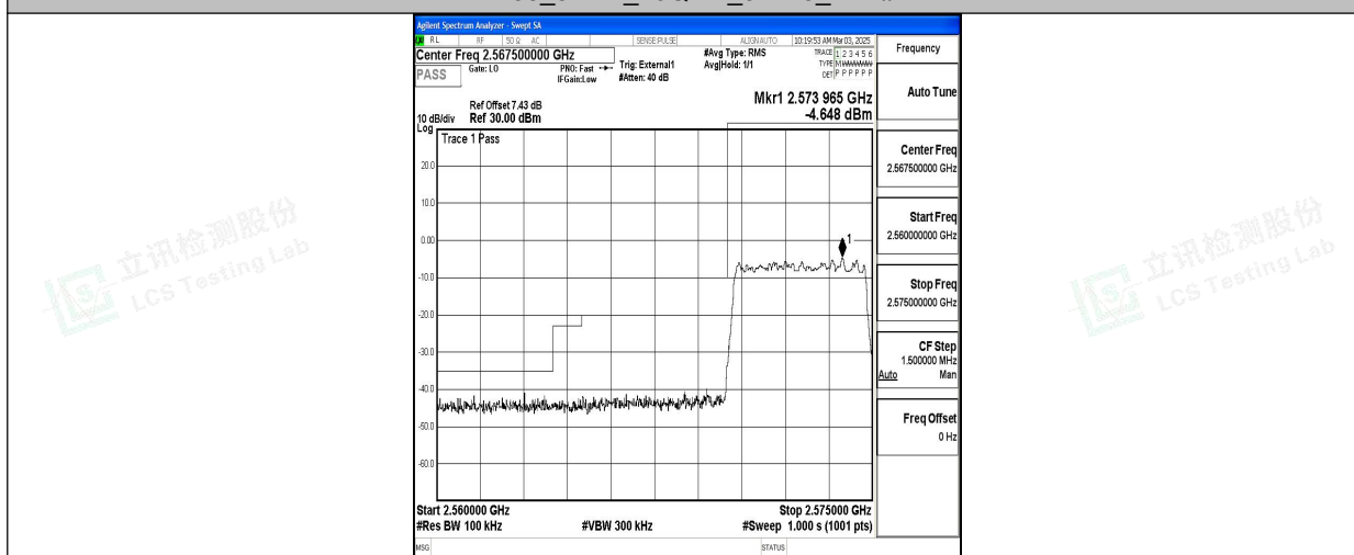
Band38_5MHz_QPSK_37775_25RB#0
