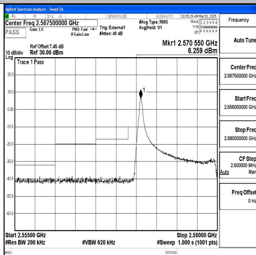
Band38_10MHz_16QAM_37800_1RB#0
