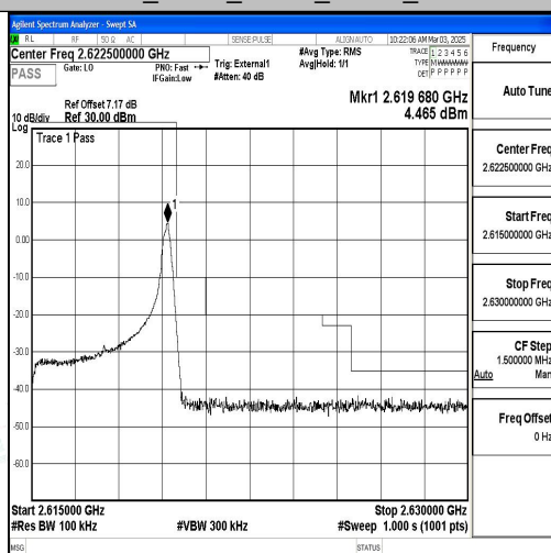
Band38_5MHz_16QAM_38225_1RB#24
