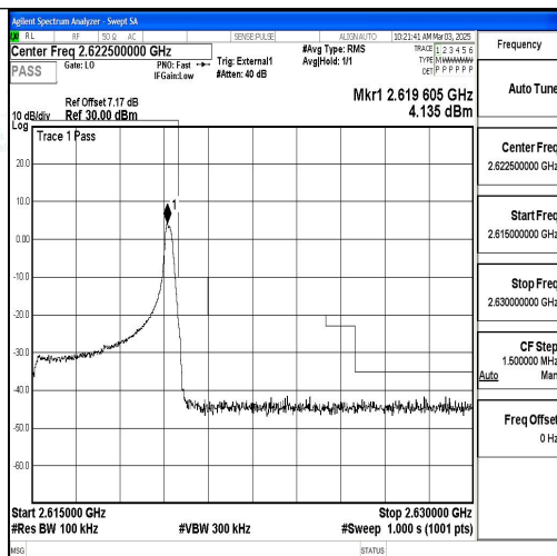
Band38_5MHz_QPSK_38225_1RB#24
