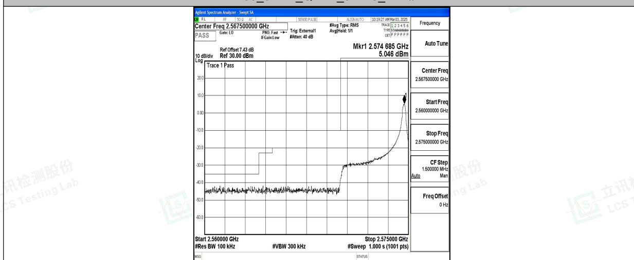
Band38_5MHz_16QAM_37775_1RB#24
