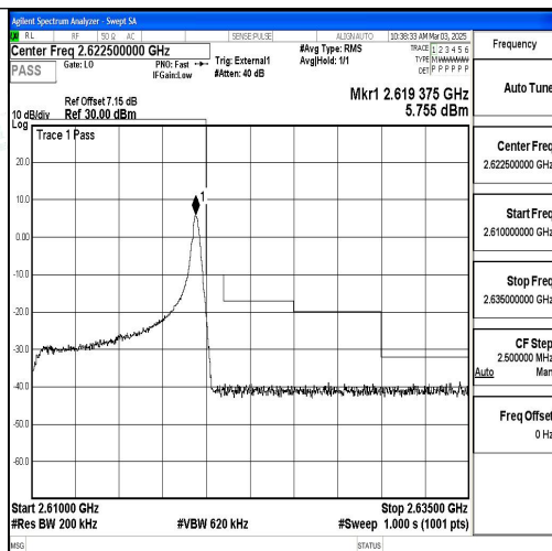
Band38_10MHz_QPSK_38200_1RB#49
