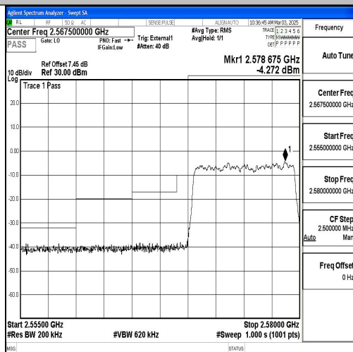
Band38_10MHz_QPSK_37800_50RB#0
