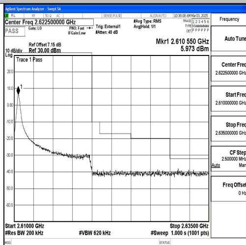
Band38_10MHz_16QAM_38200_1RB#0
