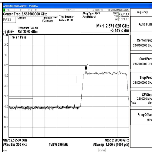
Band38_10MHz_16QAM_37800_50RB#0
