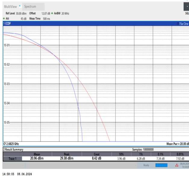
Band41-15MHz-QPSK-41515-75RB#0-PASS
