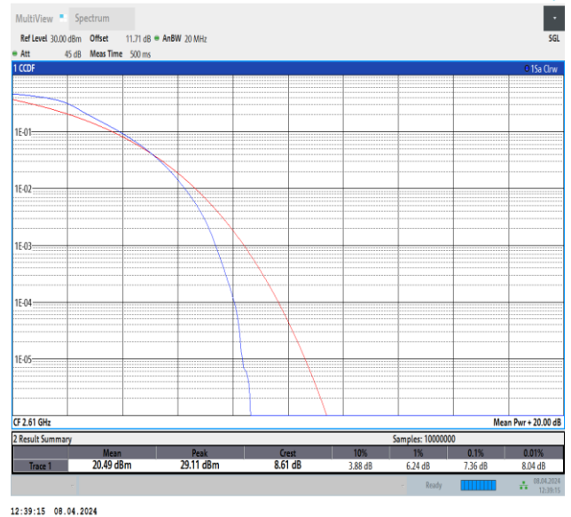
Band38-20MHz-QPSK-38150-100RB#0-PASS
