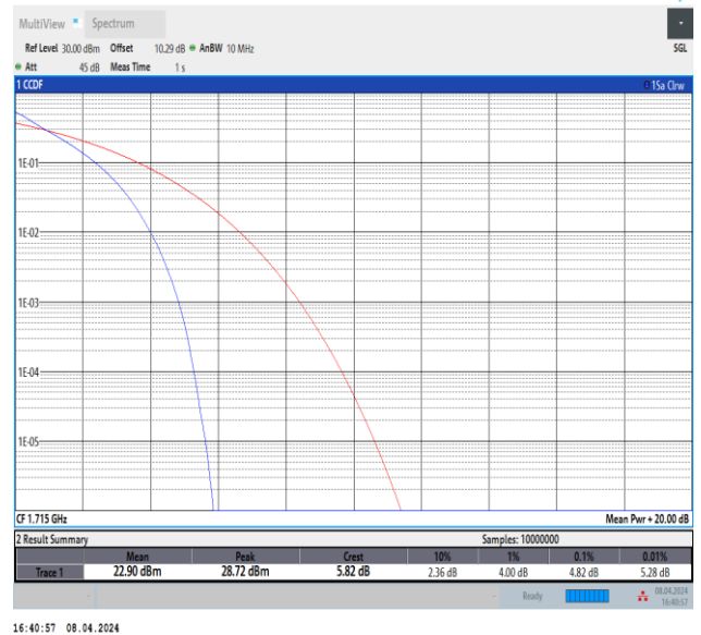
Band66-10MHz-QPSK-132022-50RB#0-PASS
