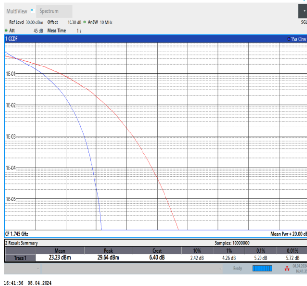
Band66-10MHz-QPSK-132322-50RB#0-PASS
