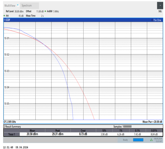
Band38-5MHz-QPSK-38000-25RB#0-PASS
