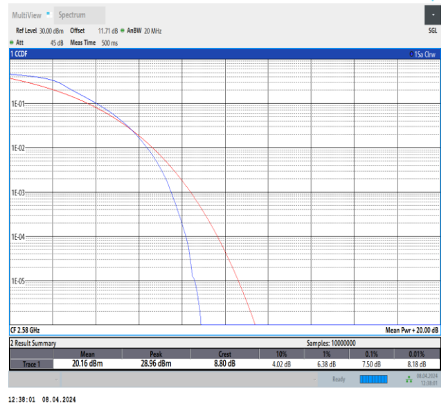
Band38-20MHz-QPSK-37850-100RB#0-PASS
