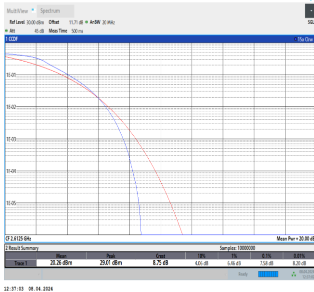
Band38-15MHz-QPSK-38175-75RB#0-PASS
