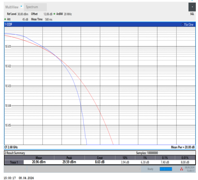
Band41-20MHz-QPSK-41490-100RB#0-PASS
