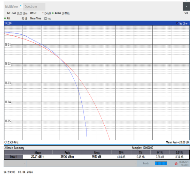
Band41-20MHz-QPSK-39750-100RB#0-PASS
