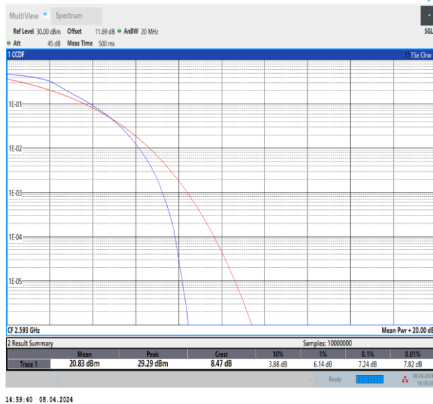
Band41-20MHz-QPSK-40620-100RB#0-PASS
