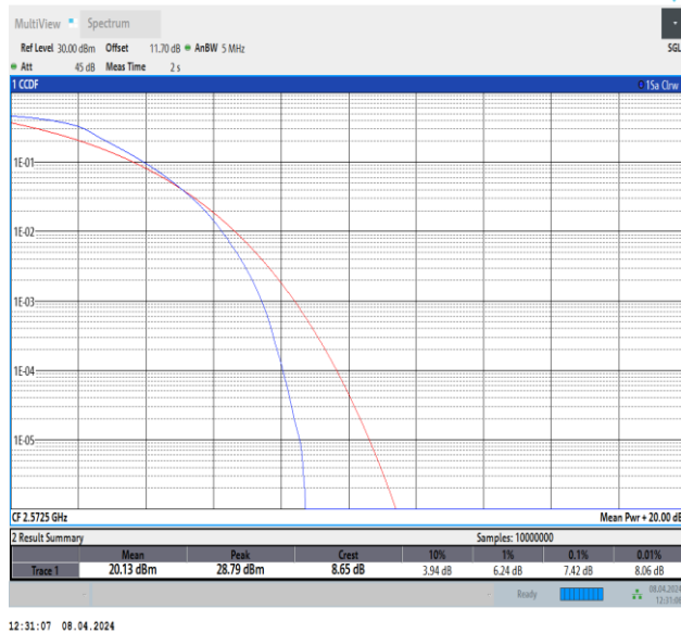
Band38-5MHz-QPSK-37775-25RB#0-PASS
