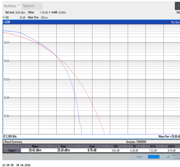
Band38-20MHz-QPSK-38000-100RB#0-PASS
