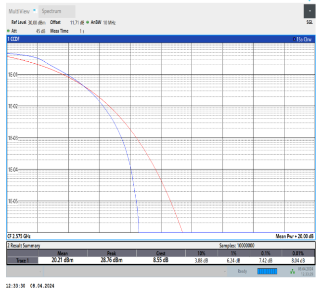
Band38-10MHz-QPSK-37800-50RB#0-PASS
