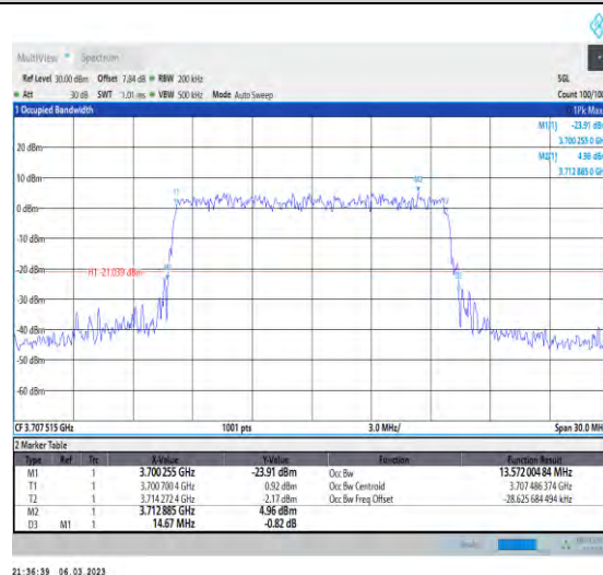
1-N77-3700-3980-PC3-30-15-L-9-CP-256QAM-Outer_Full-38@0-Ant1-13.572-14.670-≤15-PASS
