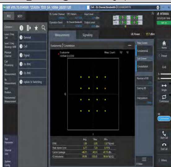
1-N77-3700-3980-PC3-30-100-M-7-CP-16QAM-Outer_Full-273@0-Ant1-see graph-PASS
