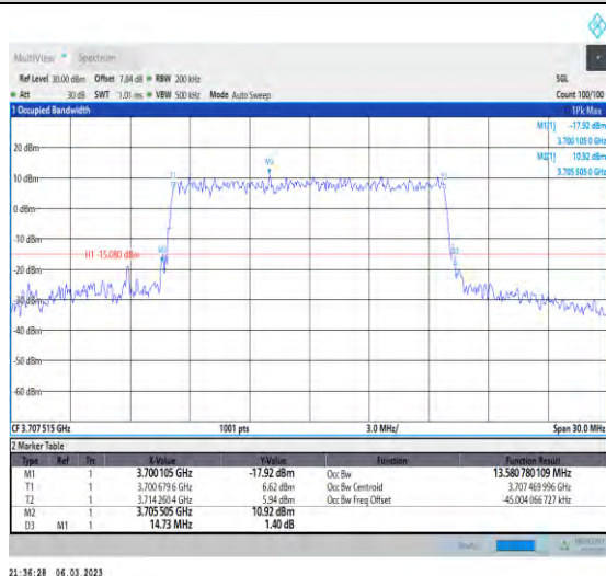
1-N77-3700-3980-PC3-30-15-L-8-CP-64QAM-Outer_Full-38@0-Ant1-13.581-14.730-≤15-PASS
