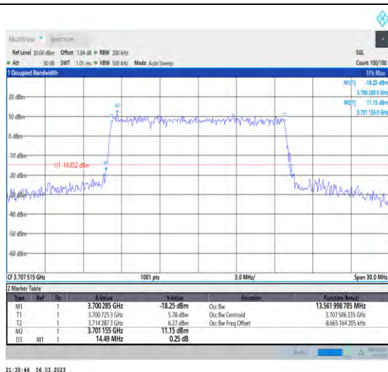
1-N77-3700-3980-PC3-30-15-L-6-CP-QPSK-Outer_Full-38@0-Ant1-13.562-14.490-≤15-PASS
