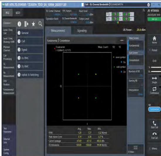
1-N77-3700-3980-PC3-30-100-M-1-DFT-PI2BPSK-Out_Full-270@0-Ant1-see graph-PASS
