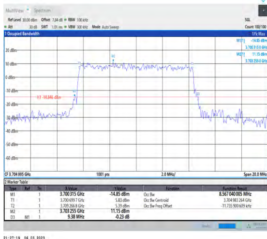
1-N77-3700-3980-PC3-30-10-L-3-DFT-16QAM-Outer_Full-24@0-Ant1-8.567-9.380-≤10-PASS
