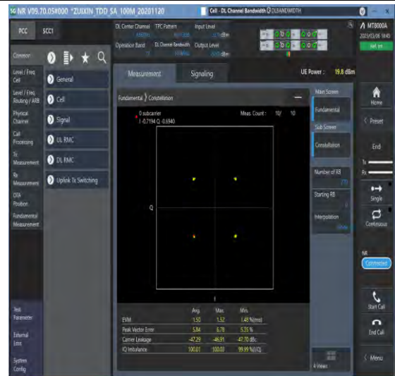
1-N77-3700-3980-PC3-30-100-M-2-DFT-QPSK-Out_Full-270@0-Ant1-see graph-PASS
