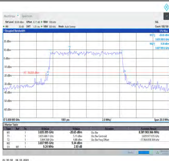
1-N77-3700-3980-PC3-30-10-M-6-CP-QPSK-Outer_Full-24@0-Ant1-8.582-9.240-≤10-PASS
