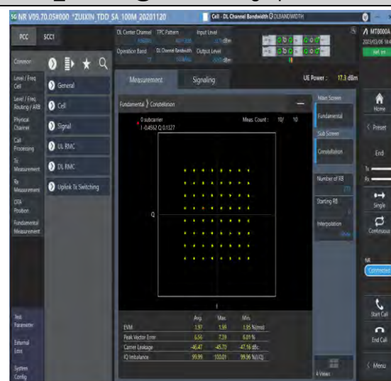
1-N77-3700-3980-PC3-30-100-M-8-CP-64QAM-Outer_Full-273@0-Ant1-see graph-PASS
