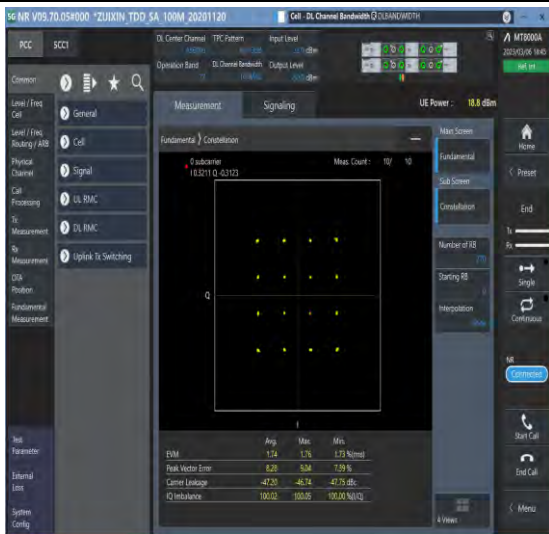
1-N77-3700-3980-PC3-30-100-M-3-DFT-16QAM-Out_Full-270@0-Ant1-see graph-PASS
