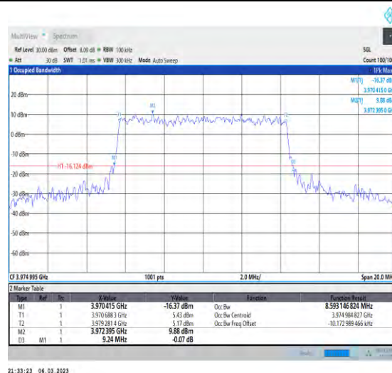
1-N77-3700-3980-PC3-30-10-H-6-CP-QPSK-Oute_r_ Full-24@0-Ant1-8.593-9.240-≤10-PASS
