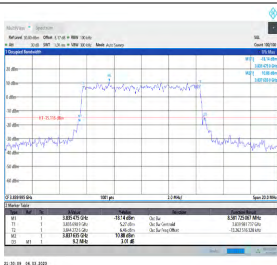
1-N77-3700-3980-PC3-30-10-M-4-DFT-64QAM-Outer_Full-24@0-Ant1-8.582-9.200-≤10-PASS
