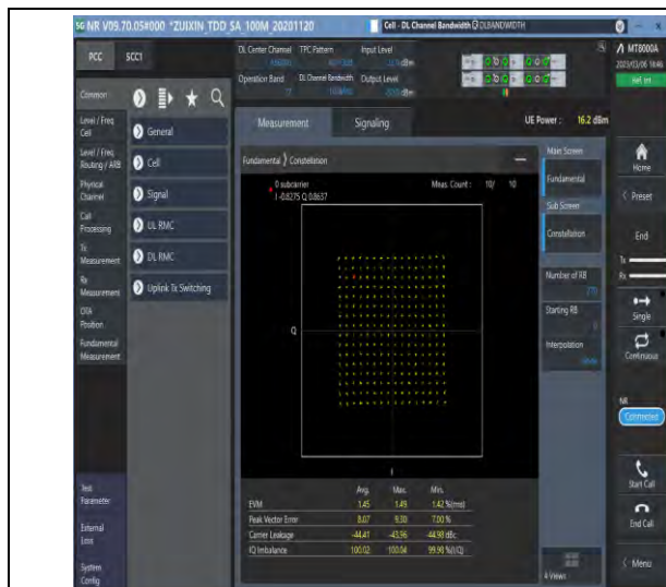
1-N77-3700-3980-PC3-30-100-M-5-DFT-256QAM-Outer_Full-270@0-Ant1-see graph-PASS
