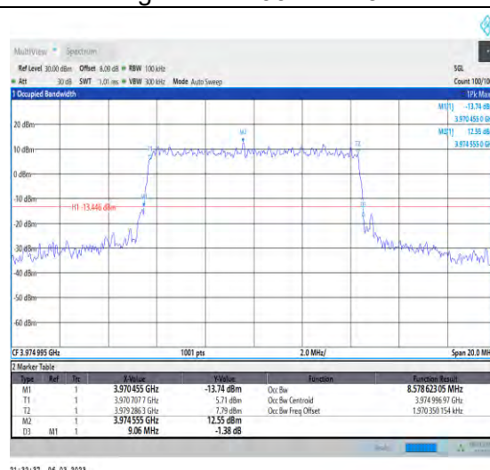
1-N77-3700-3980-PC3-30-10-H-4-DFT-64QAM-Oute r_Full-24@0-Ant1-8.579-9.060-≤10-PASS
