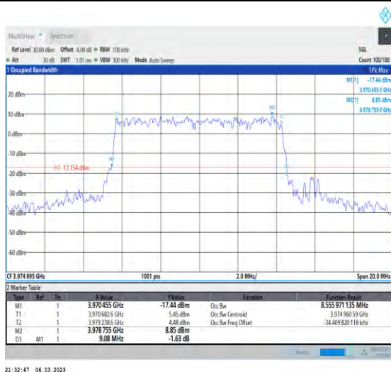
1-N77-3700-3980-PC3-30-10-H-5-DFT-256QAM-Out er_Full-24@0-Ant1-8.556-9.080-≤10-PASS
