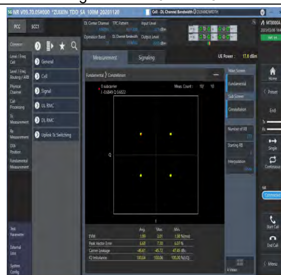
1-N77-3700-3980-PC3-30-100-M-6-CP-QPSK-Outer_Full-273@0-Ant1-see graph-PASS
