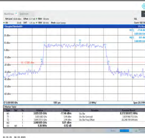
1-N77-3700-3980-PC3-30-10-M-7-CP-16QAM-Outer_Full-24@0-Ant1-8.574-9.360-≤10-PASS
