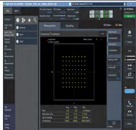
1-N77-3700-3980-PC3-30-100-M-4-DFT-64QAM-Out_Full-270@0-Ant1-see graph-PASS
