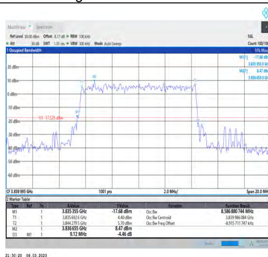
1-N77-3700-3980-PC3-30-10-M-5-DFT-256QAM-Outer_Full-24@0-Ant1-8.587-9.120-≤10-PASS
