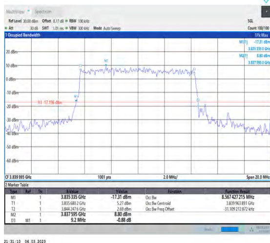
1-N77-3700-3980-PC3-30-10-M-8-CP-64QAM-Outer_Full-24@0-Ant1-8.567-9.200-≤10-PASS
