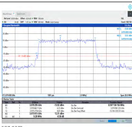
1-N77-3700-3980-PC3-30-10-H-3-DFT-16QAM-Oute r_Full-24@0-Ant1-8.597-9.280-≤10-PASS
