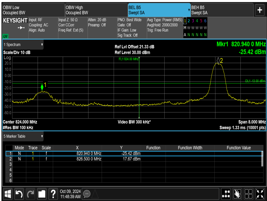
Figure 13 - Lower Band Edge, 826.5 MHz, Modulation: \pi/2 -BPSK, SCS: 3.75 kHz, Tone Number: 1, Start Sub-Carrier: 0
