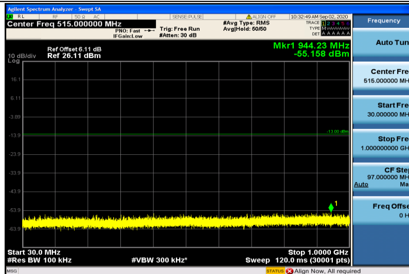
Band2-10MHz-QPSK-18900-1RB#0-30~1000MHz
