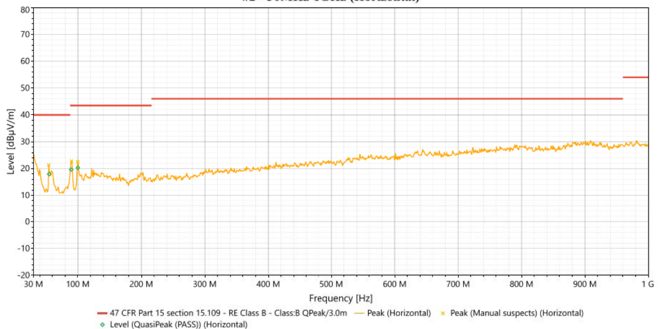
#2 - 30MHz-1GHz (Horizontal)
