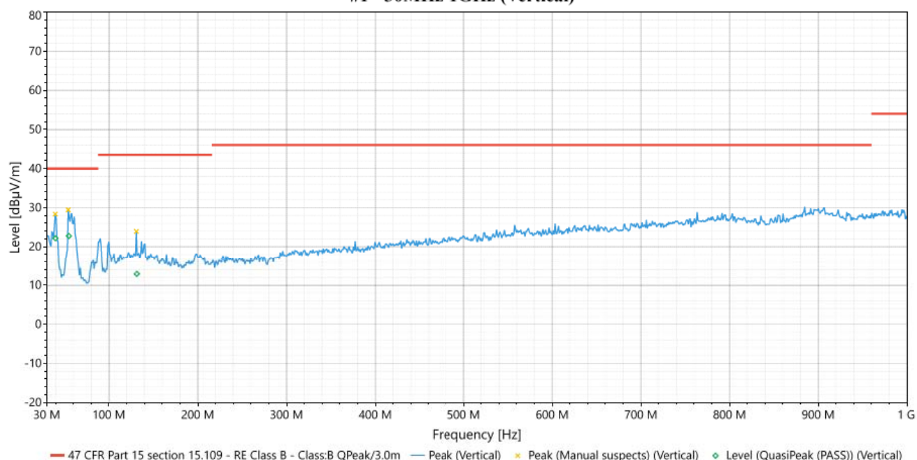
#1 - 30MHz-1GHz (Vertical)
