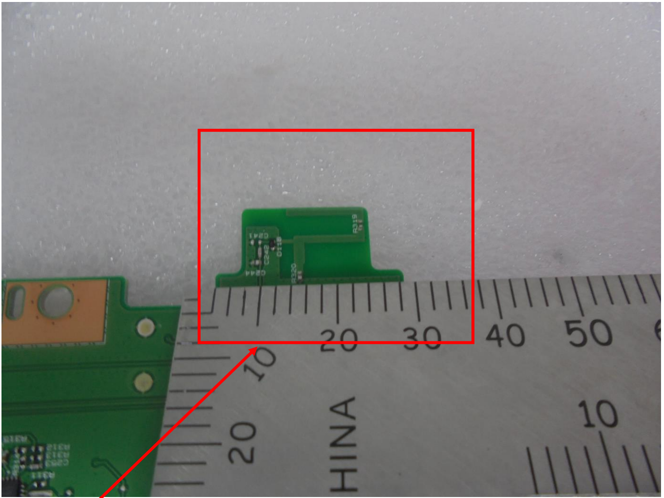
BT Antenna
