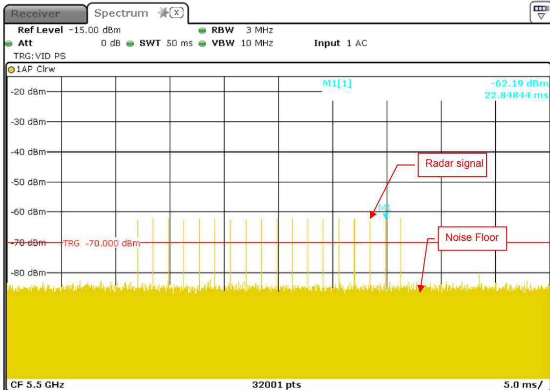
Radar Signal 0
