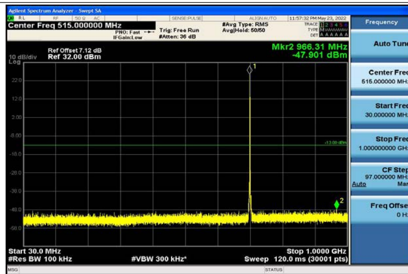
Band12-1.4MHz-16QAM-23095-1RB#0-30~1000MHz
