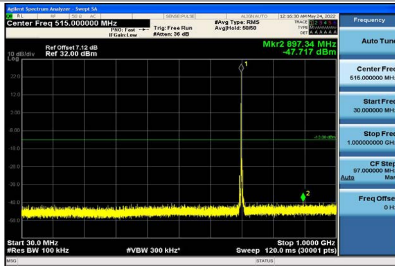
Band12-3MHz-16QAM-23095-1RB#0-30~1000MHz
