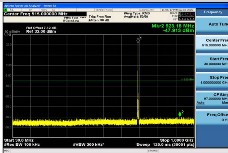
Band12-1.4MHz-16QAM-23017-1RB#0-30~1000MHz
