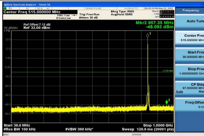
Band5-5MHz-16QAM-20625-1RB#0-30~1000MHz
