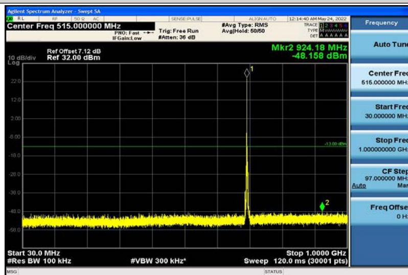
Band12-3MHz-QPSK-23025-1RB#0-30~1000MHz
