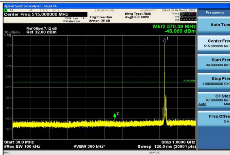
Band5-5MHz-QPSK-20525-1RB#0-30~1000MHz
