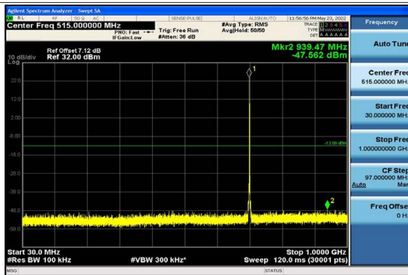
Band12-1.4MHz-QPSK-23095-1RB#0-30~1000MHz
