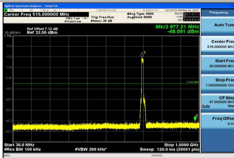
Band12-10MHz-QPSK-23060-1RB#0-30~1000MHz
