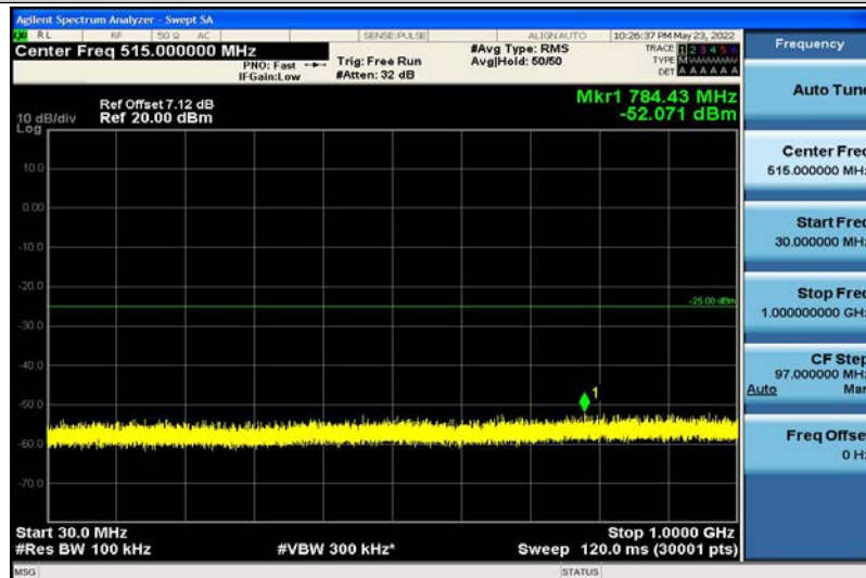
Band7-5MHz-QPSK-21425-1RB#0-30~1000MHz
