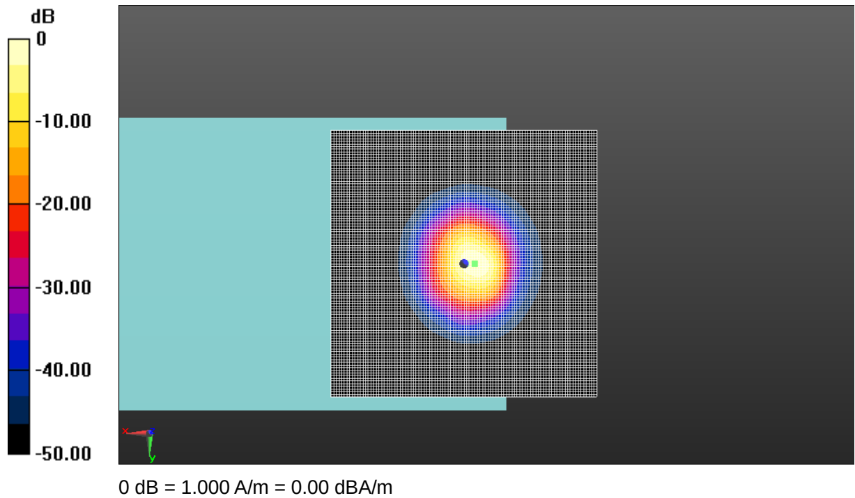
Fig A.17 T-Coil LTE-Band 12
