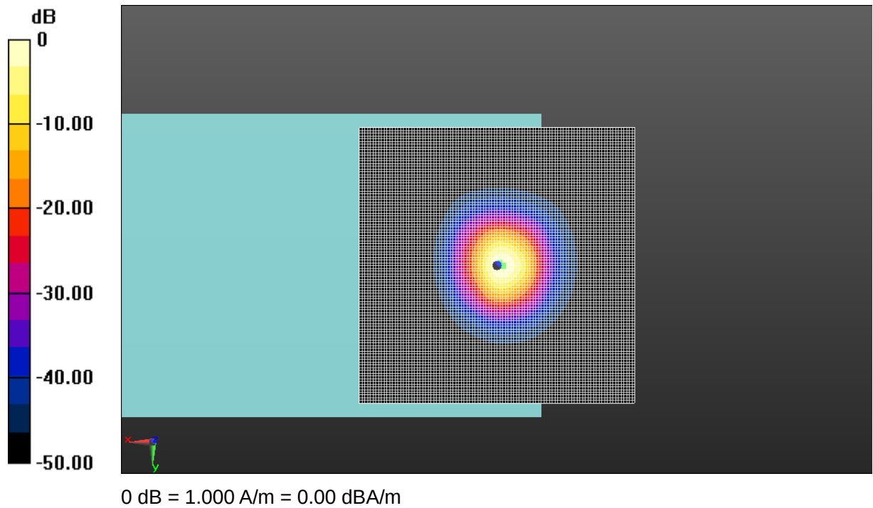
Fig A.1 T-Coil GSM 850
