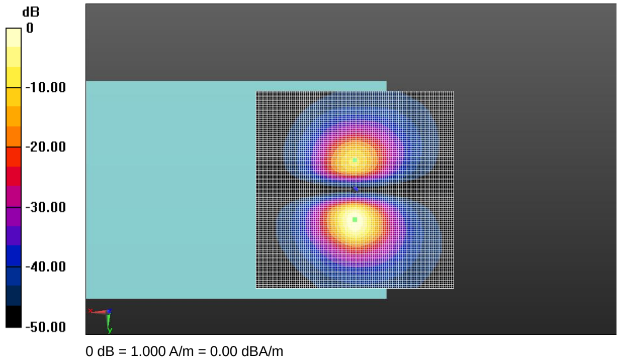
Fig A.2 T-Coil GSM 850
