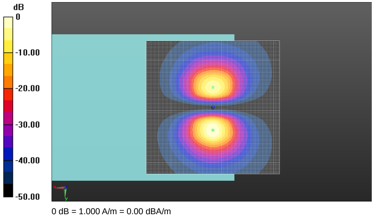
Fig A.4 T-Coil GSM 1900
