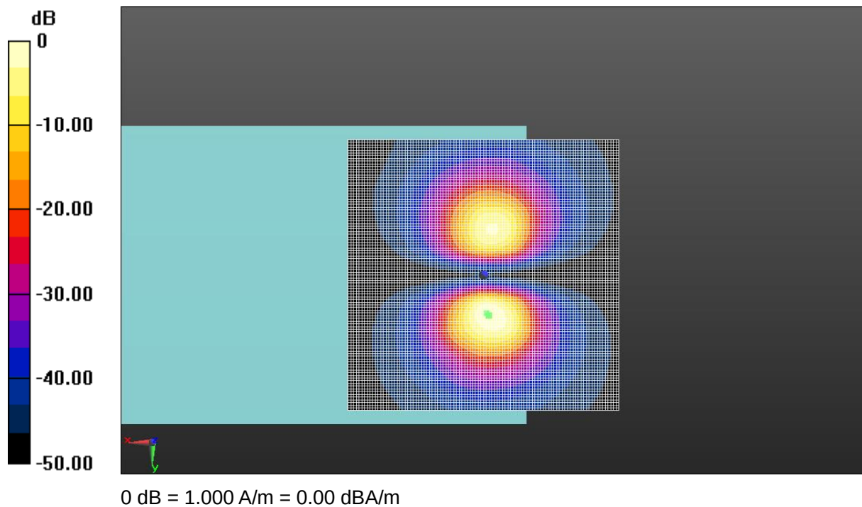
Fig A.20 T-Coil LTE-Band 66
