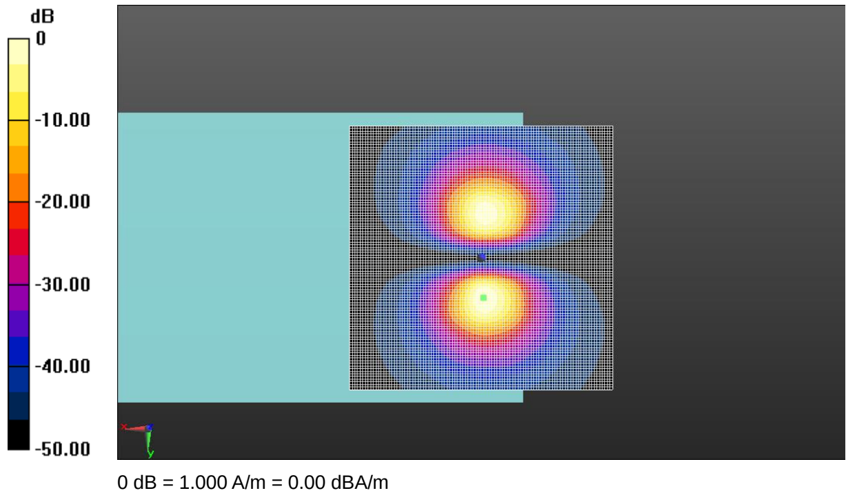
Fig A.18 T-Coil LTE-Band 12
