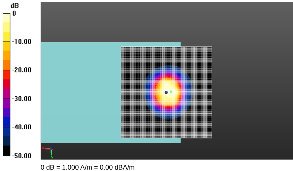
Fig A.19 T-Coil LTE-Band 66
