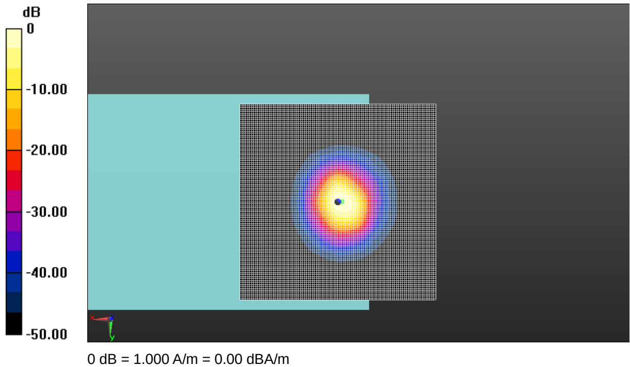
Fig A.23 T-Coil WIFI 2.4G
