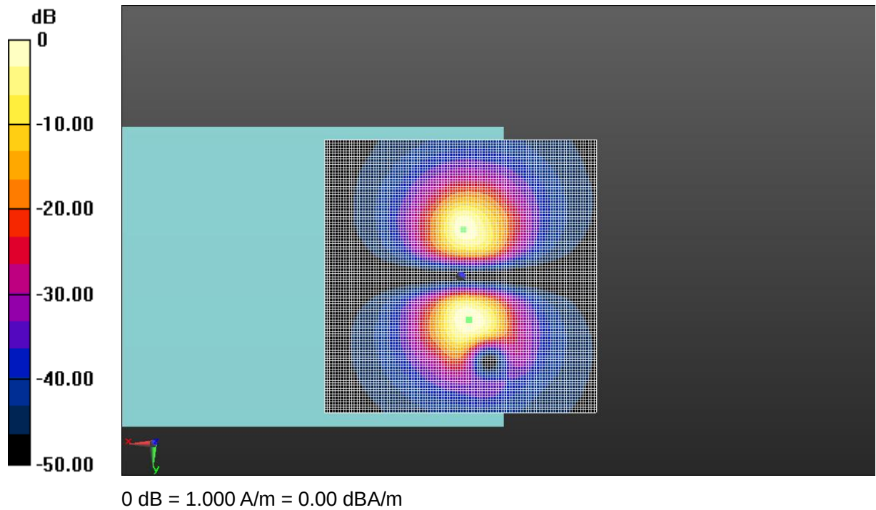
Fig A.24 T-Coil WIFI 2.4G
