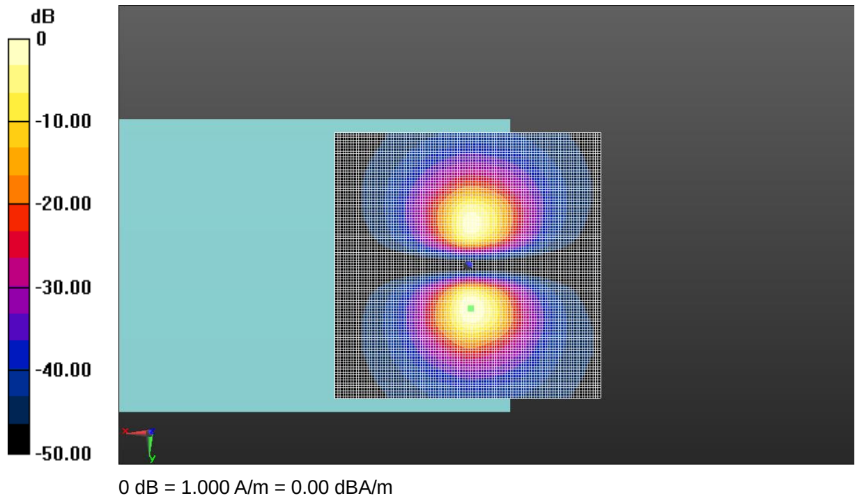
Fig A.12 T-Coil LTE-Band 2
