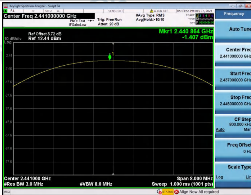
Peak_Output_Power_NVNT_ANT1_1-DH5_2441
