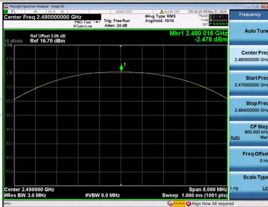
Peak_Output_Power_NVNT_ANT1_1-DH5_2480
