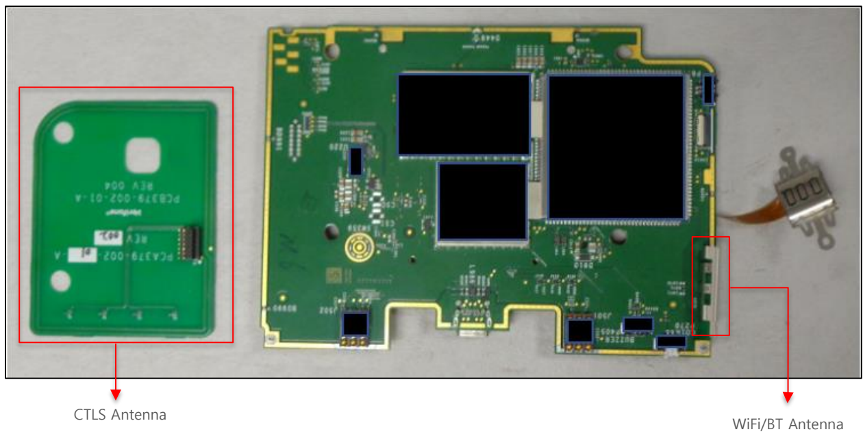
PCB Top Views
