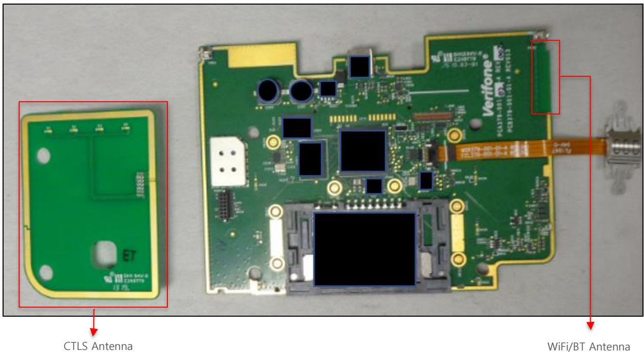
PCB Bottom Views
