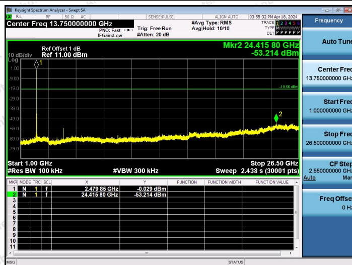
Zigbee-Ant1-2480-1000~26500-PASS
