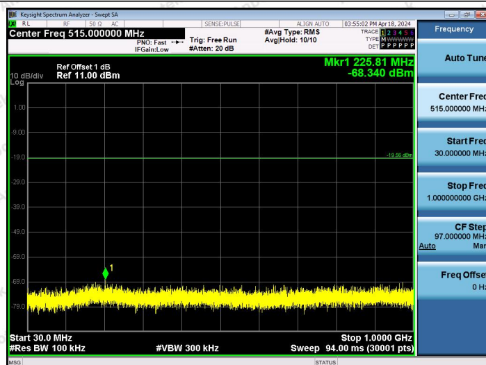
Zigbee-Ant1-2480-30~1000-PASS
