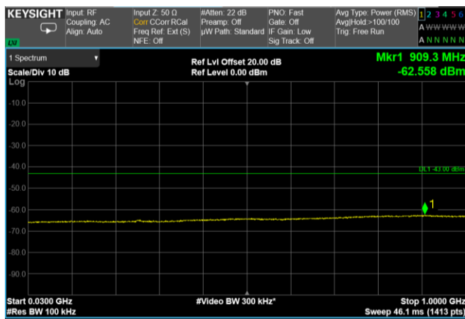
Channel: TOP, Modulation: 64QAM, BW=20MHz, Range: 30 MHz – 1000 MHz
