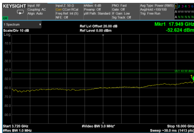
Channel: TOP, Modulation: 64QAM, BW=10MHz, Range: 3720 MHz – 18 GHz
