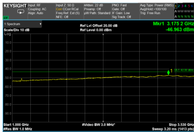
Channel: TOP, Modulation: 64QAM, BW=15MHz, Range: 1000 MHz – 3530 MHz
