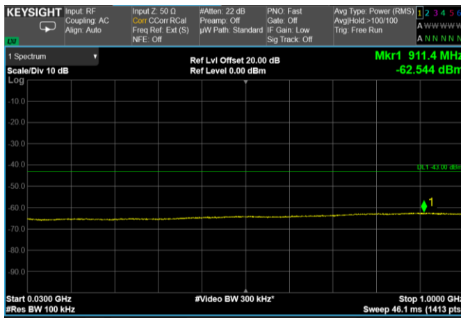
Channel: TOP, Modulation: 64QAM, BW=60MHz, Range: 30 MHz - 1000 MHz
