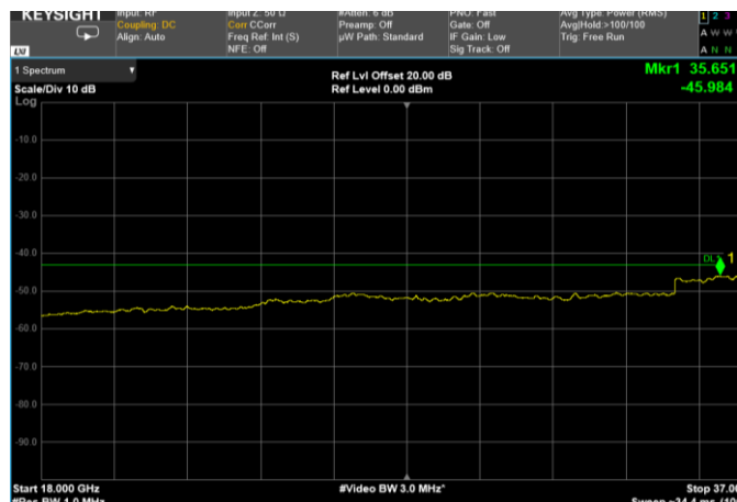
Channel: TOP, Modulation: 64QAM, BW=10MHz, Range: 18 GHz – 37 GHz
