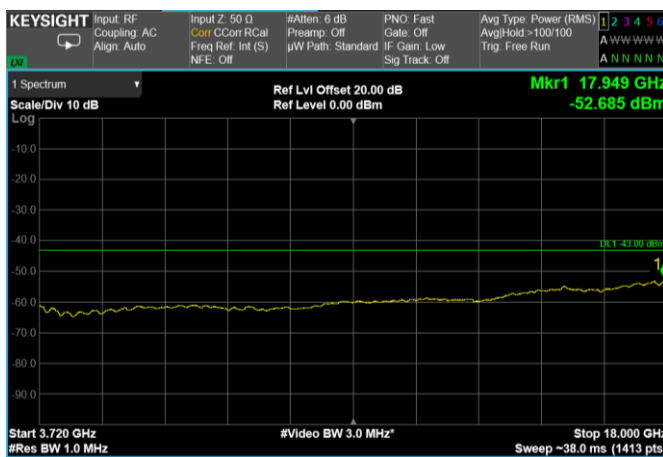
Channel: BOTTOM, Modulation: 64QAM, BW=15MHz, Range: 3720 MHz – 18 GHz
