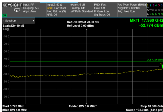
Channel: TOP, Modulation: 64QAM, BW=15MHz, Range: 3720 MHz – 18 GHz
