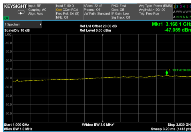
Channel: MIDDLE, Modulation: 64QAM, BW=25MHz, Range: 1000 MHz - 3530 MHz
