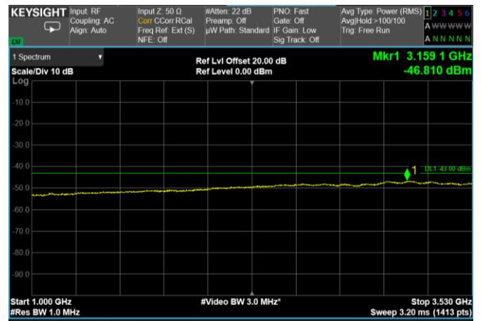
Channel: TOP, Modulation: 64QAM, BW=60MHz, Range: 1000 MHz - 3530 MHz
