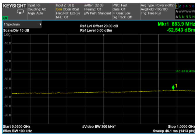
Channel: TOP, Modulation: 64QAM, BW=15MHz, Range: 30 MHz – 1000 MHz
