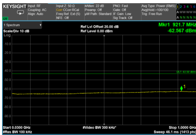
Channel: MIDDLE, Modulation: 64QAM, BW=60MHz, Range: 30 MHz – 1000 MHz
