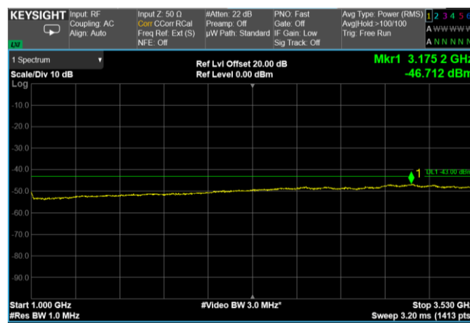
Channel: BOTTOM, Modulation: 64QAM, BW=25MHz, Range: 1000 MHz - 3530 MHz
