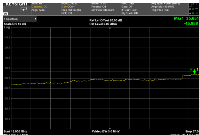
Channel: TOP, Modulation: 64QAM, BW=15MHz, Range: 18 GHz – 37 GHz
