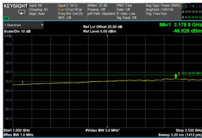
Channel: TOP, Modulation: 64QAM, BW=10MHz, Range: 1000 MHz – 3530 MHz
