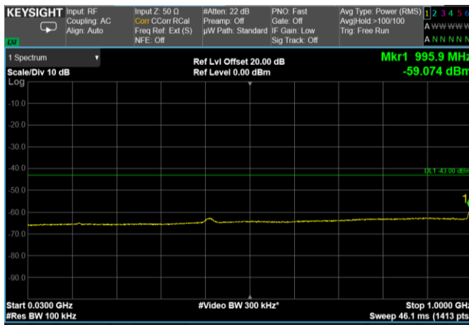
Channel: BOTTOM, Modulation: 64QAM, BW=15MHz, Range: 30 MHz – 1000 MHz
