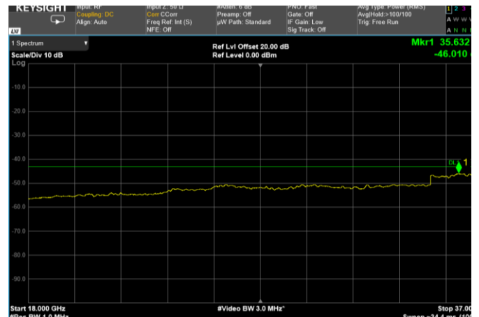
Channel: TOP, Modulation: 64QAM, BW=60MHz, Range: 18 GHz - 37 GHz
