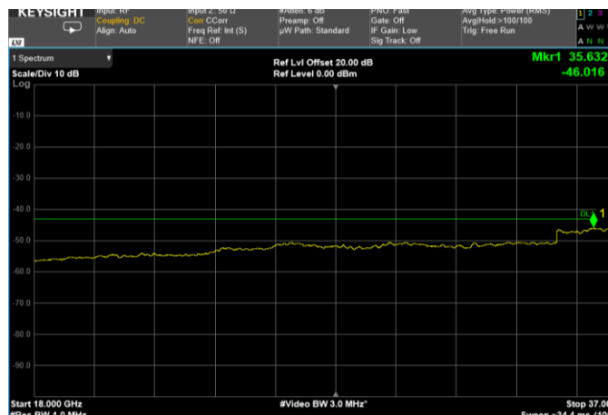
Channel: MIDDLE, Modulation: 64QAM, BW=60MHz, Range: 18 GHz – 37 GHz
