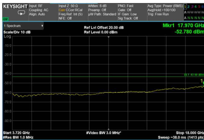
Channel: MIDDLE, Modulation: 64QAM, BW=25MHz, Range: 3720 MHz - 18 GHz
