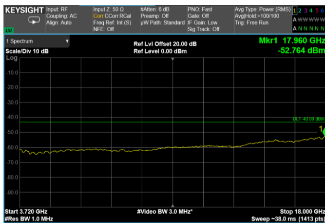
Channel: MIDDLE, Modulation: 64QAM, BW=10MHz, Range: 3720 MHz – 18 GHz
