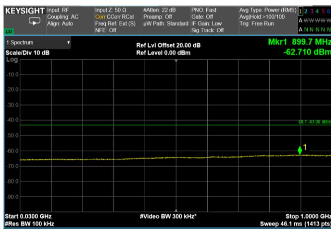
Channel: MIDDLE, Modulation: 64QAM, BW=25MHz, Range: 30 MHz - 1000 MHz
