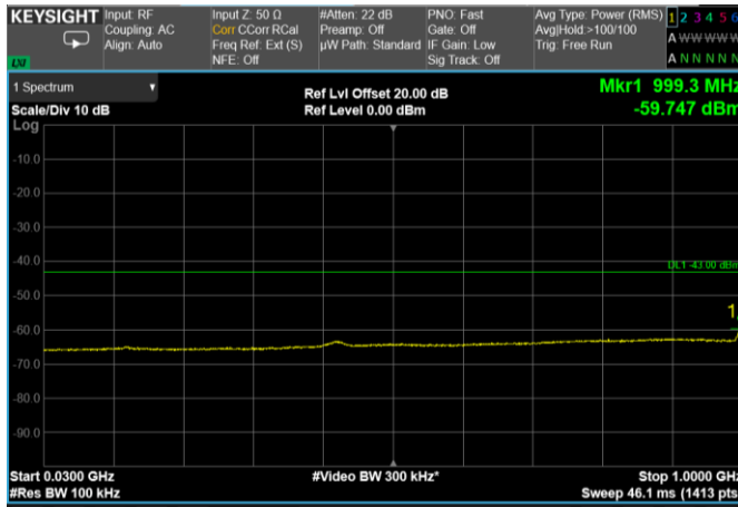
Channel: BOTTOM, Modulation: 64QAM, BW=20MHz, Range: 30 MHz – 1000 MHz
