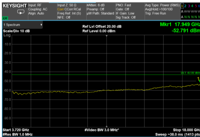
Channel: TOP, Modulation: 64QAM, BW=60MHz, Range: 3720 MHz - 18 GHz
