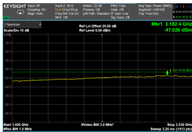
Channel: MIDDLE, Modulation: 64QAM, BW=60MHz, Range: 1000 MHz – 3530 MHz
