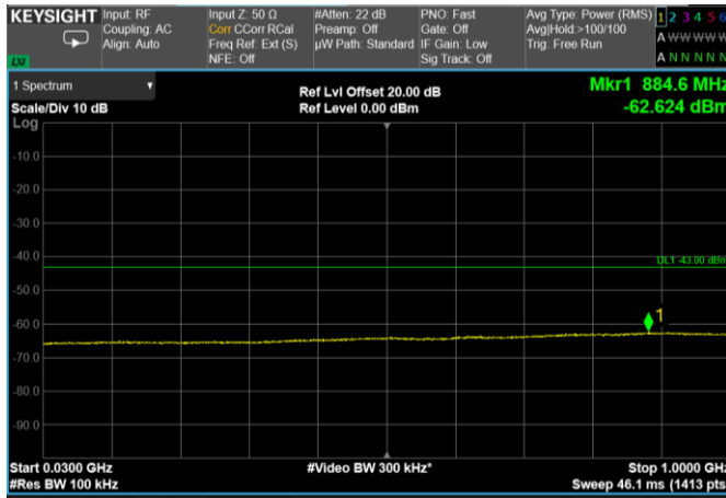
Channel: MIDDLE, Modulation: 64QAM, BW=30MHz, Range: 30 MHz – 1000 MHz
