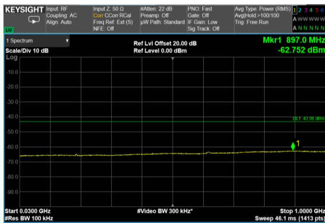
Channel: MIDDLE, Modulation: 64QAM, BW=10MHz, Range: 30 MHz – 1000 MHz
