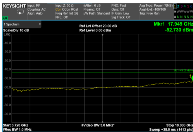
Channel: MIDDLE, Modulation: 64QAM, BW=60MHz, Range: 3720 MHz – 18 GHz
