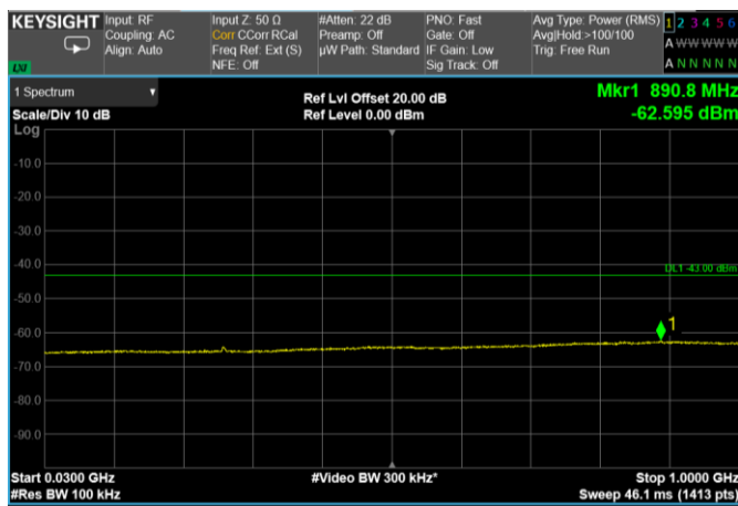
Channel: TOP, Modulation: 64QAM, BW=10MHz, Range: 30 MHz – 1000 MHz
