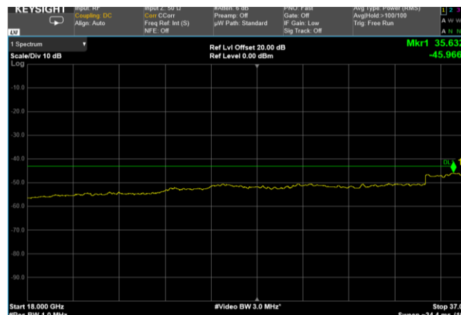
Channel: MIDDLE, Modulation: 64QAM, BW=25MHz, Range: 18 GHz - 37 GHz
