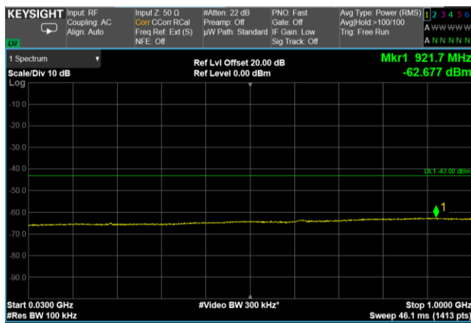
Channel: MIDDLE, Modulation: 64QAM, BW=15MHz, Range: 30 MHz – 1000 MHz
