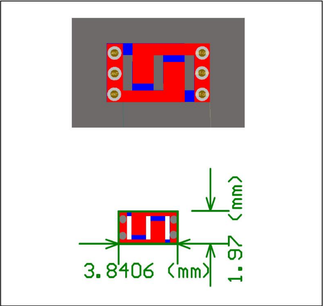
产品规格图(Antenna Specification chart)
