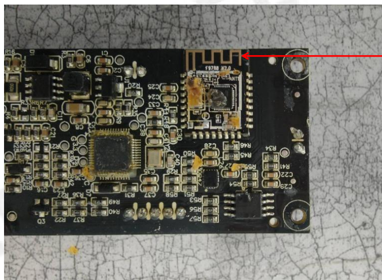
Bluetooth Antenna
