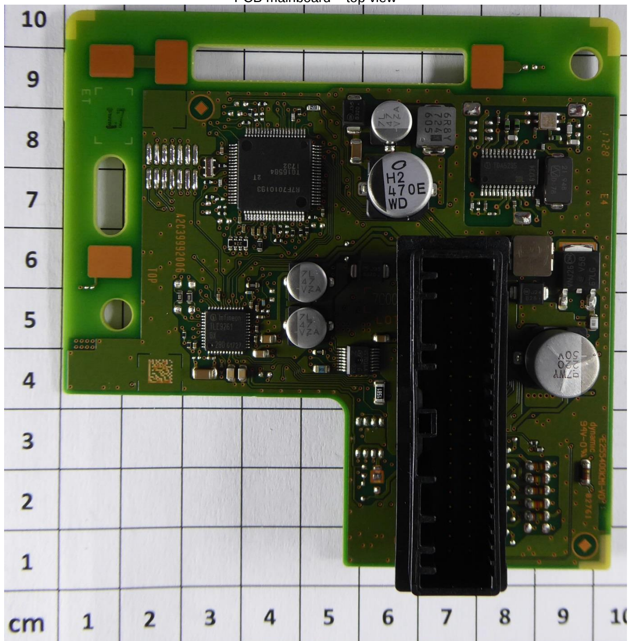
PCB mainboard – top view
