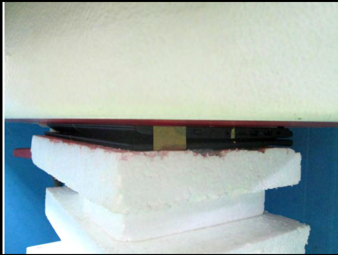
Body - Rear Face of EUT at 0 mm (EUT 1)
