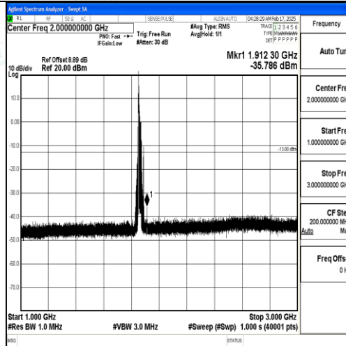
Band25_20MHz_QPSK_26140_1RB#0_1000~3000_1000~3000
