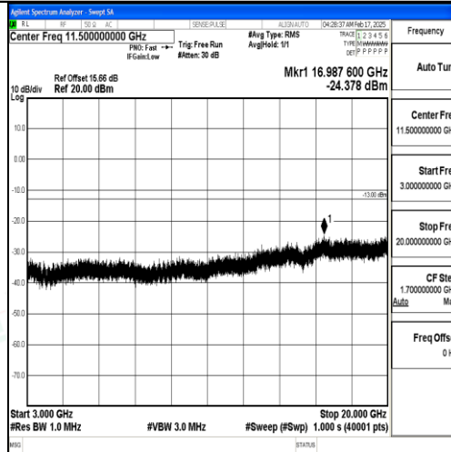
Band25_20MHz_QPSK_26140_1RB#0_3000~20000_3000~20000
