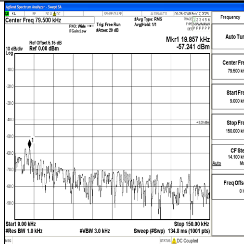
Band25_20MHz_16QAM_26140_1RB#0_0.009~0.15_0.009~0.15
