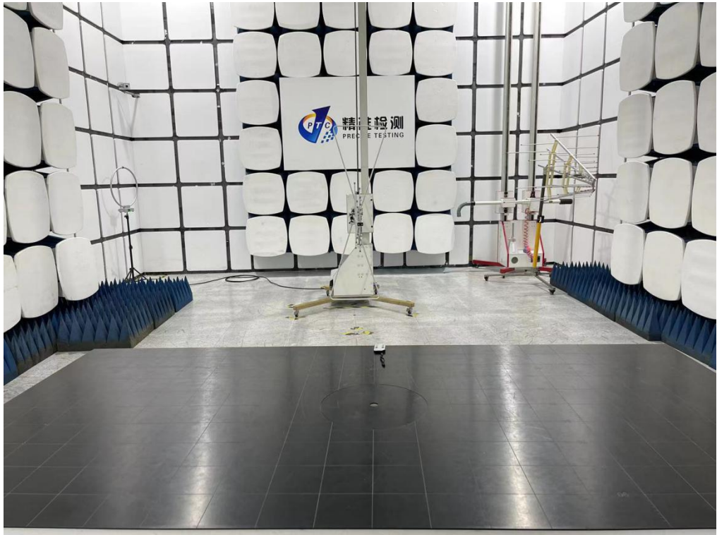
Radiated Spurious Emissions From 30MHz-1000MHz
