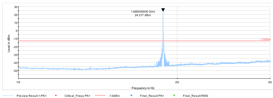
Plot #17 Radiated Emissions: 1-3 GHz
