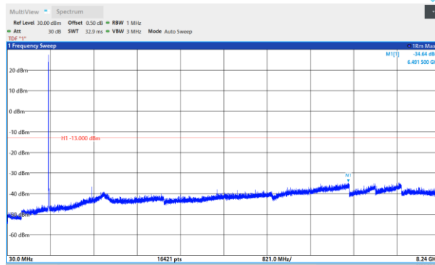
Band26-3MHz-QPSK-26775-1RB#0- Range1:30~8240MHz
