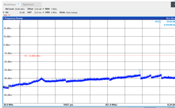
Band26-1.4MHz-64QAM-26740-1RB#0- Range1:30~8240MHz
