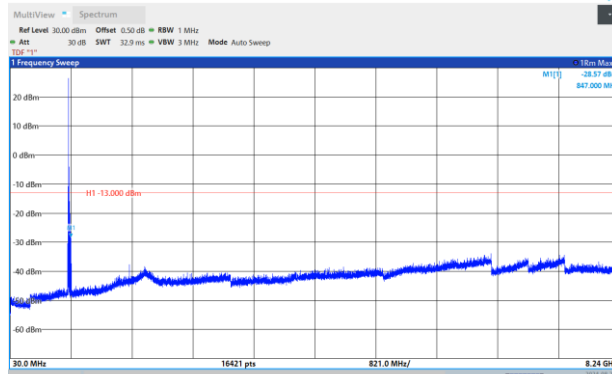
Band26-3MHz-QPSK-26705-1RB#0- Range1:30~8240MHz
