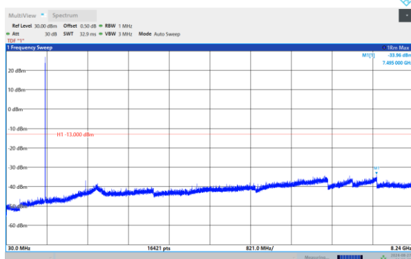
Band26-3MHz-QPSK-26740-1RB#0- Range1:30~8240MHz
