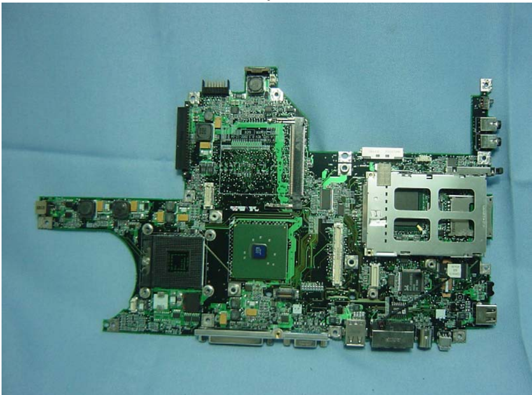
Main Board of Notebook -5
