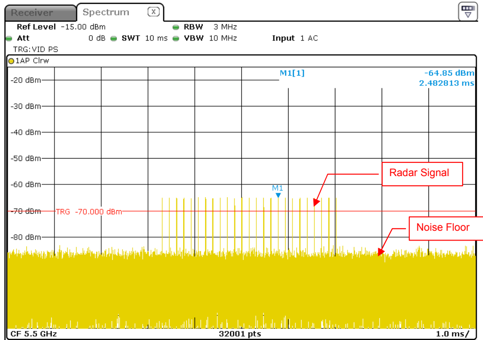
Radar Signal 2
