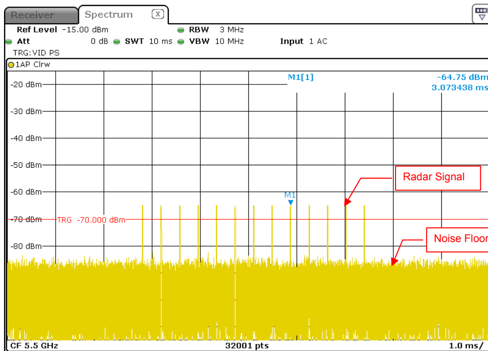
Radar Signal 4
