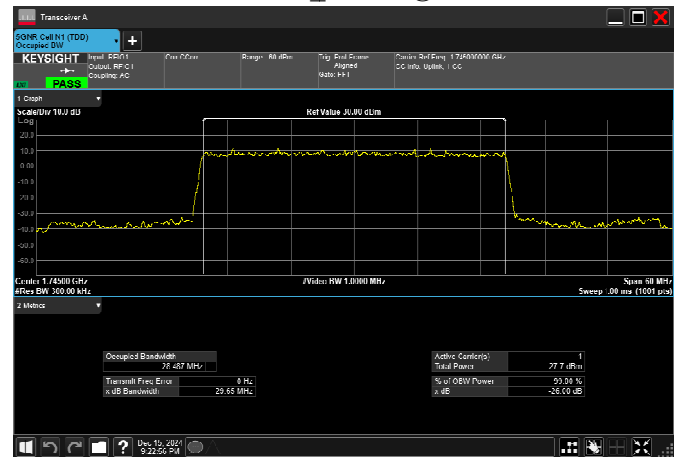
n66_30MHz_15kHz_1745MHz_DFT-s-OFDM 16 QAM_RB160@0
