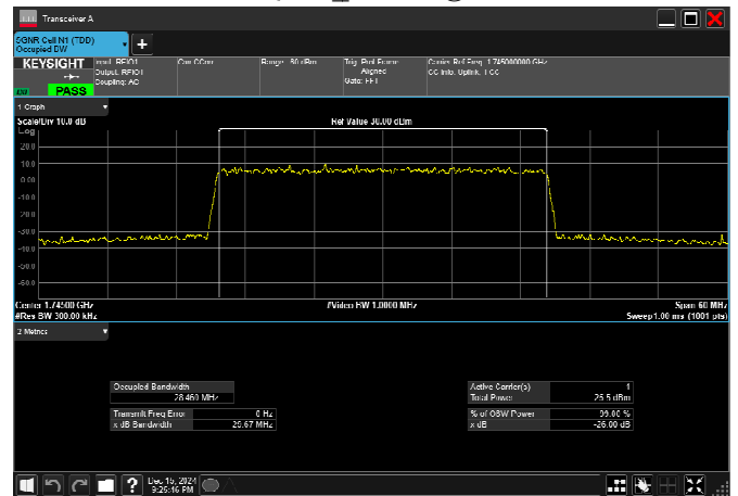
n66_30MHz_15kHz_1745MHz_CP-OFDM 256 QAM_RB160@0
