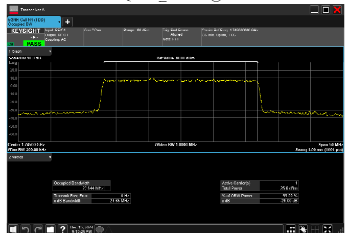
n66_25MHz_15kHz_1745MHz_CP-OFDM QPSK_RB133@0
