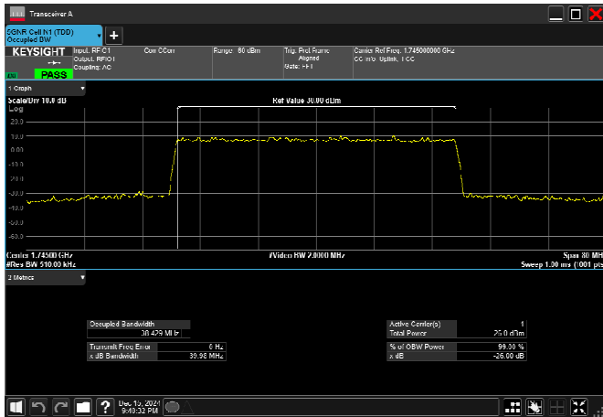
n66_40MHz_15kHz_1745MHz_CP-OFDM 16 QAM_RB216@0
