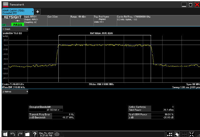
n66_40MHz_15kHz_1745MHz_DFT-s-OFDM 16 QAM_RB216@0
