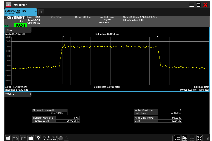
n66_40MHz_15kHz_1745MHz_DFT-s-OFDM 64 QAM_RB216@0
