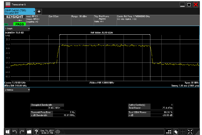
n66_40MHz_15kHz_1745MHz_CP-OFDM 64 QAM_RB216@0
