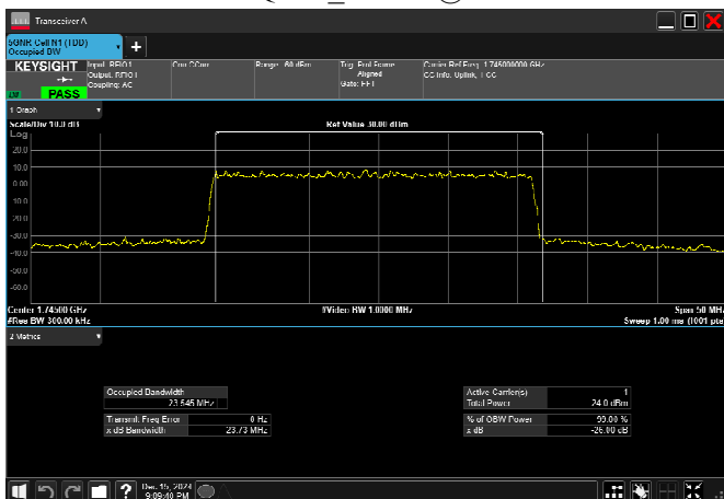
n66_25MHz_15kHz_1745MHz_DFT-s-OFDM 256 QAM_RB128@0
