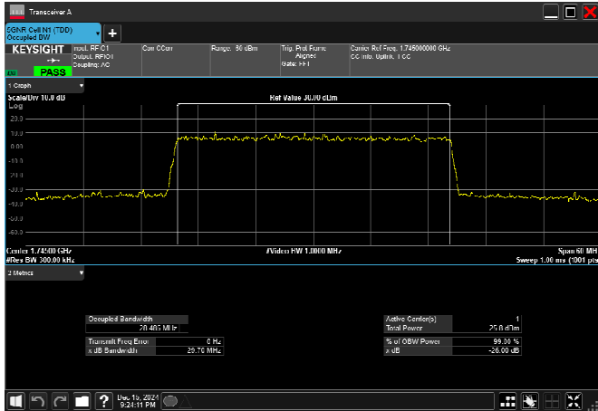
n66_30MHz_15kHz_1745MHz_CP-OFDM QPSK_RB160@0
