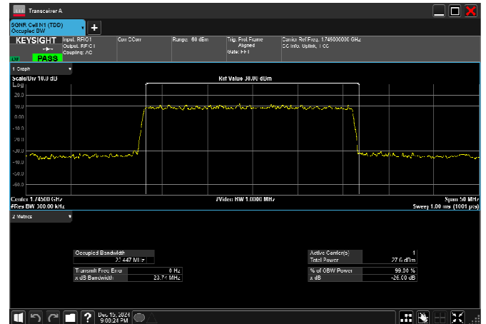
n66_25MHz_15kHz_1745MHz_DFT-s-OFDM 64 QAM_RB128@0
