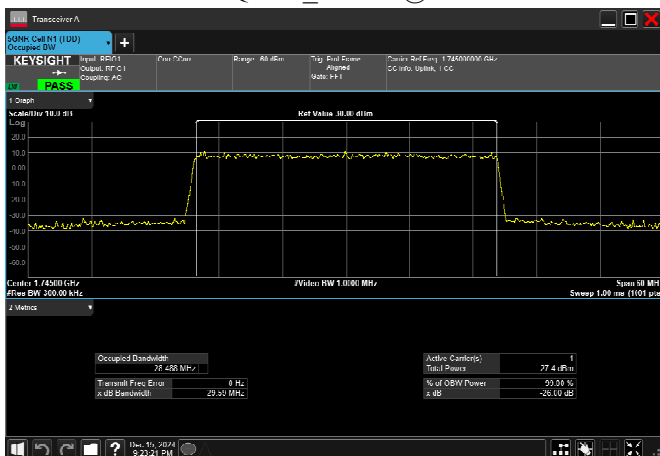
n66_30MHz_15kHz_1745MHz_DFT-s-OFDM QPSK_RB160@0
