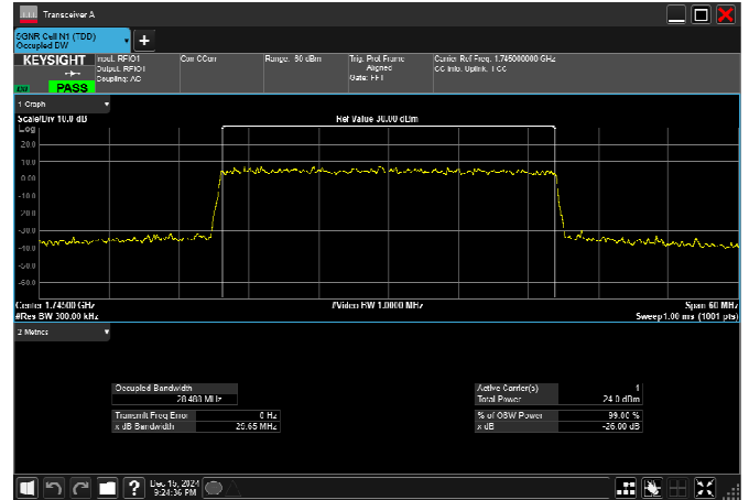
n66_30MHz_15kHz_1745MHz_CP-OFDM 16 QAM_RB160@0
