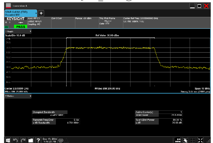
n7_5MHz_15kHz_2535MHz_DFT-s-OFDM 16 QAM_RB25@0
