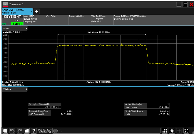
n66_25MHz_15kHz_1745MHz_CP-OFDM 256 QAM_RB133@0
