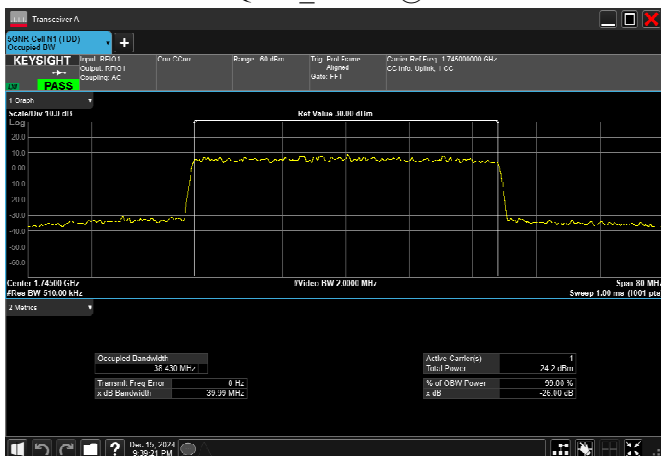
n66_40MHz_15kHz_1745MHz_DFT-s-OFDM 256 QAM_RB216@0
