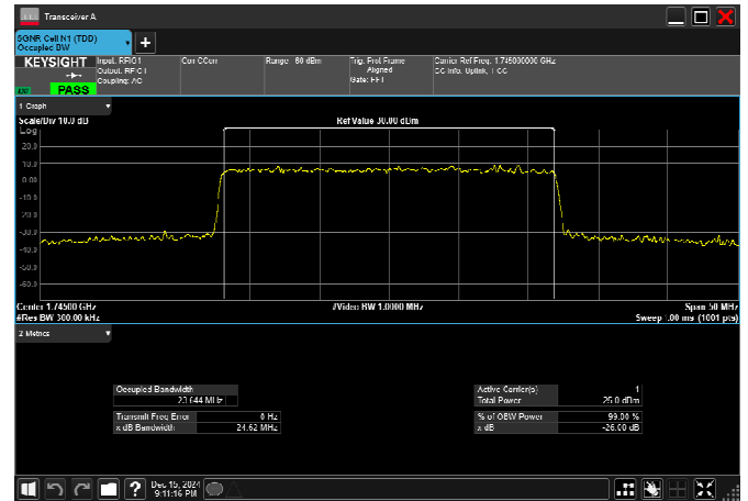
n66_30MHz_15kHz_1745MHz_DFT-s-OFDM \pi/2 BPSK_RB160@0
