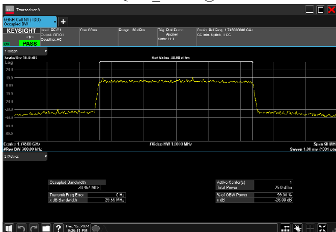
n66_30MHz_15kHz_1745MHz_CP-OFDM 64 QAM_RB160@0
