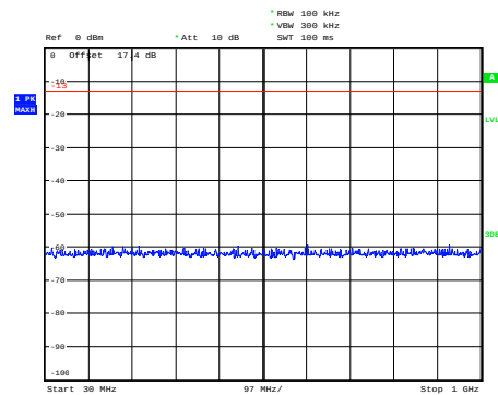
WCDMA Band IV CH-Middle 30MHz~1GHz
