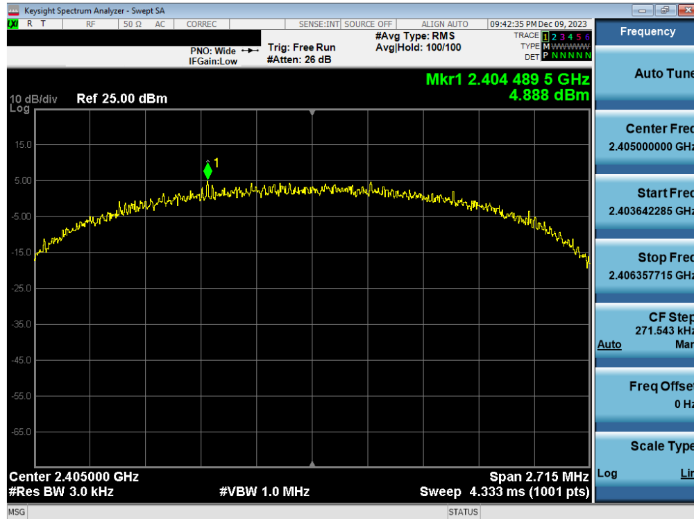
Plot 7-13. Power Spectral Density Antenna WF2b (802.15.4, ePA – Ch. 11)
