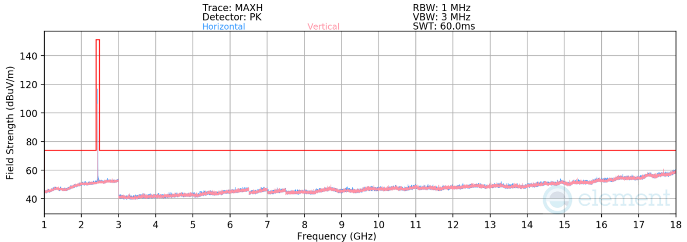
Plot 7-36. Radiated Spurious Emissions 1-18GHz Antenna WF7b (802.15.4, ePA – Ch. 18)
