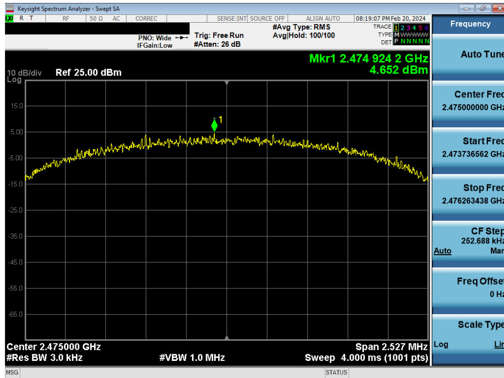
Plot 7-9. Power Spectral Density Antenna WF7b (802.15.4, ePA – Ch. 25)
