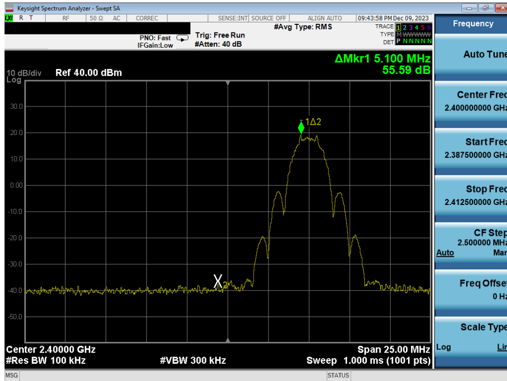
Plot 7-21. Band Edge Antenna WF2b (802.15.4, ePA – Ch. 11)
