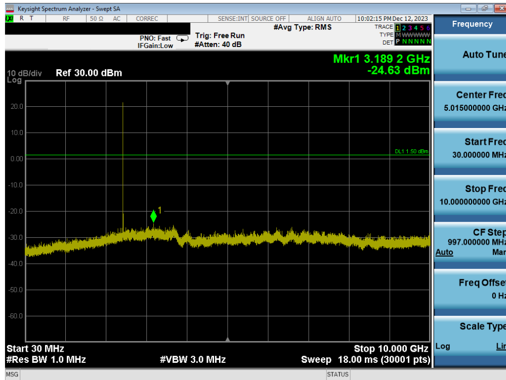
Plot 7-31. Conducted Spurious Antenna WF2b (802.15.4, ePA – Ch. 18)
