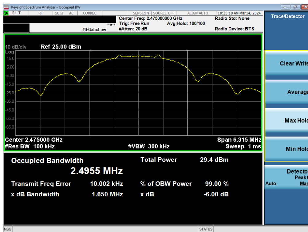
Plot 7-6. 6dB BW & 99% OBW Antenna WF2b(802.15.4, Ch. 25)
