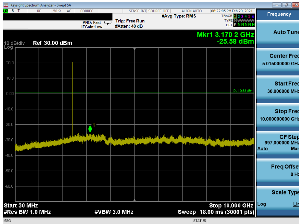
Plot 7-25. Conducted Spurious Antenna WF7b (802.15.4, ePA – Ch. 18)
