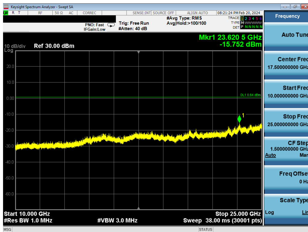
Plot 7-24. Conducted Spurious Antenna WF7b (802.15.4, ePA – Ch. 11)
