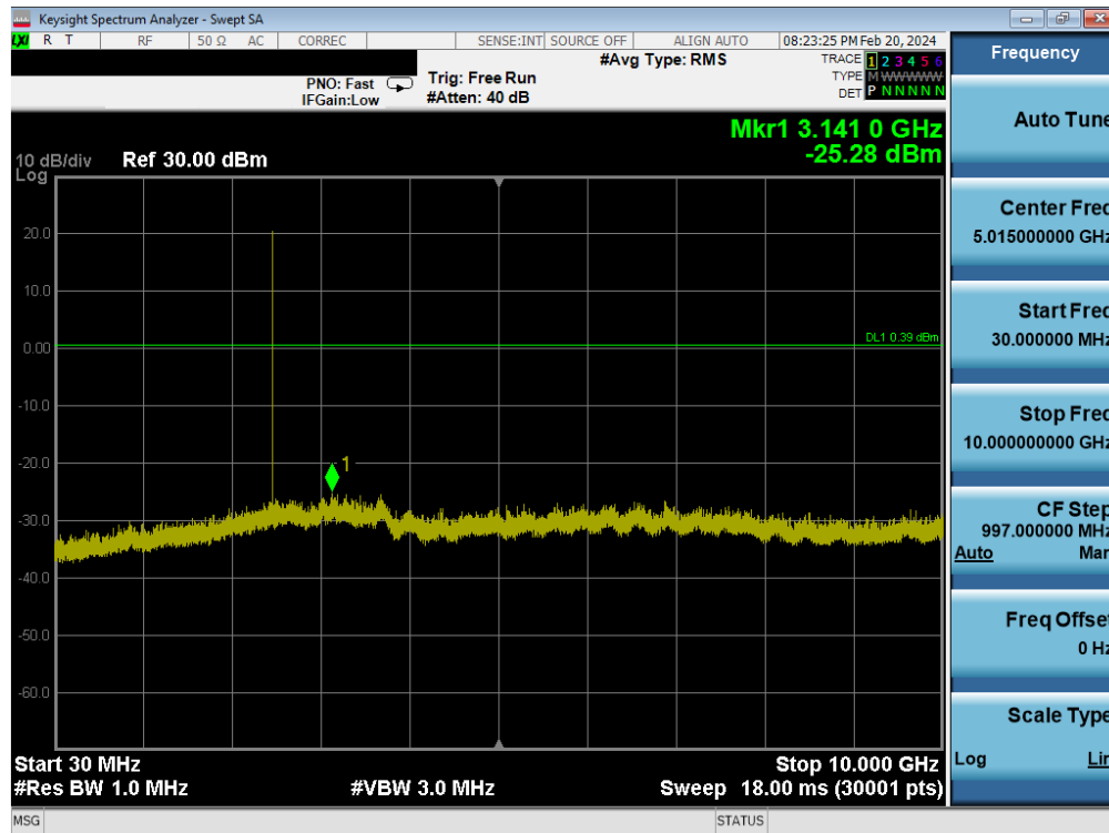
Plot 7-27. Conducted Spurious Antenna WF7b (802.15.4, ePA – Ch. 25)
