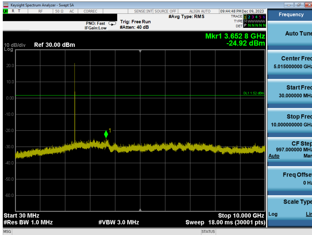
Plot 7-29. Conducted Spurious Antenna WF2b (802.15.4, ePA – Ch. 11)
