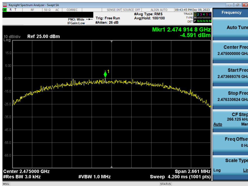
Plot 7-18. Power Spectral Density Antenna WF2b (802.15.4, iPA – Ch. 25)
