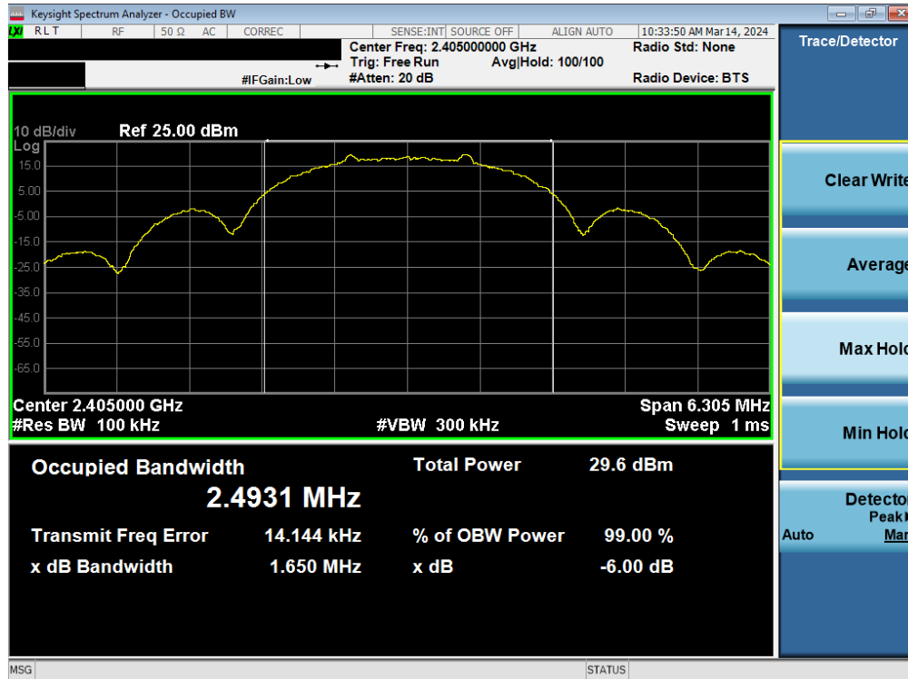
Plot 7-4. 6dB BW & 99% OBW Antenna WF2b (802.15.4, Ch. 11)
