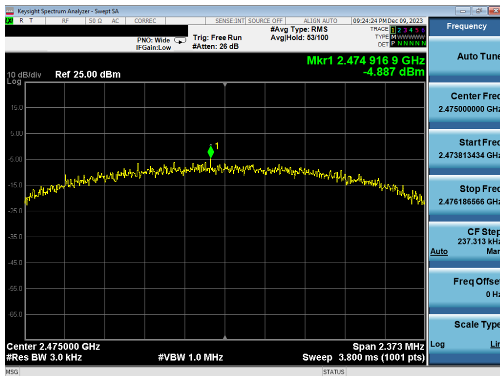
Plot 7-12. Power Spectral Density Antenna WF7b (802.15.4, iPA – Ch. 25)
