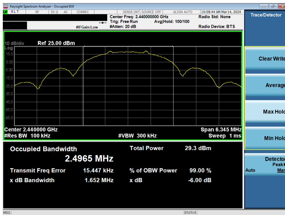
Plot 7-2. 6dB BW & 99% OBW Antenna WF7b (802.15.4, Ch. 18)
