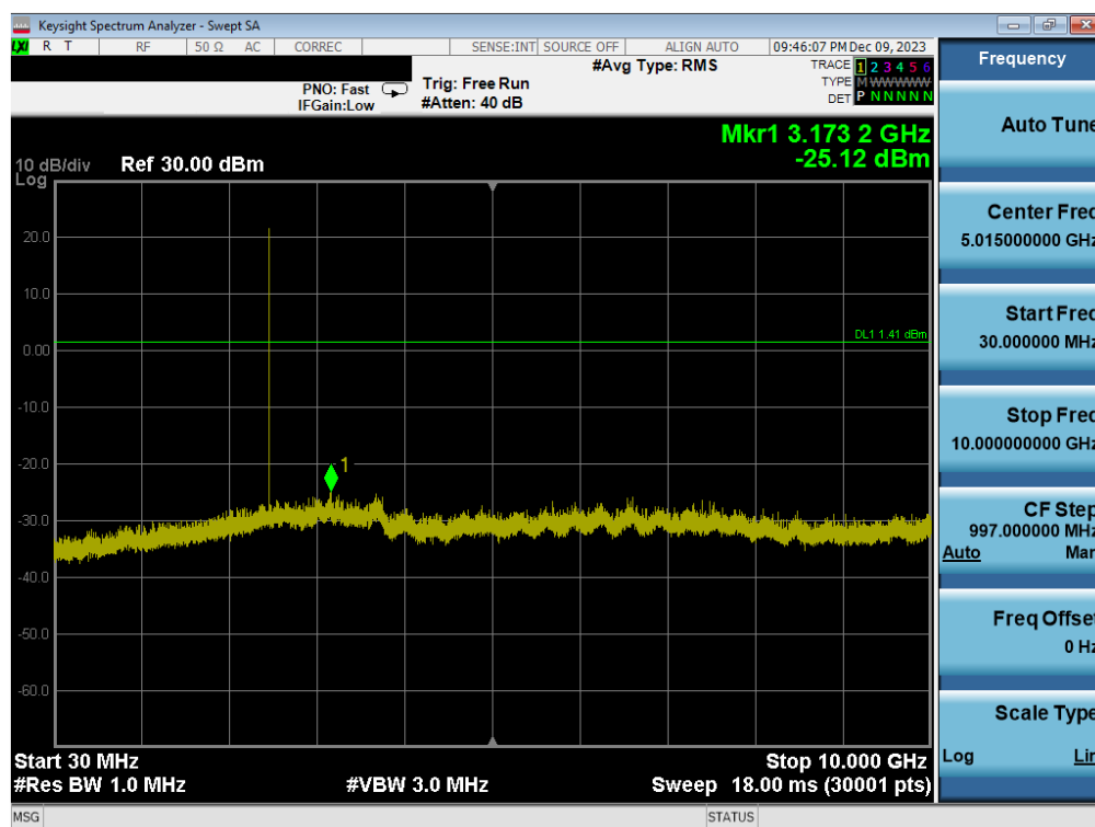
Plot 7-33. Conducted Spurious Antenna WF2b (802.15.4, ePA – Ch. 25)
