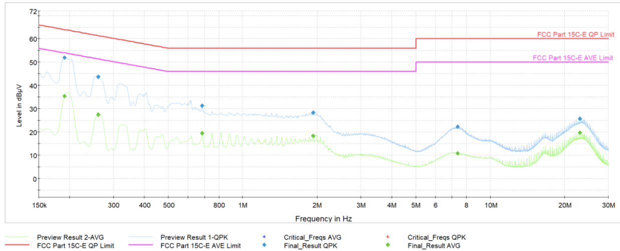
Plot 7-48. AC Line Conducted Emission with 802.15.4 (N, Ch.11, ePA with Laptop)
