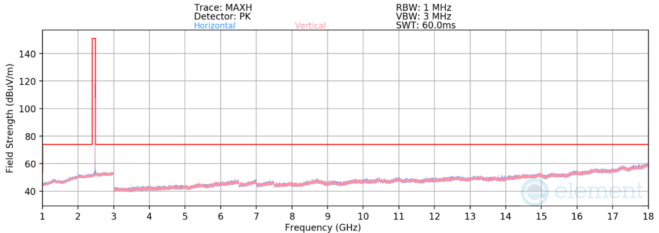
Plot 7-37. Radiated Spurious Emissions 1-18GHz Antenna WF7b (802.15.4, ePA – Ch. 25)
