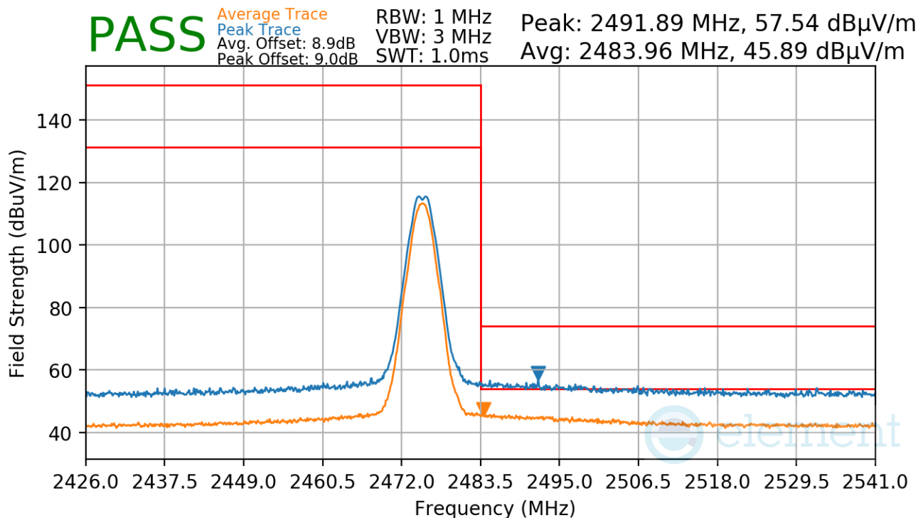
Plot 7-43. Radiated Restricted Upper Band Edge Measurement Antenna WF7b
