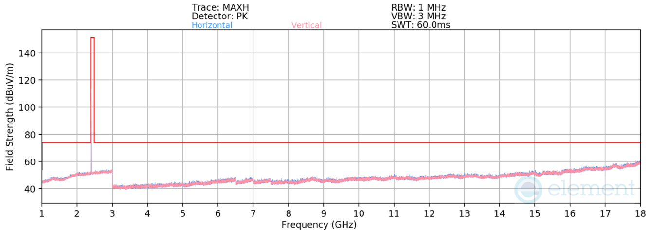
Plot 7-38. Radiated Spurious Emissions 1-18GHz Antenna WF2b (802.15.4, ePA – Ch. 11)
