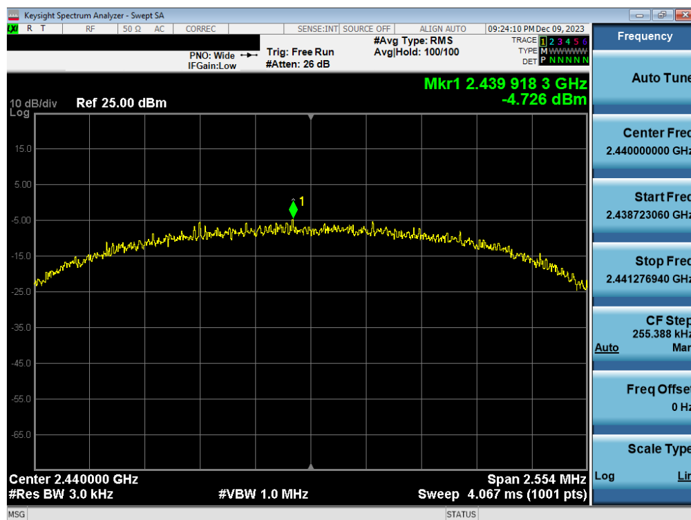
Plot 7-11. Power Spectral Density Antenna WF7b (802.15.4, iPA – Ch. 18)
