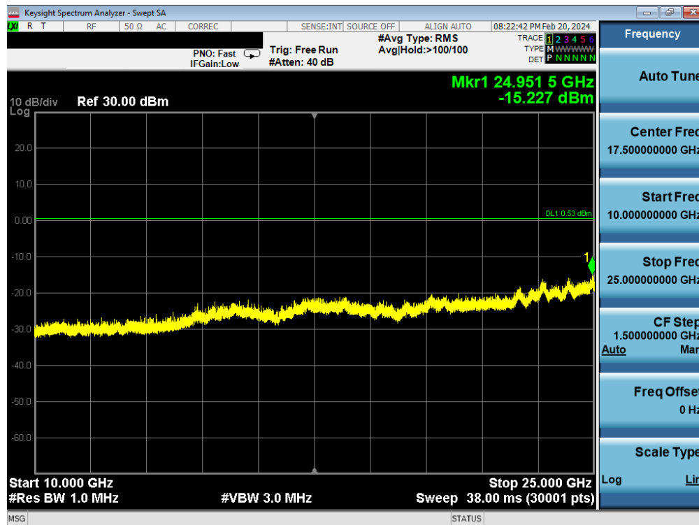
Plot 7-26. Conducted Spurious Antenna WF7b (802.15.4, ePA – Ch. 18)
