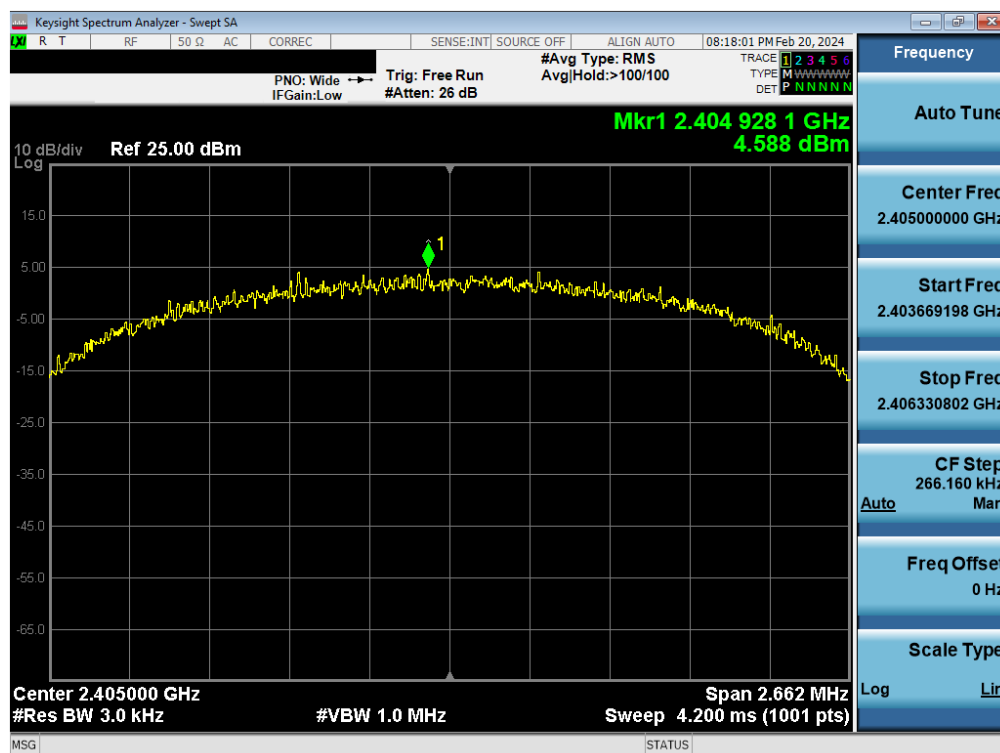
Plot 7-7. Power Spectral Density Antenna WF7b (802.15.4, ePA - Ch. 11)
