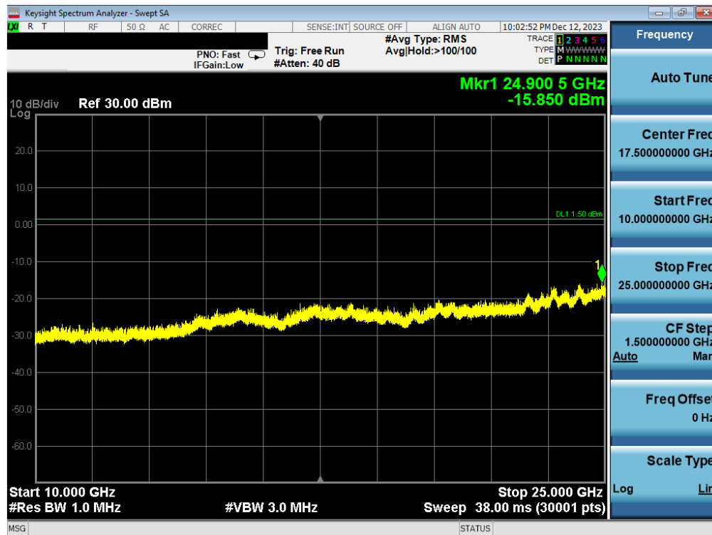
Plot 7-32. Conducted Spurious Antenna WF2b (802.15.4, ePA – Ch. 18)
