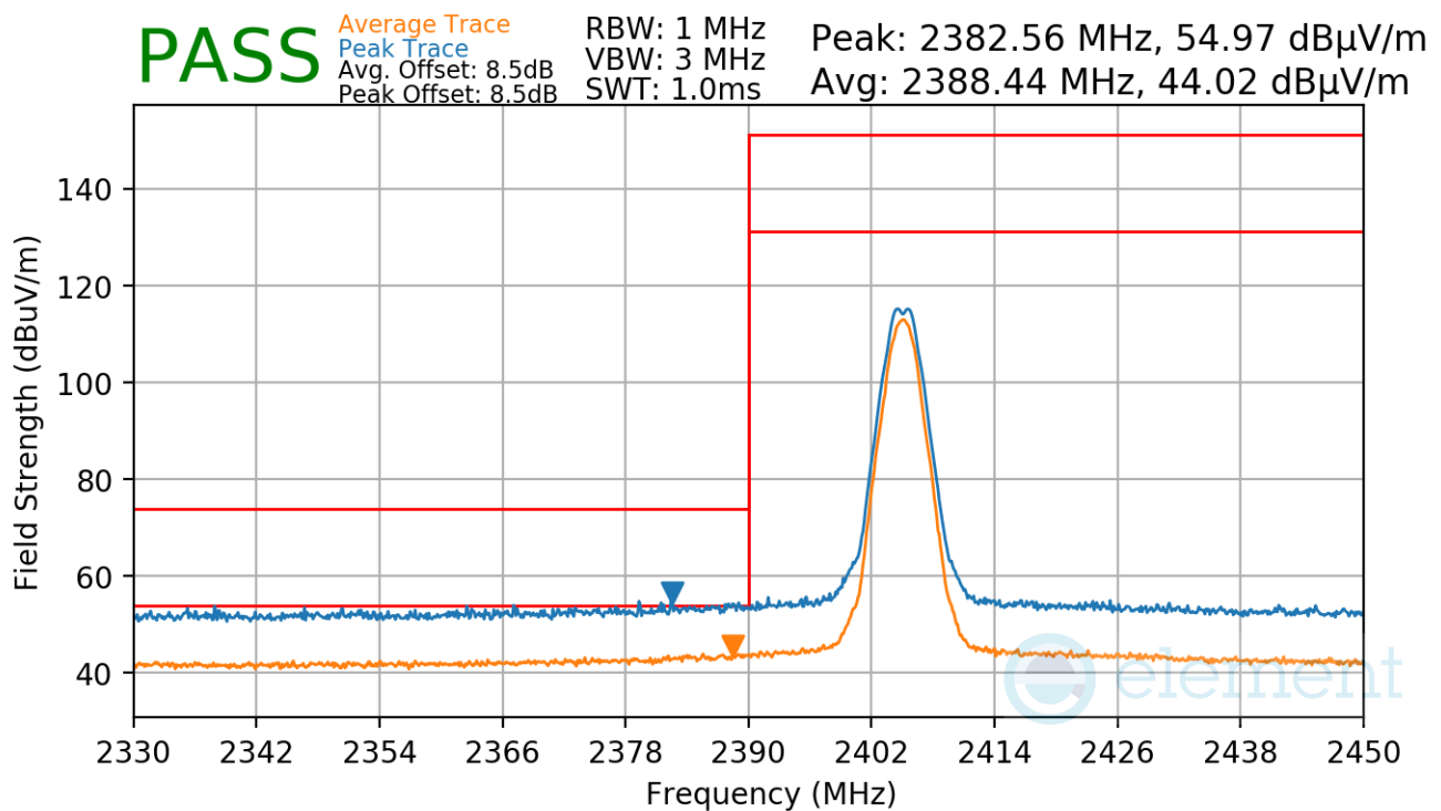
Plot 7-44. Radiated Restricted Lower Band Edge Measurement Antenna WF2b
