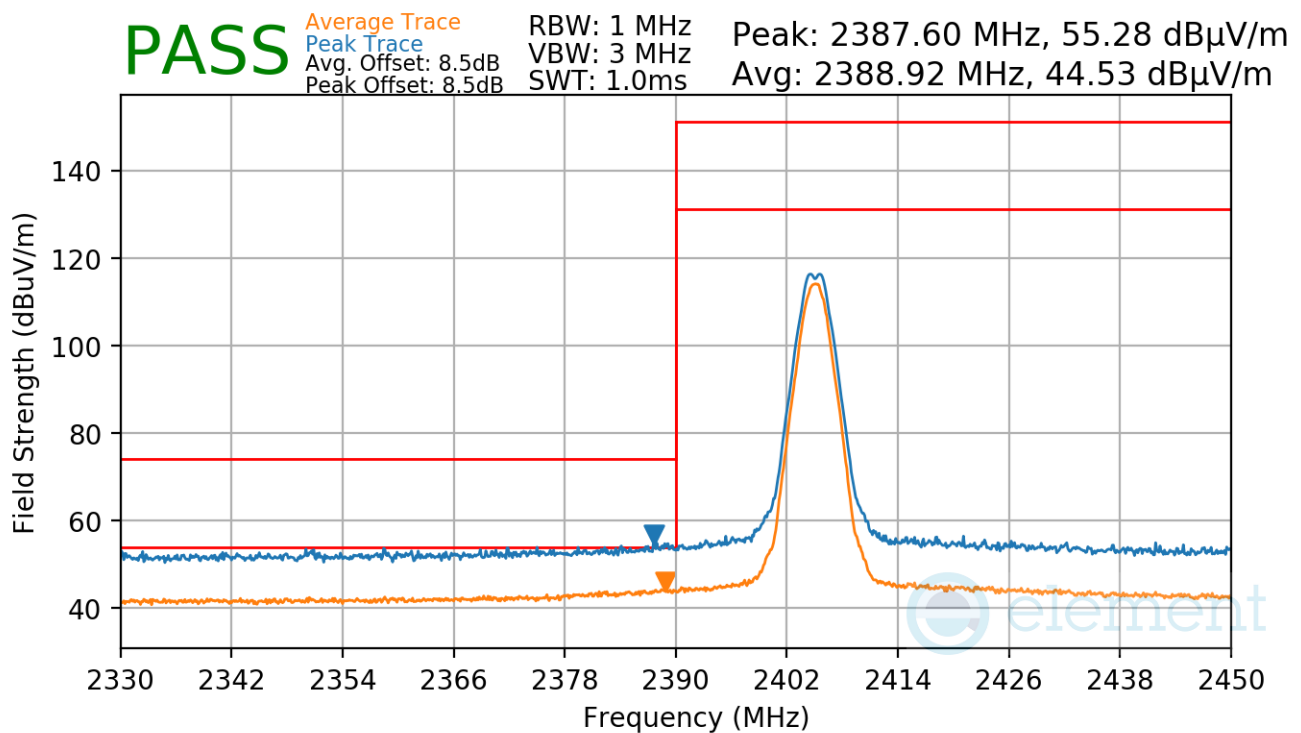
Plot 7-42. Radiated Restricted Lower Band Edge Measurement Antenna WF7b
