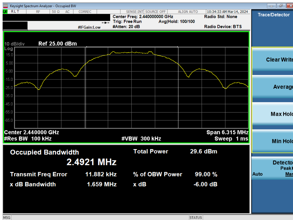
Plot 7-5. 6dB BW & 99% OBW Antenna WF2b (802.15.4, Ch. 18)
