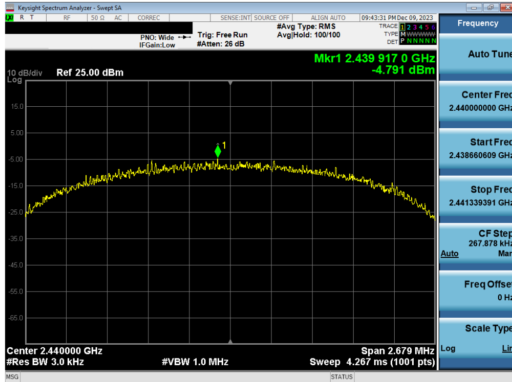
Plot 7-17. Power Spectral Density Antenna WF2b (802.15.4, iPA – Ch. 18)
