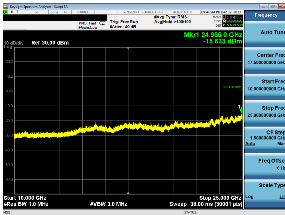
Plot 7-34. Conducted Spurious Antenna WF2b (802.15.4, ePA – Ch. 25)
