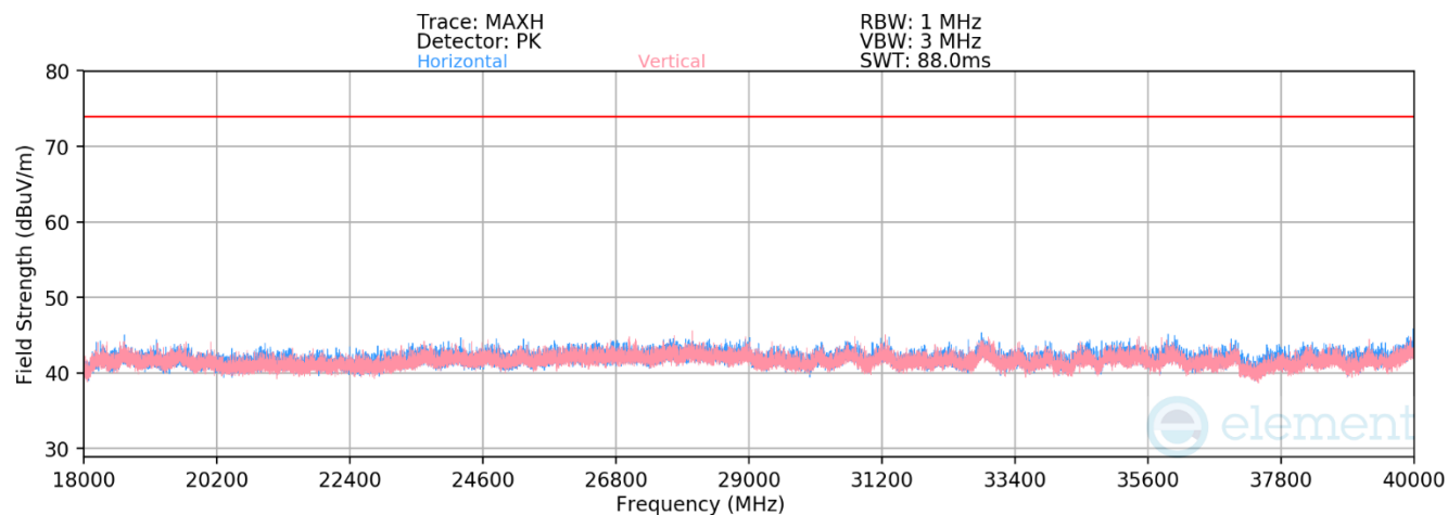
Plot 7-41. Radiated Spurious Emissions (802.15.4, ePA – Ch.11, Antenna WF2b)
