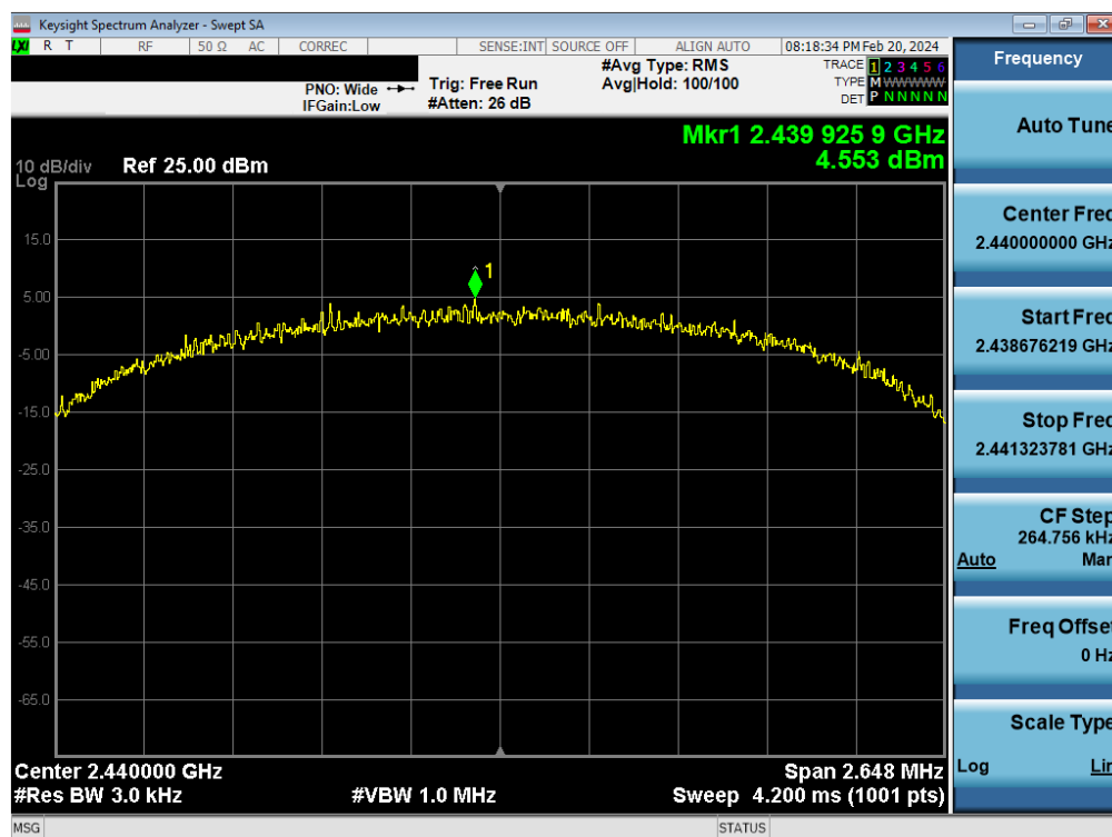
Plot 7-8. Power Spectral Density Antenna WF7b (802.15.4, ePA - Ch. 18)
