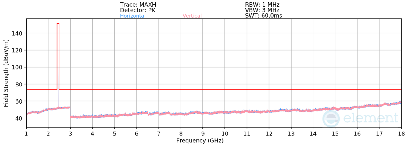
Plot 7-39. Radiated Spurious Emissions 1-18GHz Antenna WF2b (802.15.4, ePA – Ch. 18)
