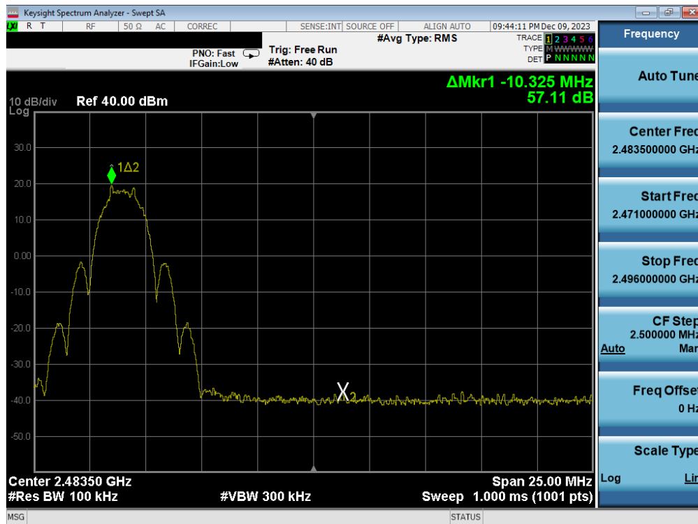
Plot 7-22. Band Edge Antenna WF2b (802.15.4, ePA – Ch. 25)
