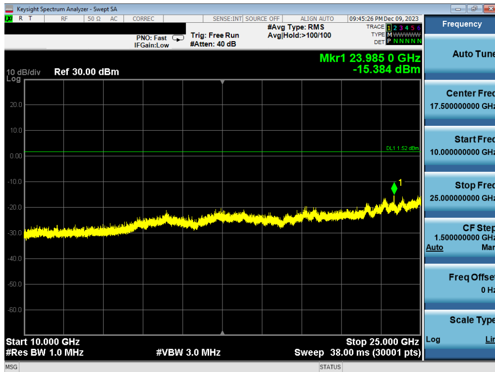
Plot 7-30. Conducted Spurious Antenna WF2b (802.15.4, ePA – Ch. 11)
