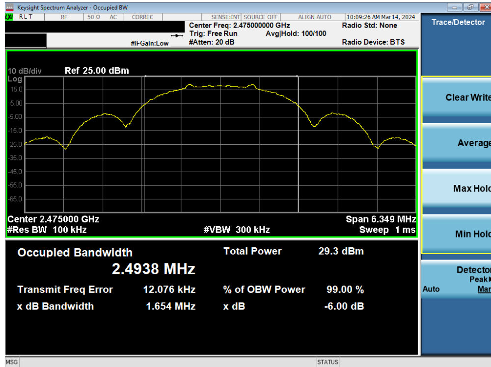
Plot 7-3. 6dB BW & 99% OBW Antenna WF7b (802.15.4, Ch. 25)
