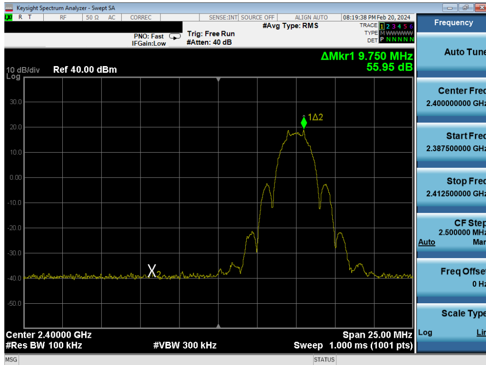
Plot 7-19. Band Edge Antenna WF7b (802.15.4, ePA – Ch. 11)
