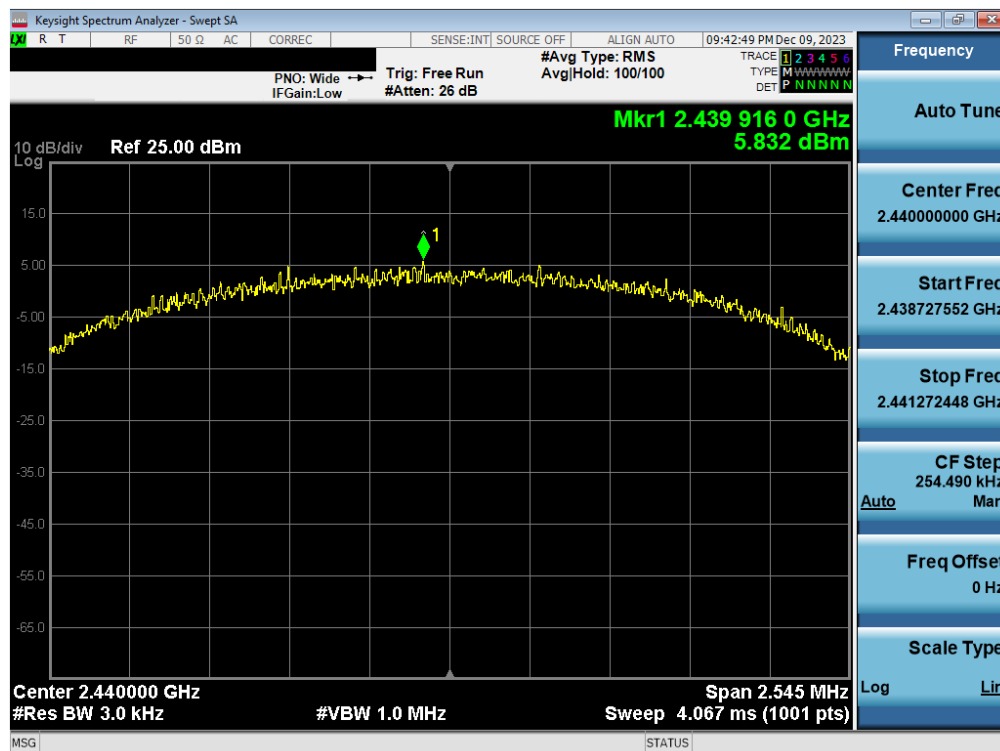
Plot 7-14. Power Spectral Density Antenna WF2b (802.15.4, ePA – Ch. 18)
