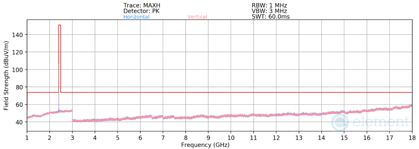
Plot 7-35. Radiated Spurious Emissions 1-18GHz Antenna WF7b (802.15.4, ePA – Ch. 11)
