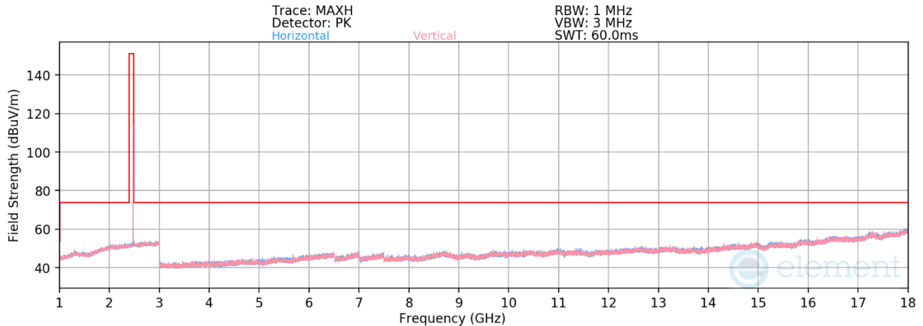
Plot 7-40. Radiated Spurious Emissions 1-18GHz Antenna WF2b (802.15.4, ePA – Ch. 25)
