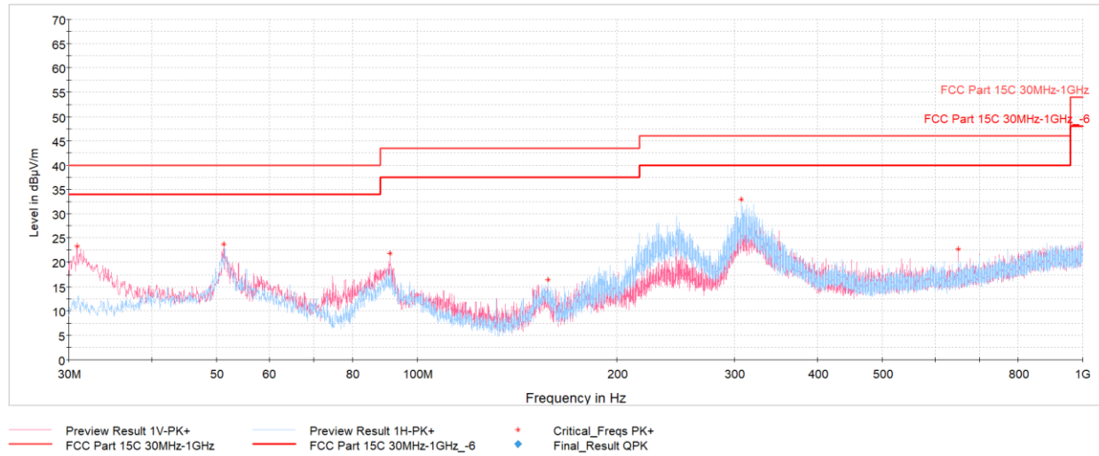
Plot 7-46. Radiated Spurious Emissions 30MHz-1GHz (Ch.11, ePA Antenna WF2b, with Laptop)
