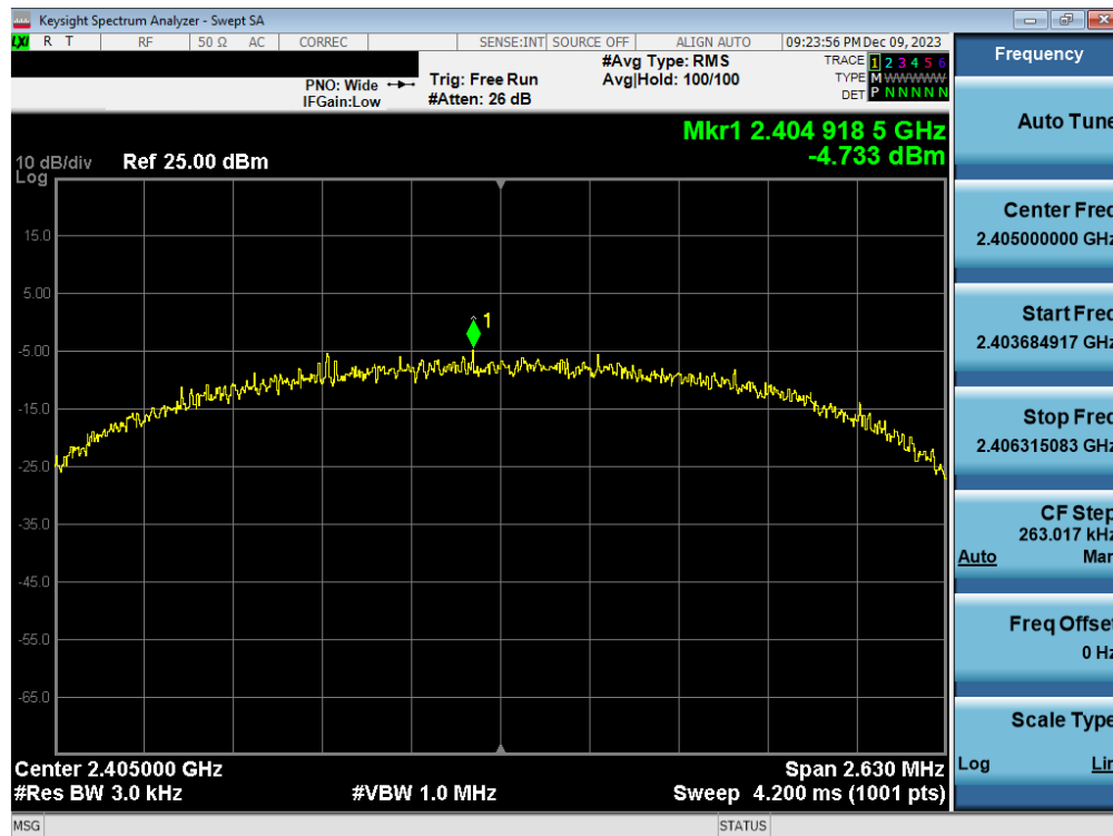
Plot 7-10. Power Spectral Density Antenna WF7b (802.15.4, iPA – Ch. 11)
