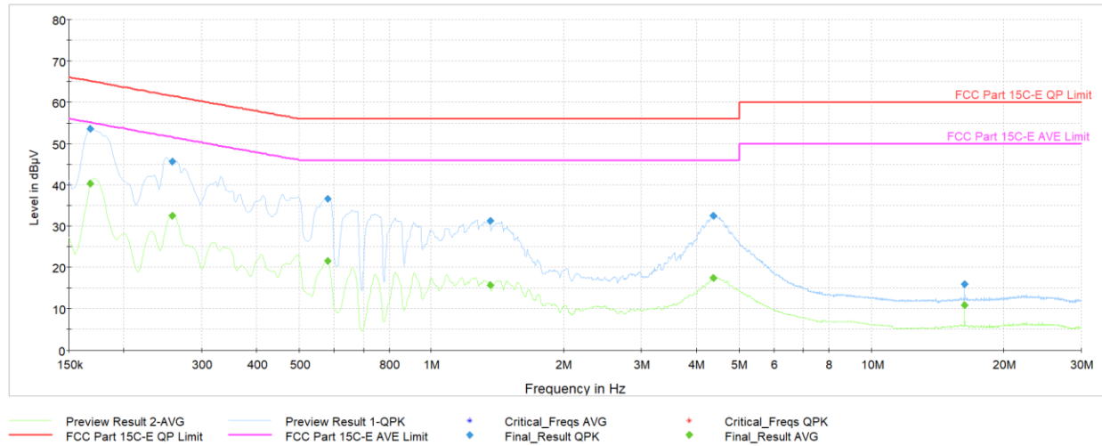
Plot 7-47. AC Line Conducted Emission with 802.15.4 (L1, Ch.11, ePA with Laptop)
