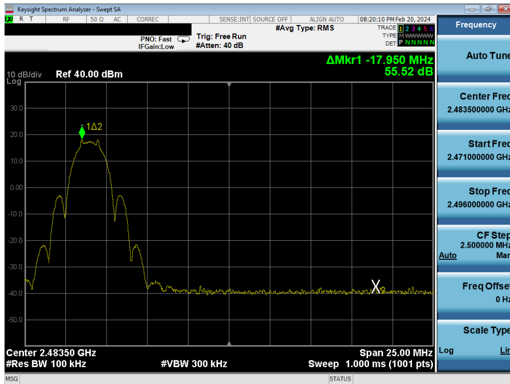
Plot 7-20. Band Edge Antenna WF7b (802.15.4, ePA – Ch. 25)
