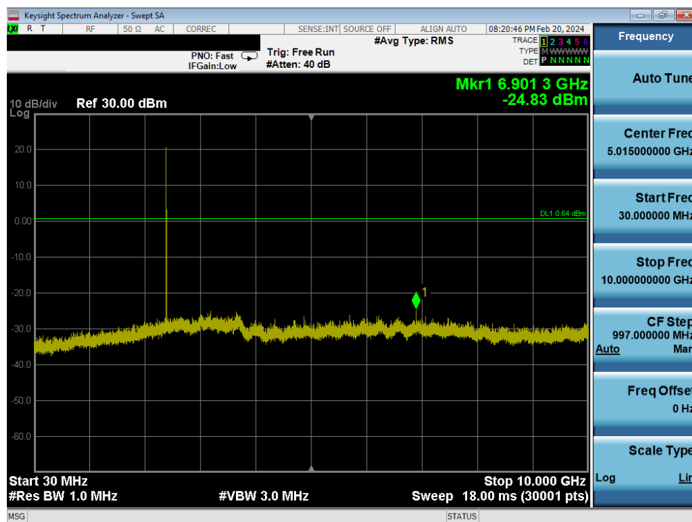
Plot 7-23. Conducted Spurious Antenna WF7b (802.15.4, ePA – Ch. 11)
