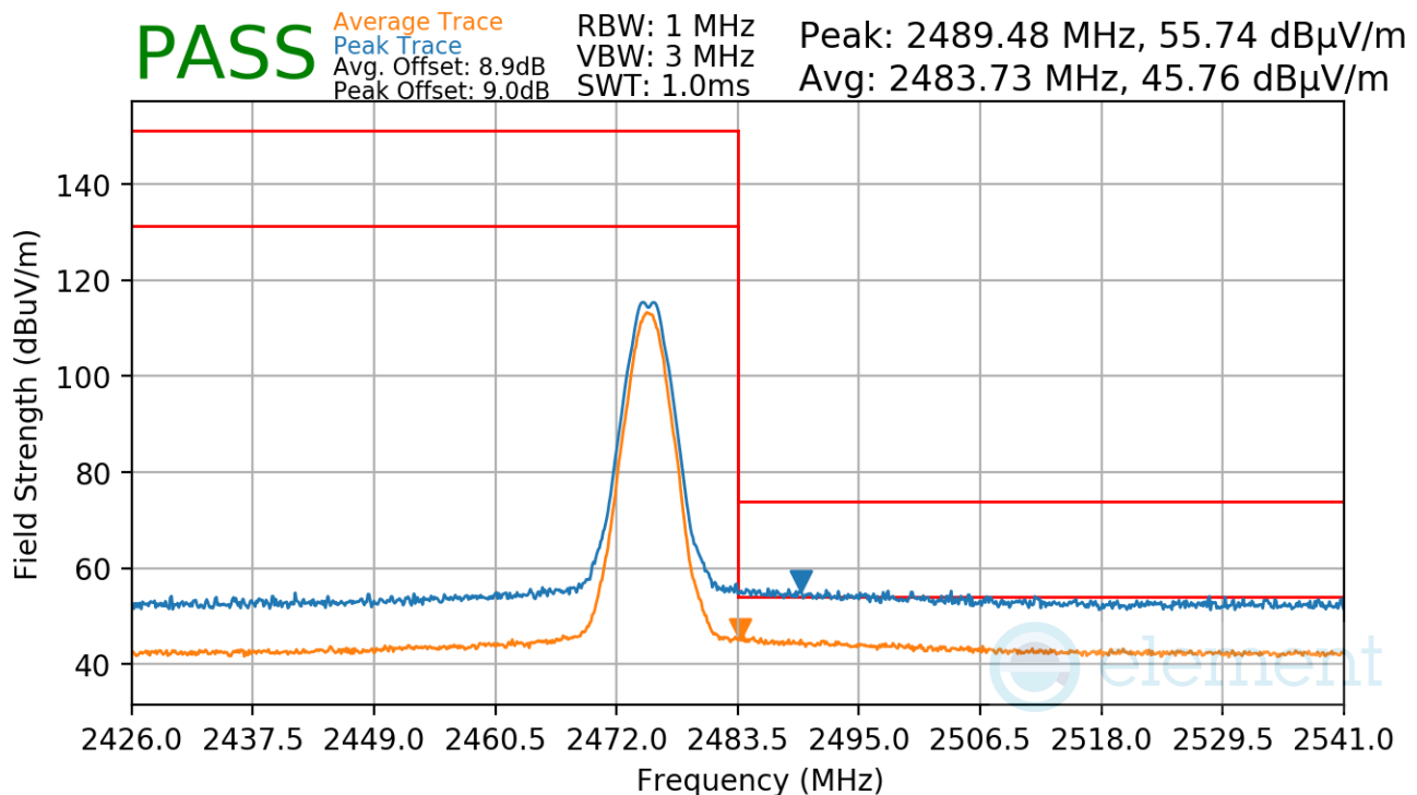
Plot 7-45. Radiated Restricted Upper Band Edge Measurement Antenna WF2b
