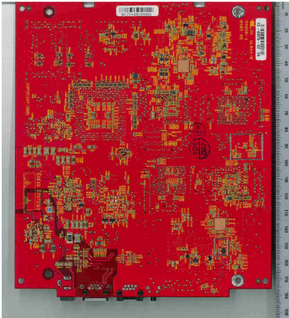
Photograph No.2 PCB second side view without shields
