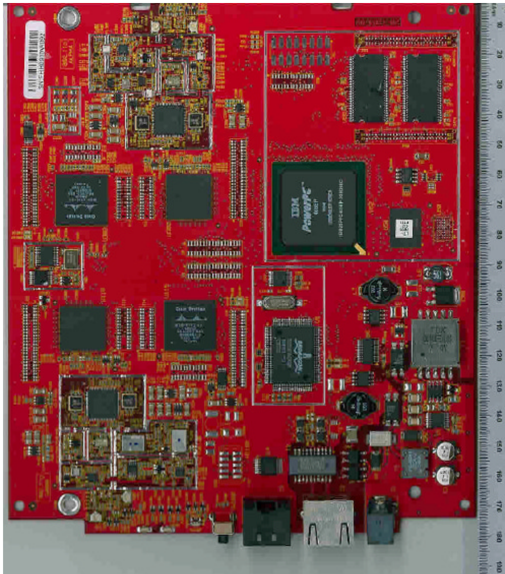
Photograph No.1 PCB top view without shields
