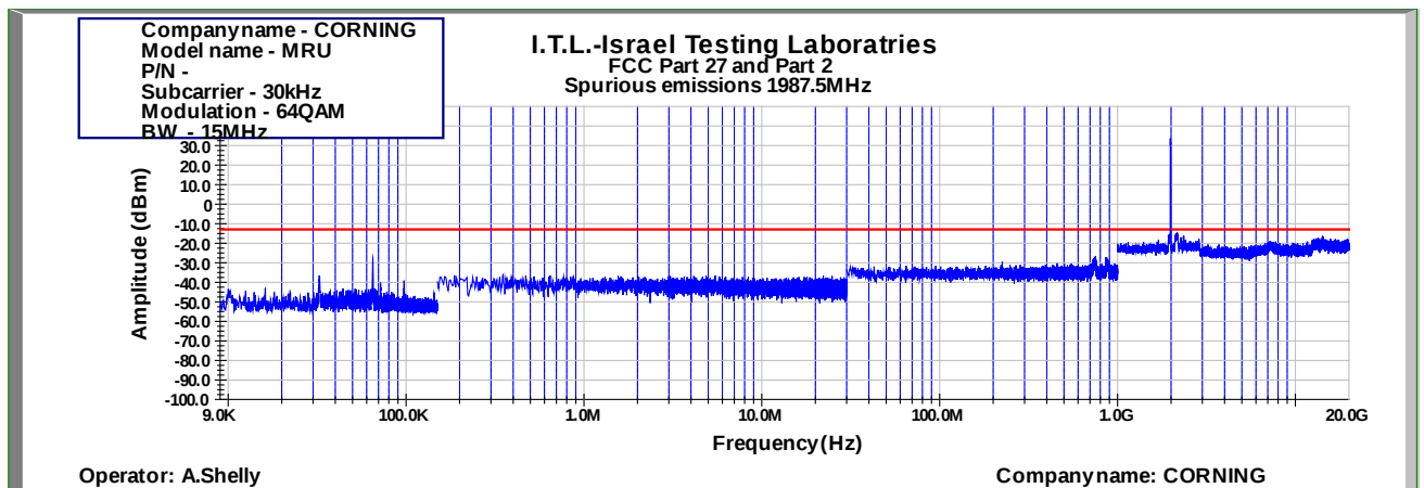
Figure 889: Spurious Emissions at Antenna Terminal 64QAM 15MHz B.W.; 1987.5MHz, 30kHz
