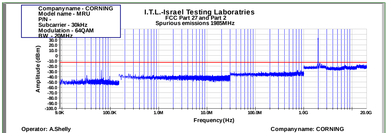
Figure 898: Spurious Emissions at Antenna Terminal 64QAM 20MHz B.W.; 1985.0MHz, 30kHz
