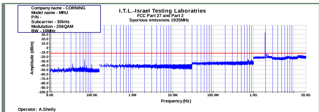
Figure 940: Spurious Emissions at Antenna Terminal 256QAM 10MHz B.W.; 1935.00MHz, 30kHz
