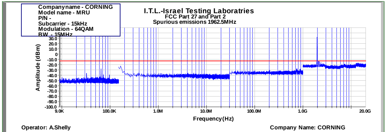
Figure 885: Spurious Emissions at Antenna Terminal 64QAM 15MHz B.W.; 1962.5MHz, 15kHz
