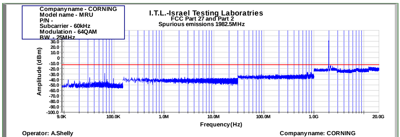
Figure 908: Spurious Emissions at Antenna Terminal 64QAM 25MHz B.W.; 1982.5MHz, 60kHz
