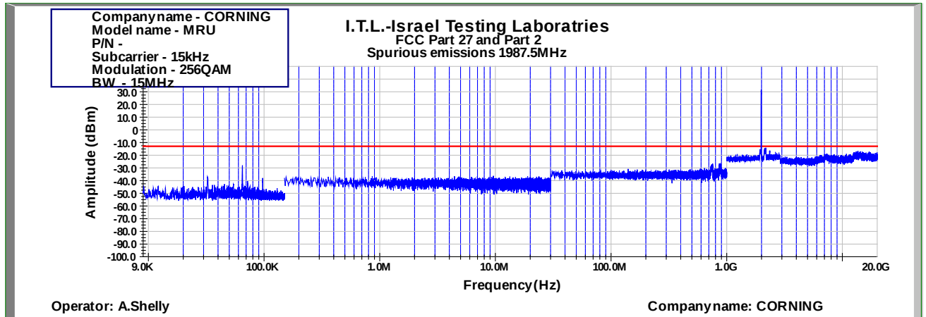
Figure 954: Spurious Emissions at Antenna Terminal 256QAM 15MHz B.W.; 1987.5MHz, 15kHz
