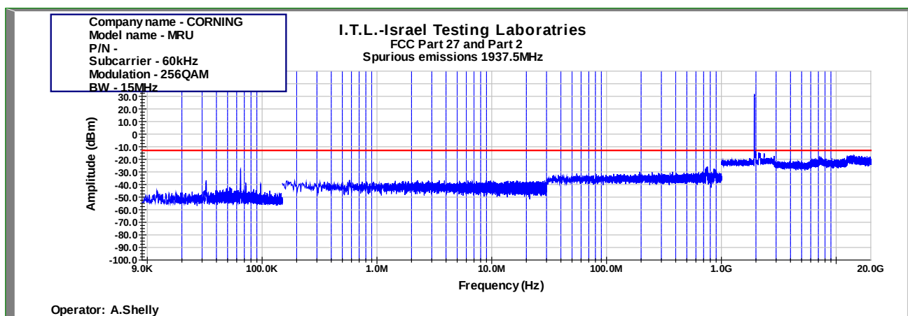
Figure 950: Spurious Emissions at Antenna Terminal 256QAM 15MHz B.W.; 1937.5MHz, 60kHz
