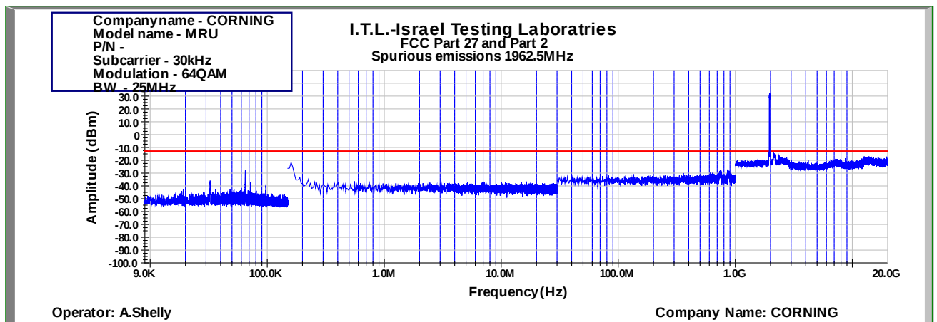
Figure 904: Spurious Emissions at Antenna Terminal 64QAM 25MHz B.W.; 1962.5MHz, 30kHz
