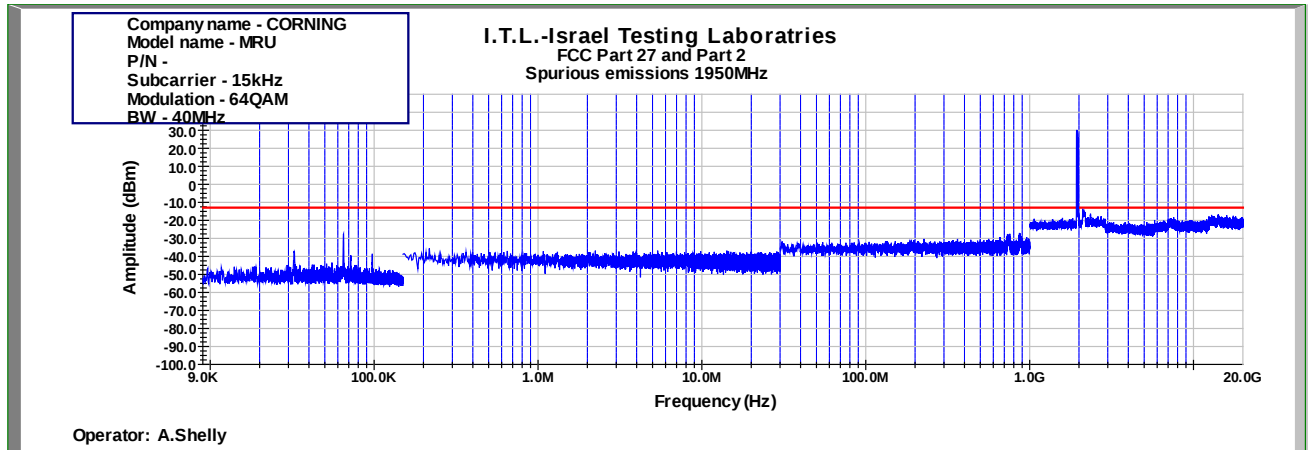
Figure 909: Spurious Emissions at Antenna Terminal 64QAM 40MHz B.W.; 1950.0MHz, 15kHz
