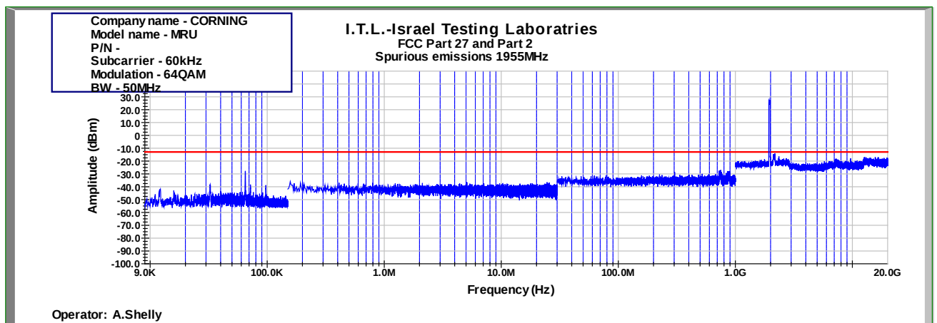
Figure 920: Spurious Emissions at Antenna Terminal 64QAM 50MHz B.W.; 1955.0MHz, 60kHz
