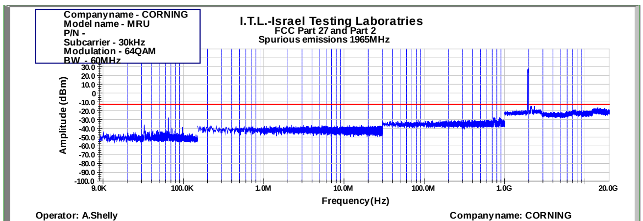
Figure 931: Spurious Emissions at Antenna Terminal 64QAM 60MHz B.W.; 1965.0MHz, 30kHz
