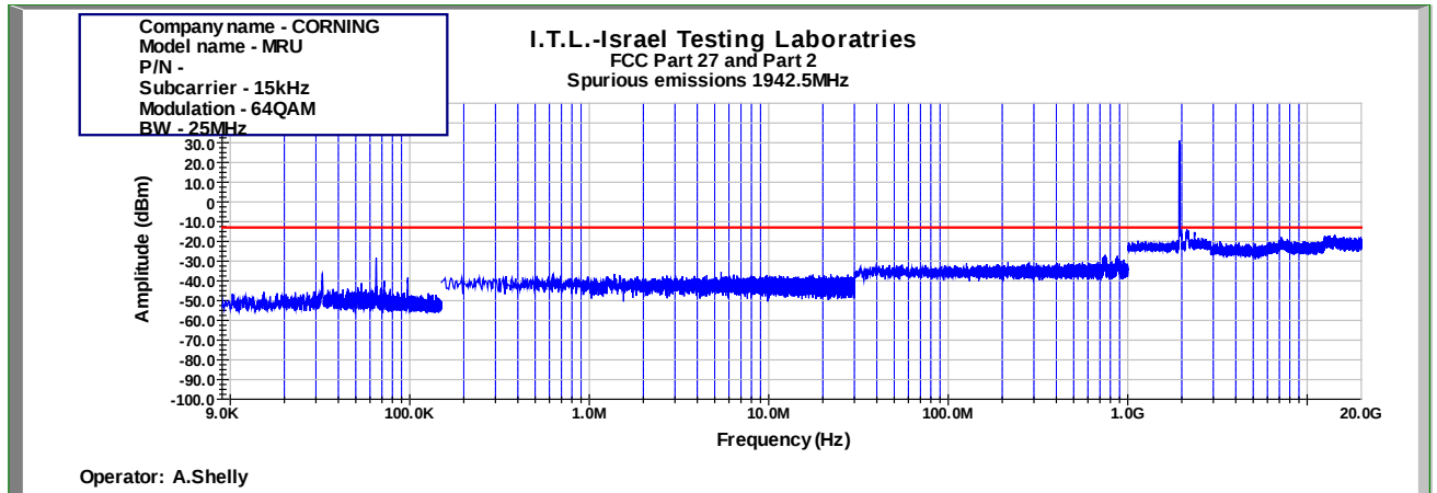
Figure 900: Spurious Emissions at Antenna Terminal 64QAM 25MHz B.W.; 1942.5MHz, 15kHz
