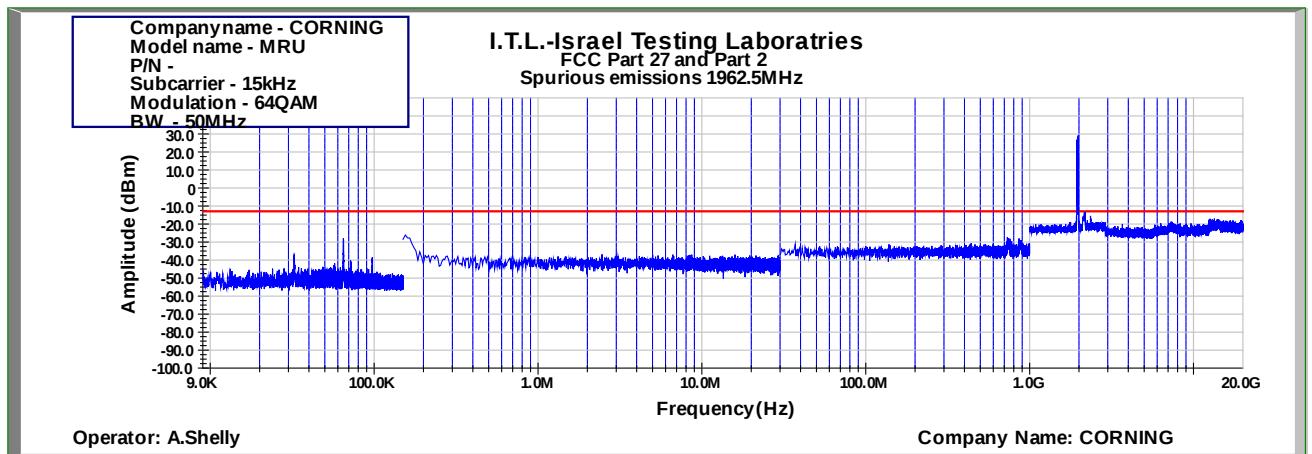
Figure 921: Spurious Emissions at Antenna Terminal 64QAM 50MHz B.W.; 1962.5MHz, 15kHz
