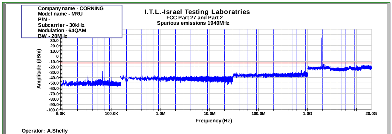
Figure 892: Spurious Emissions at Antenna Terminal 64QAM 20MHz B.W.; 1940.0MHz, 30kHz
