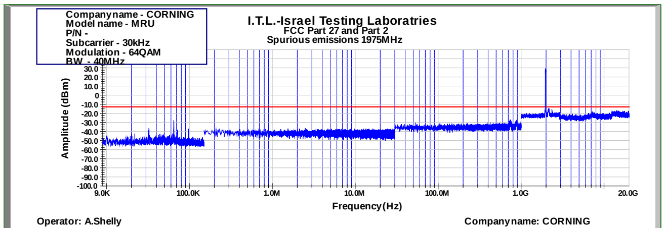
Figure 916: Spurious Emissions at Antenna Terminal 64QAM 40MHz B.W.; 1975.0MHz, 30kHz
