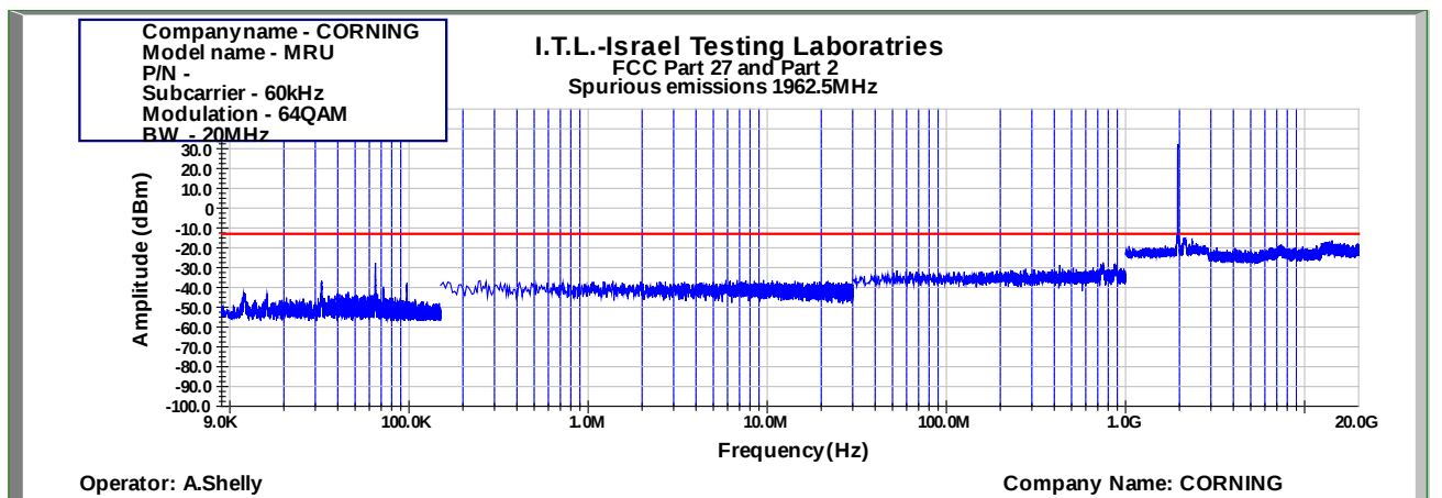
Figure 896: Spurious Emissions at Antenna Terminal 64QAM 20MHz B.W.; 1962.5MHz, 60kHz
