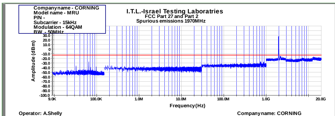
Figure 924: Spurious Emissions at Antenna Terminal 64QAM 50MHz B.W.; 1970.0MHz, 15kHz
