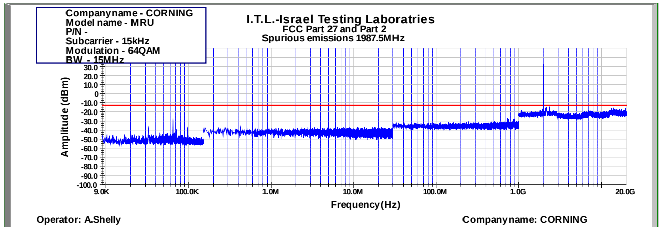
Figure 888: Spurious Emissions at Antenna Terminal 64QAM 15MHz B.W.; 1987.5MHz, 15kHz
