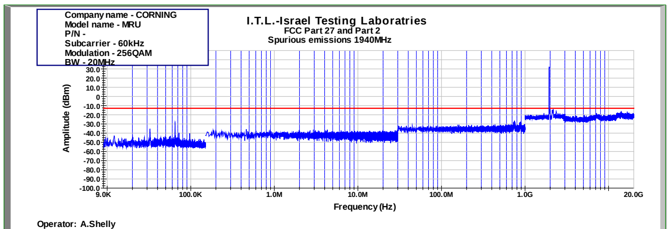
Figure 959: Spurious Emissions at Antenna Terminal 256QAM 20MHz B.W.; 1940.0MHz, 60kHz
