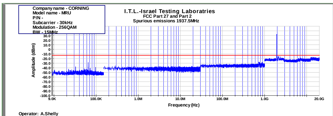
Figure 949: Spurious Emissions at Antenna Terminal 256QAM 15MHz B.W.; 1937.5MHz, 30kHz
