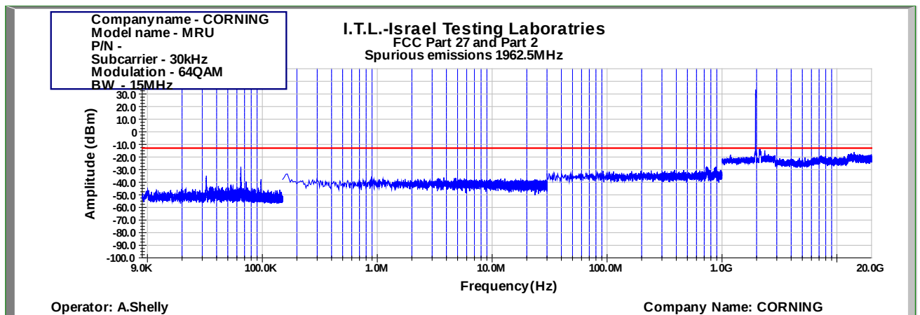
Figure 886: Spurious Emissions at Antenna Terminal 64QAM 15MHz B.W.; 1962.5MHz, 30kHz
