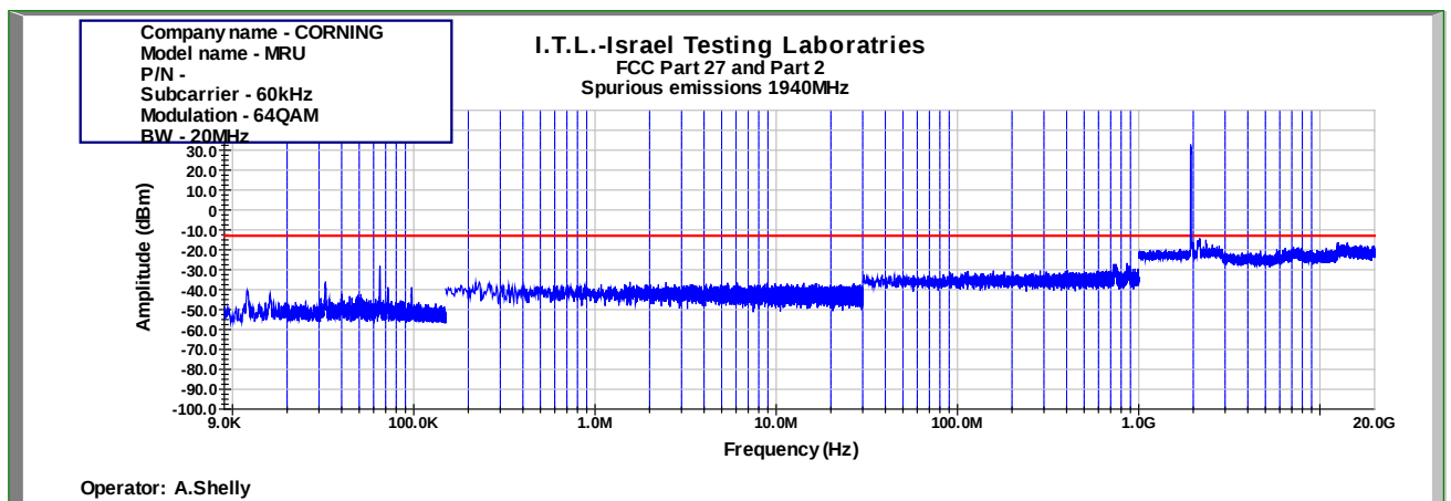
Figure 893: Spurious Emissions at Antenna Terminal 64QAM 20MHz B.W.; 1940.0MHz, 60kHz
