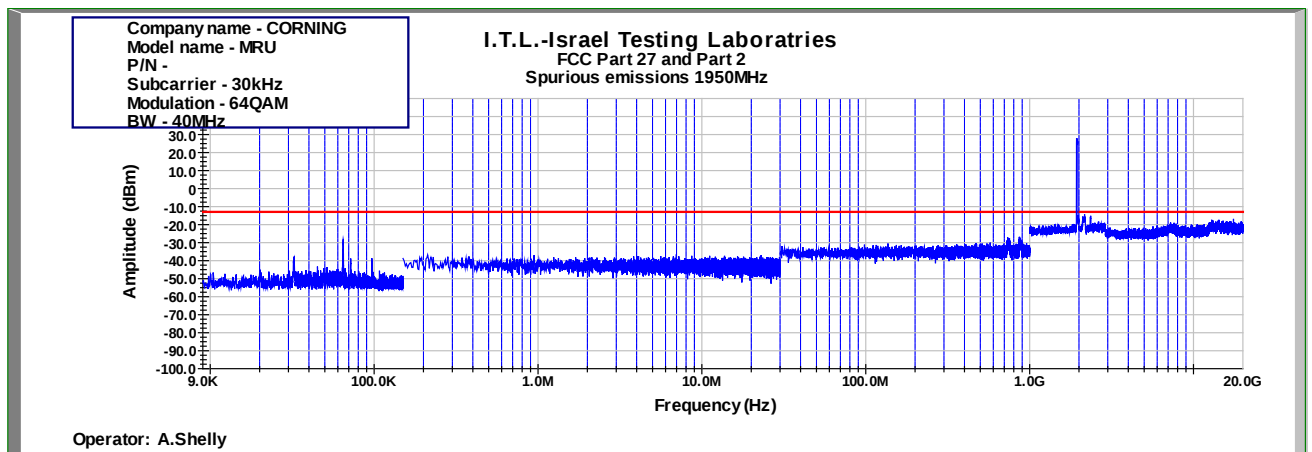
Figure 910: Spurious Emissions at Antenna Terminal 64QAM 40MHz B.W.; 1950.0MHz, 30kHz
