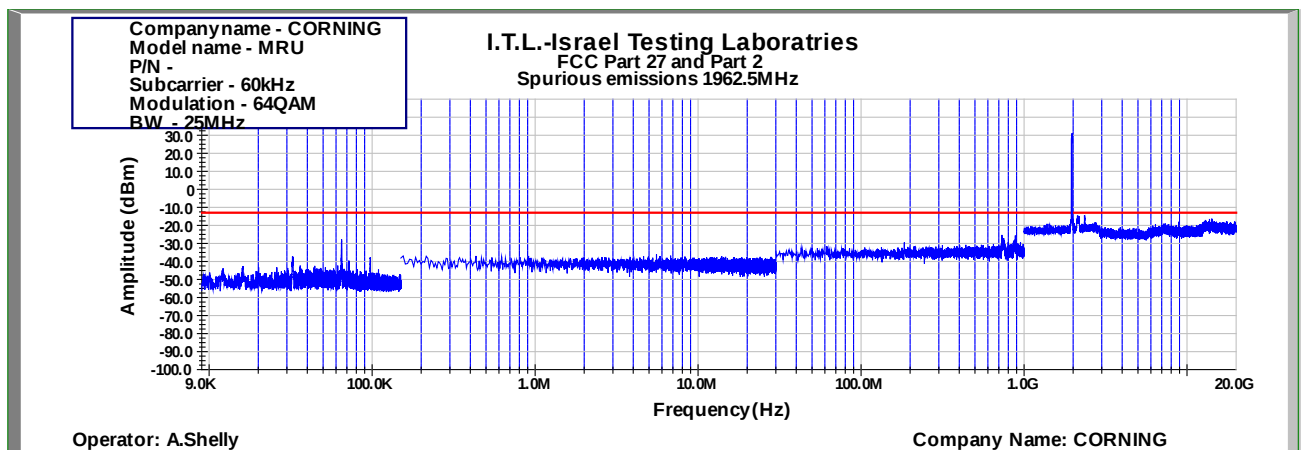
Figure 905: Spurious Emissions at Antenna Terminal 64QAM 25MHz B.W.; 1962.5MHz, 60kHz
