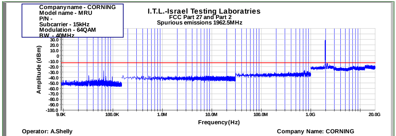
Figure 912: Spurious Emissions at Antenna Terminal 64QAM 40MHz B.W.; 1962.5MHz, 15kHz
