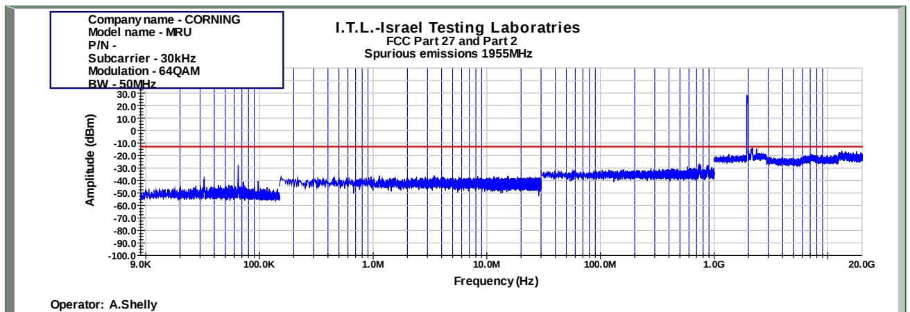
Figure 919: Spurious Emissions at Antenna Terminal 64QAM 50MHz B.W.; 1955.0MHz, 30kHz
