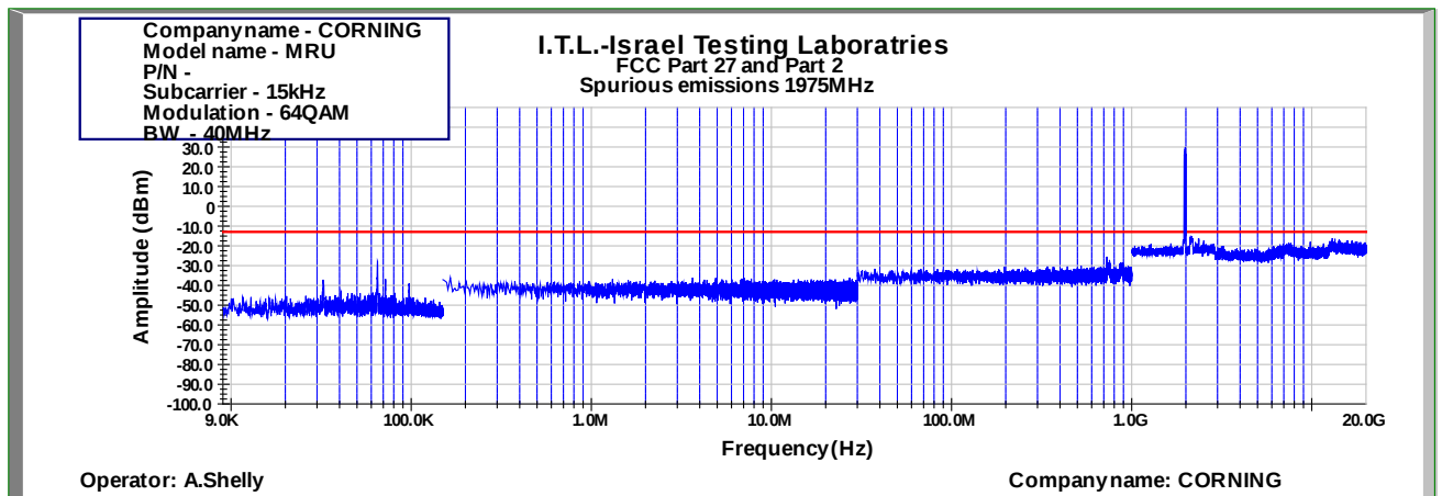
Figure 915: Spurious Emissions at Antenna Terminal 64QAM 40MHz B.W.; 1975.0MHz, 15kHz
