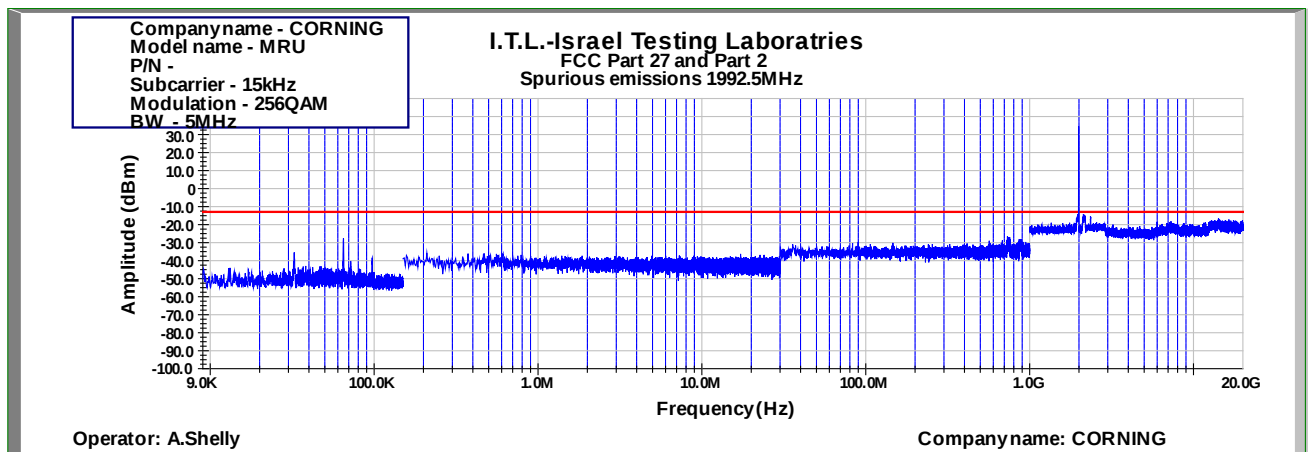
Figure 937: Spurious Emissions at Antenna Terminal 256QAM 5MHz B.W.; 1992.5MHz, 15kHz
