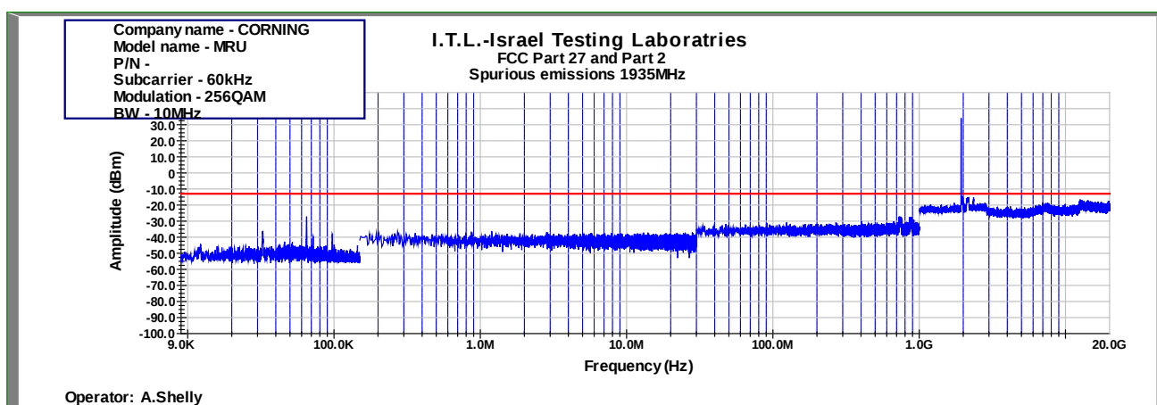
Figure 941: Spurious Emissions at Antenna Terminal 256QAM 10MHz B.W.; 1935.00MHz, 60kHz
