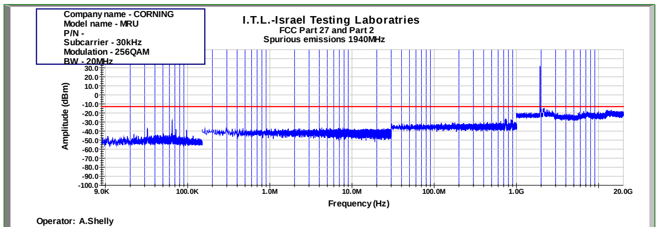
Figure 958: Spurious Emissions at Antenna Terminal 256QAM 20MHz B.W.; 1940.0MHz, 30kHz
