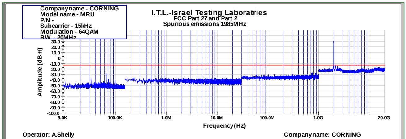
Figure 897: Spurious Emissions at Antenna Terminal 64QAM 20MHz B.W.; 1985.0MHz, 15kHz
