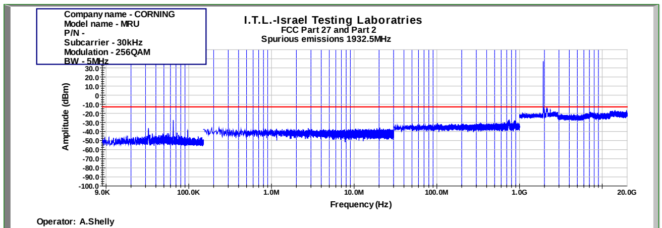
Figure 934: Spurious Emissions at Antenna Terminal 256QAM 5MHz B.W.; 1932.5MHz, 30kHz
