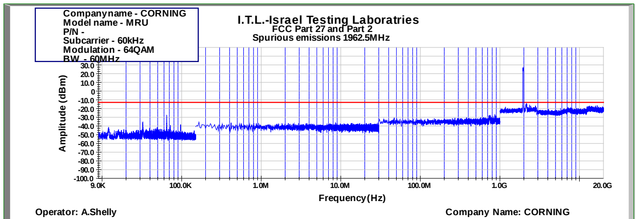
Figure 930: Spurious Emissions at Antenna Terminal 64QAM 60MHz B.W.; 1962.5MHz, 60kHz
