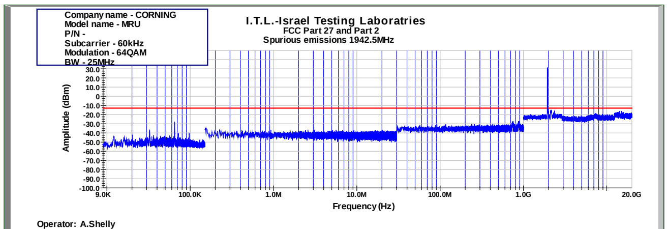
Figure 902: Spurious Emissions at Antenna Terminal 64QAM 25MHz B.W.; 1942.5MHz, 60kHz
