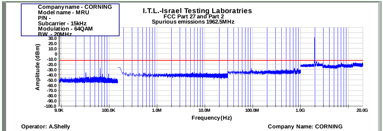
Figure 894: Spurious Emissions at Antenna Terminal 64QAM 20MHz B.W.; 1962.5MHz, 15kHz
