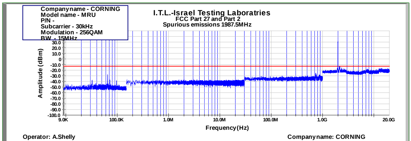
Figure 955: Spurious Emissions at Antenna Terminal 256QAM 15MHz B.W.; 1987.5MHz, 30kHz
