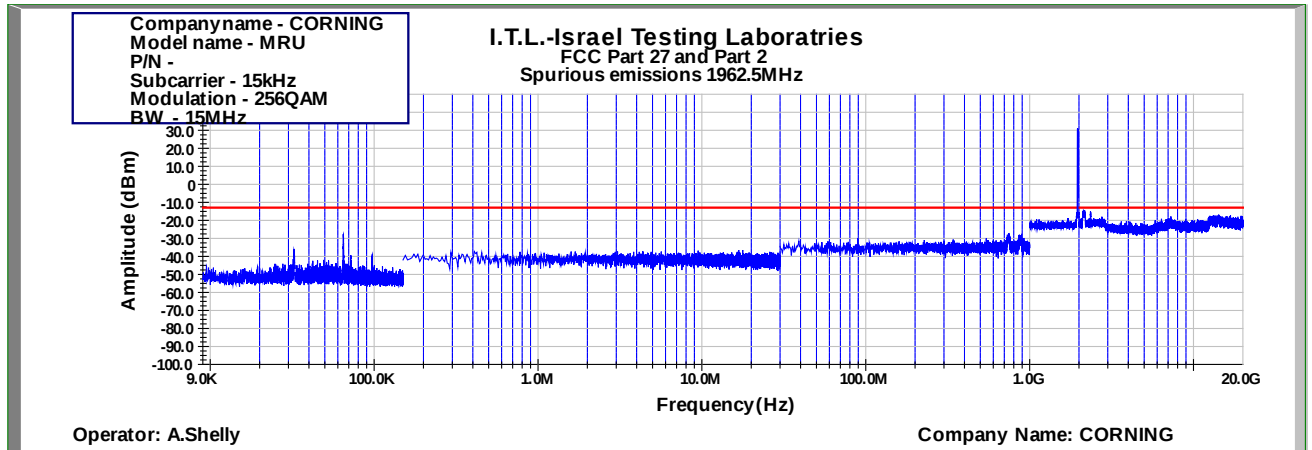
Figure 951: Spurious Emissions at Antenna Terminal 256QAM 15MHz B.W.; 1962.5MHz, 15kHz
