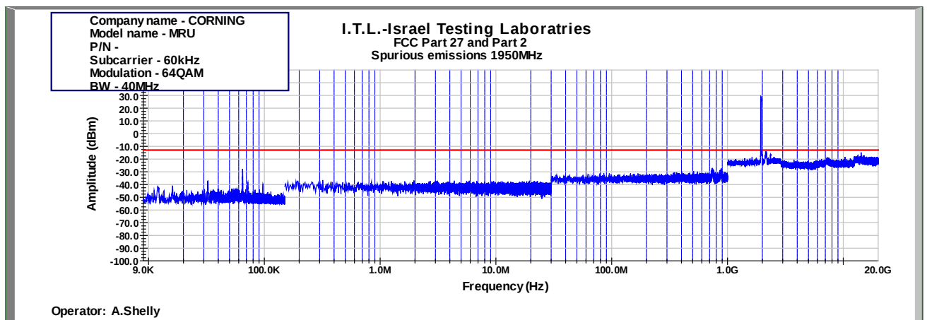
Figure 911: Spurious Emissions at Antenna Terminal 64QAM 40MHz B.W.; 1950.0MHz, 60kHz
