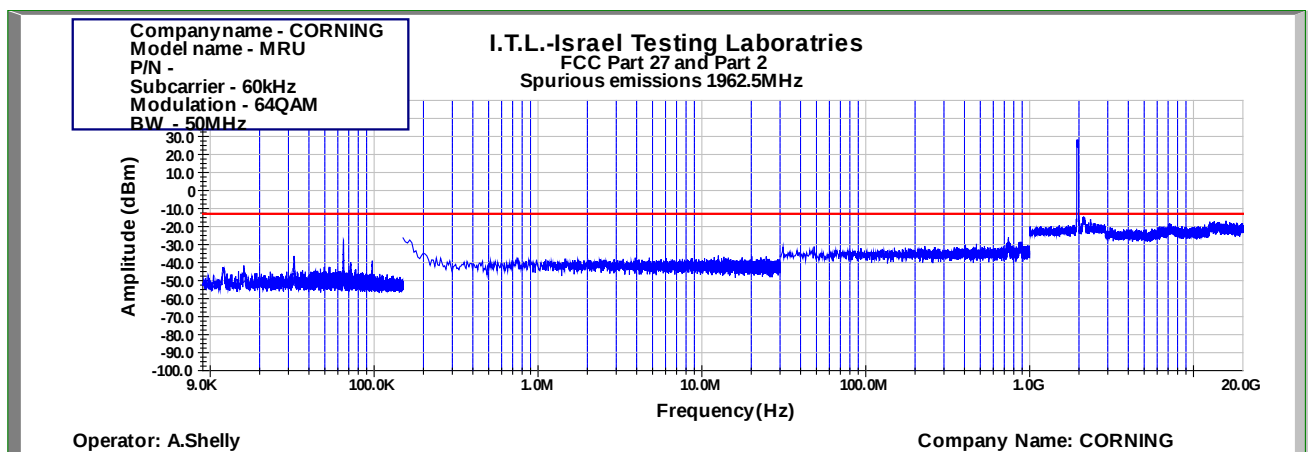
Figure 923: Spurious Emissions at Antenna Terminal 64QAM 50MHz B.W.; 1962.5MHz, 60kHz
