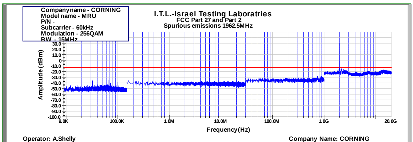
Figure 953: Spurious Emissions at Antenna Terminal 256QAM 15MHz B.W.; 1962.5MHz, 60kHz
