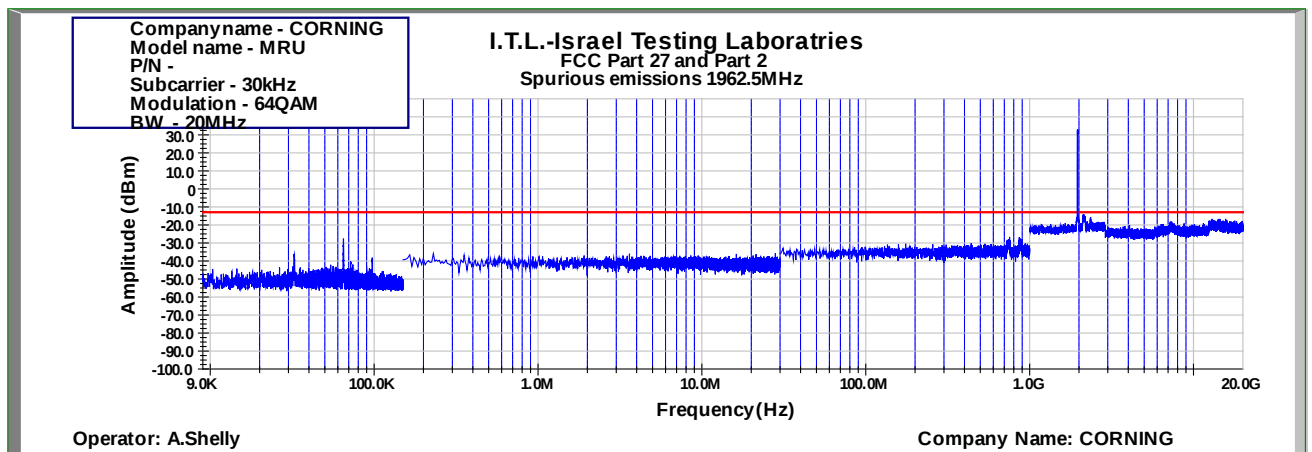
Figure 895: Spurious Emissions at Antenna Terminal 64QAM 20MHz B.W.; 1962.5MHz, 30kHz
