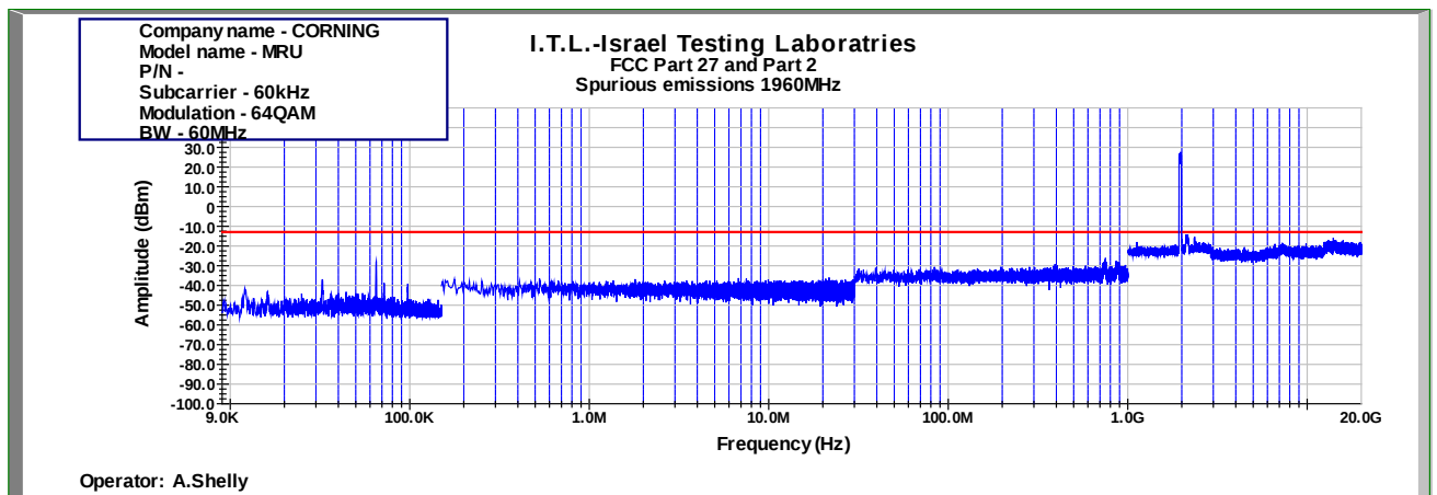
Figure 928: Spurious Emissions at Antenna Terminal 64QAM 60MHz B.W.; 1960.0MHz, 60kHz
