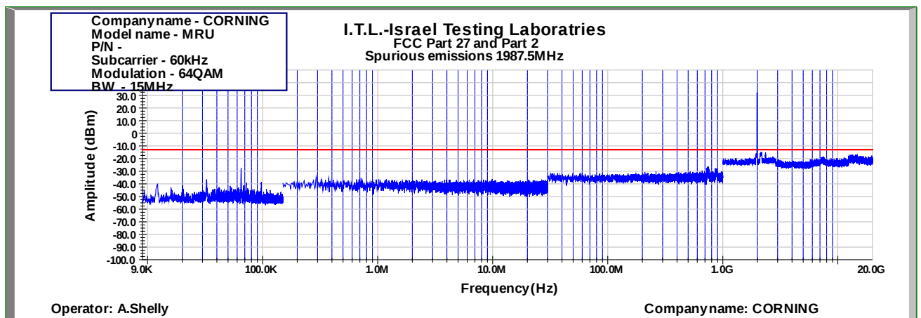
Figure 890: Spurious Emissions at Antenna Terminal 64QAM 15MHz B.W.; 1987.5MHz, 60kHz
