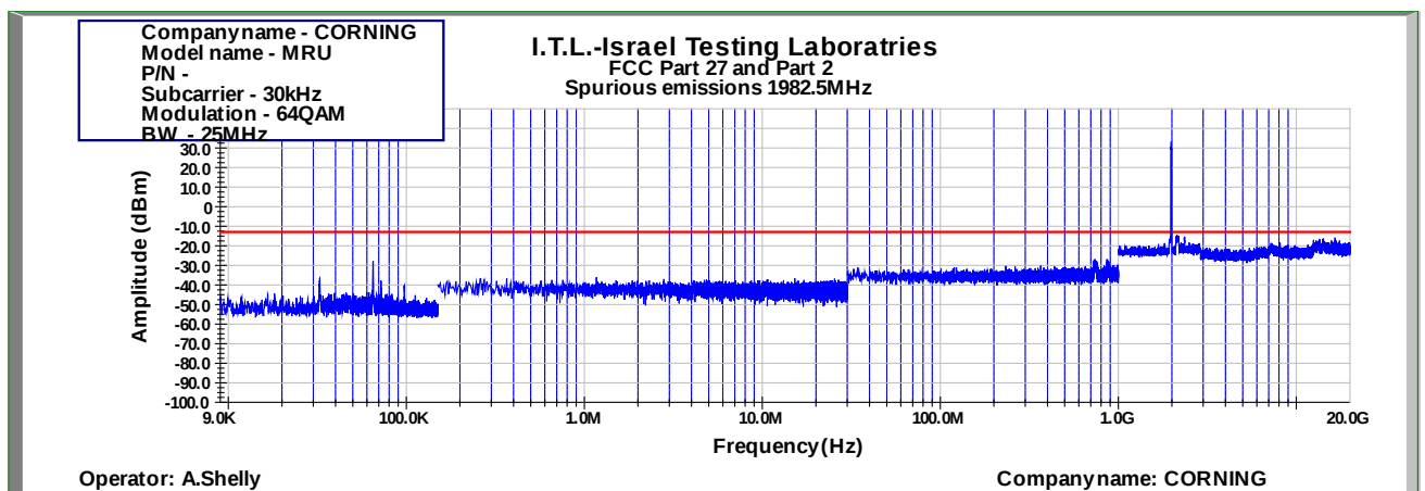
Figure 907: Spurious Emissions at Antenna Terminal 64QAM 25MHz B.W.; 1982.5MHz, 30kHz
