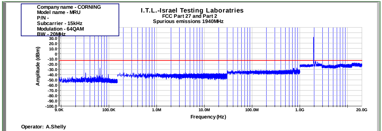
Figure 891: Spurious Emissions at Antenna Terminal 64QAM 20MHz B.W.; 1940.0MHz, 15kHz
