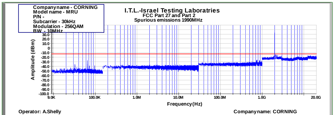
Figure 946: Spurious Emissions at Antenna Terminal 256QAM 10MHz B.W.; 1990.0MHz, 30kHz
