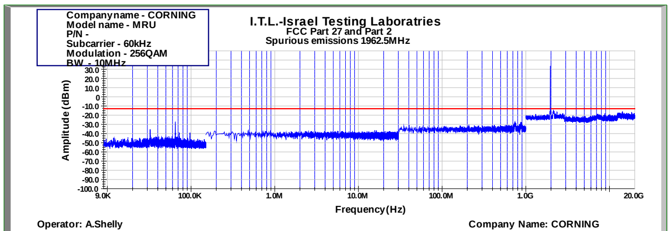
Figure 944: Spurious Emissions at Antenna Terminal 256QAM 10MHz B.W.; 1962.5MHz, 60kHz
