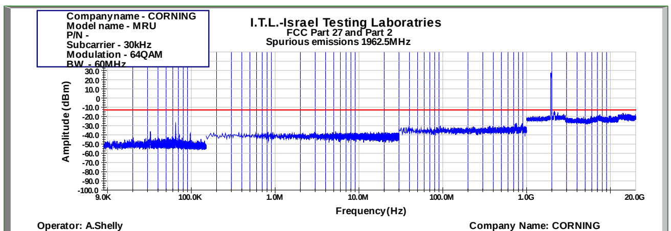
Figure 929: Spurious Emissions at Antenna Terminal 64QAM 60MHz B.W.; 1962.5MHz, 30kHz
