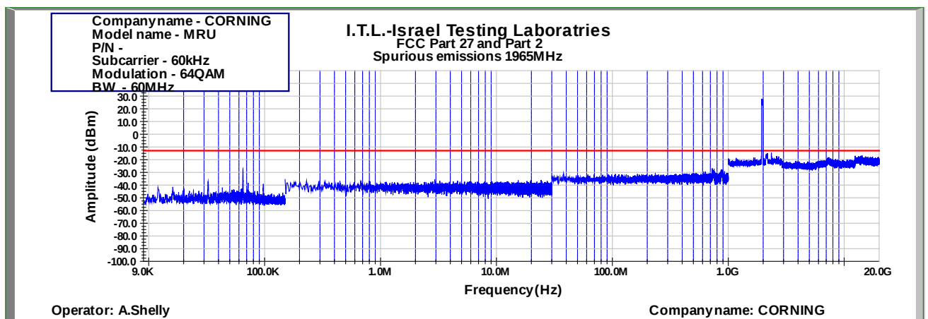
Figure 932: Spurious Emissions at Antenna Terminal 64QAM 60MHz B.W.; 1965.0MHz, 60kHz
