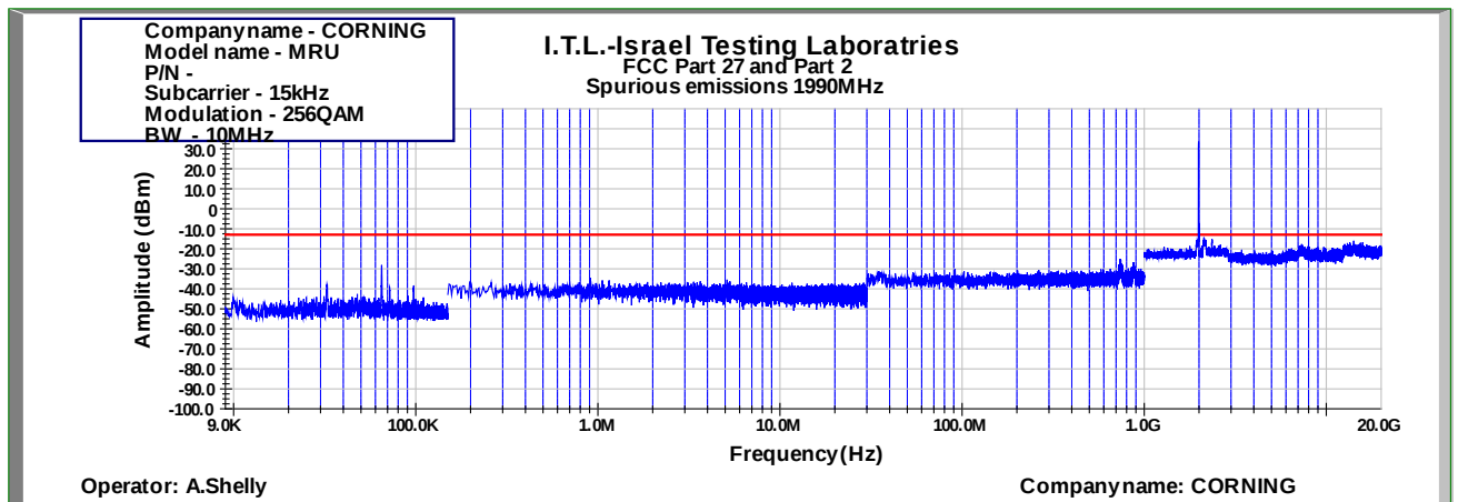
Figure 945: Spurious Emissions at Antenna Terminal 256QAM 10MHz B.W.; 1990.0MHz, 15kHz
