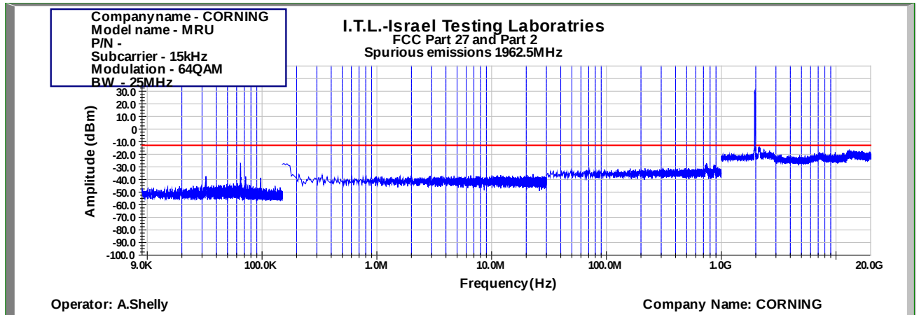
Figure 903: Spurious Emissions at Antenna Terminal 64QAM 25MHz B.W.; 1962.5MHz, 15kHz
