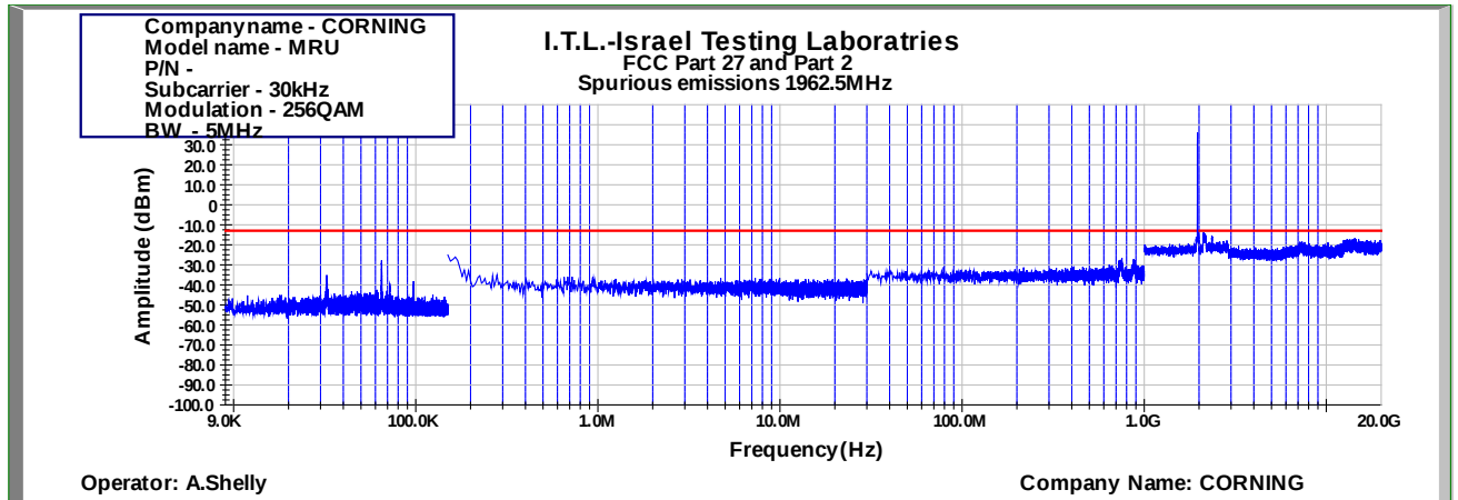
Figure 936: Spurious Emissions at Antenna Terminal 256QAM 5MHz B.W.; 1962.5MHz, 30kHz
