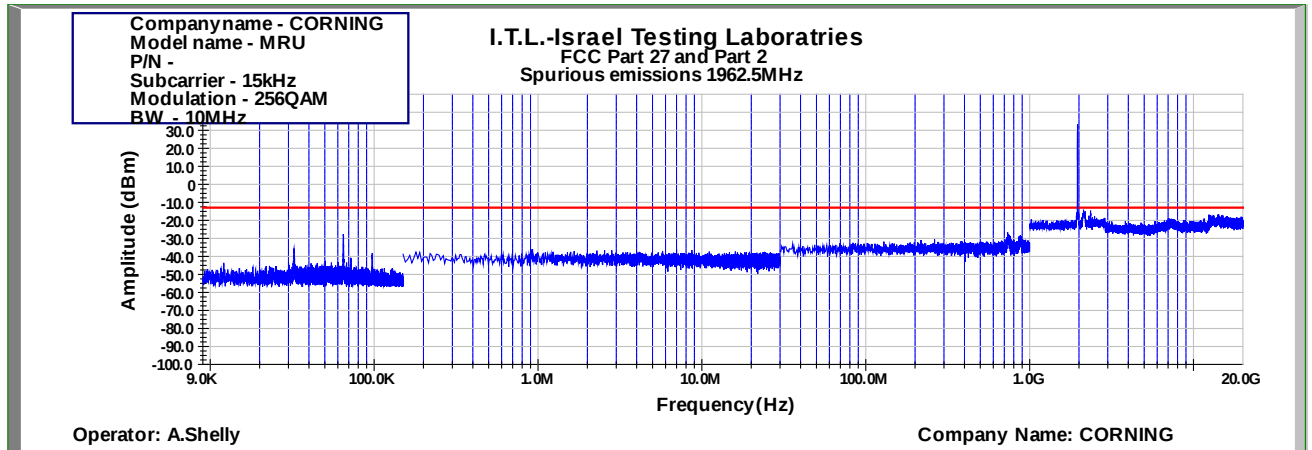
Figure 942: Spurious Emissions at Antenna Terminal 256QAM 10MHz B.W.; 1962.5MHz, 15kHz
