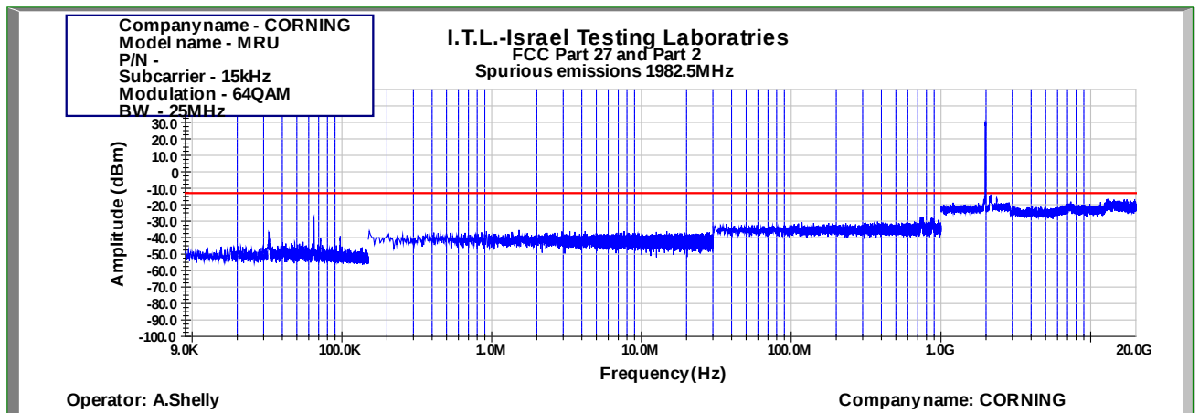
Figure 906: Spurious Emissions at Antenna Terminal 64QAM 25MHz B.W.; 1982.5MHz, 15kHz
