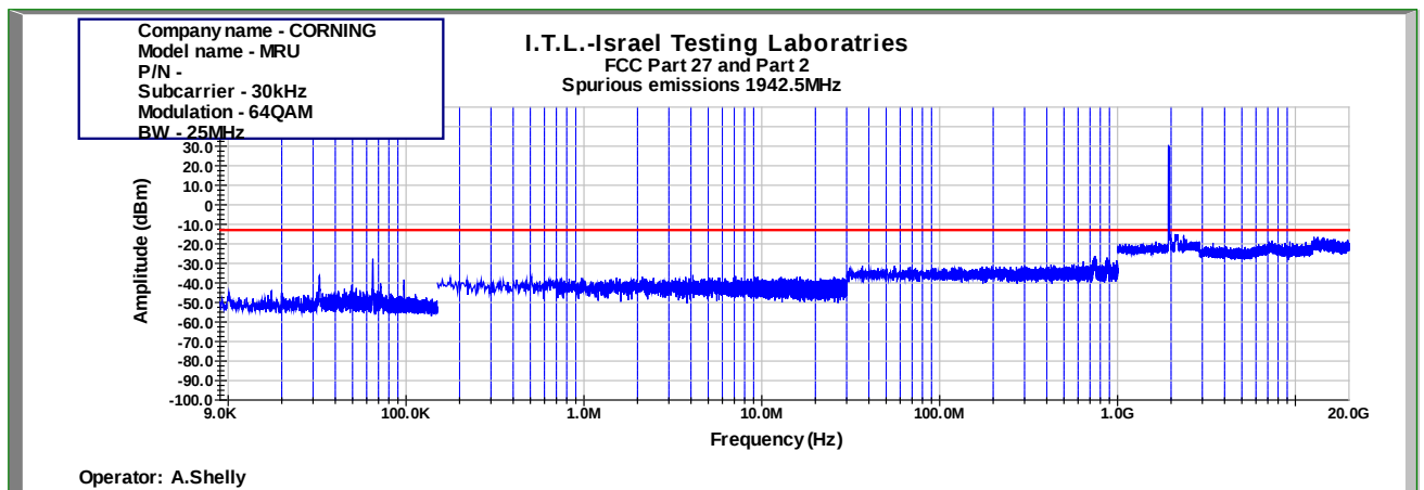
Figure 901: Spurious Emissions at Antenna Terminal 64QAM 25MHz B.W.; 1942.5MHz, 30kHz
