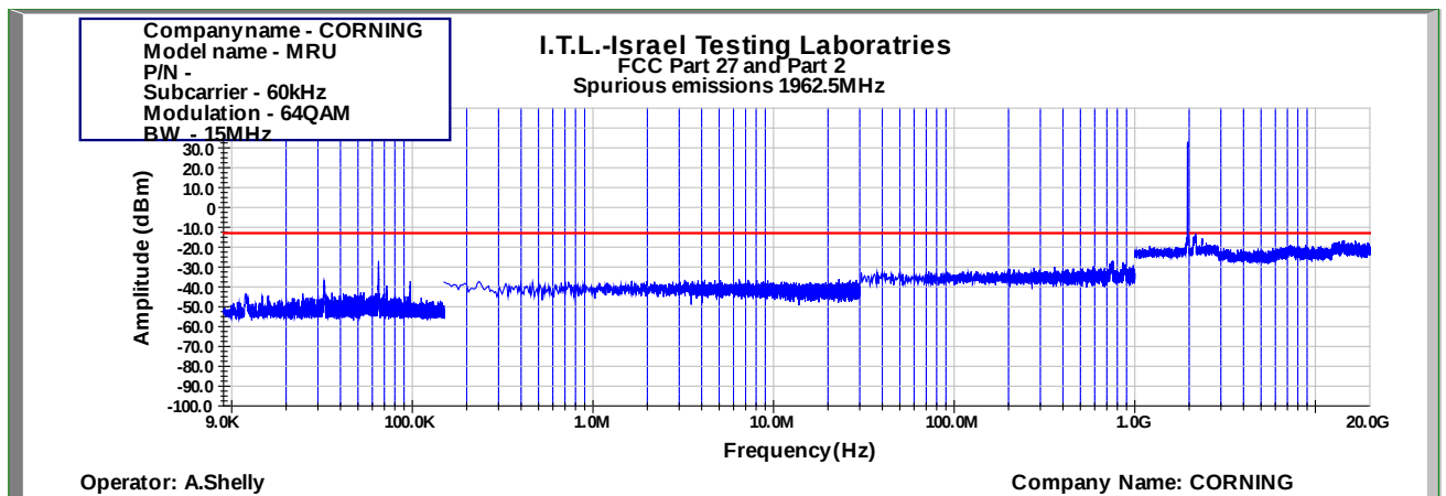
Figure 887: Spurious Emissions at Antenna Terminal 64QAM 15MHz B.W.; 1962.5MHz, 60kHz
