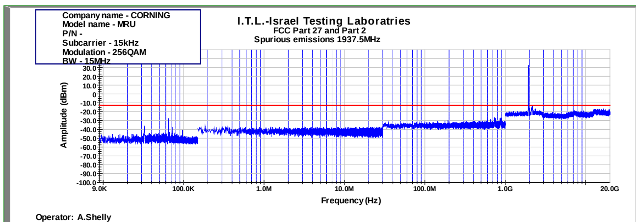
Figure 948: Spurious Emissions at Antenna Terminal 256QAM 15MHz B.W.; 1937.5MHz, 15kHz
