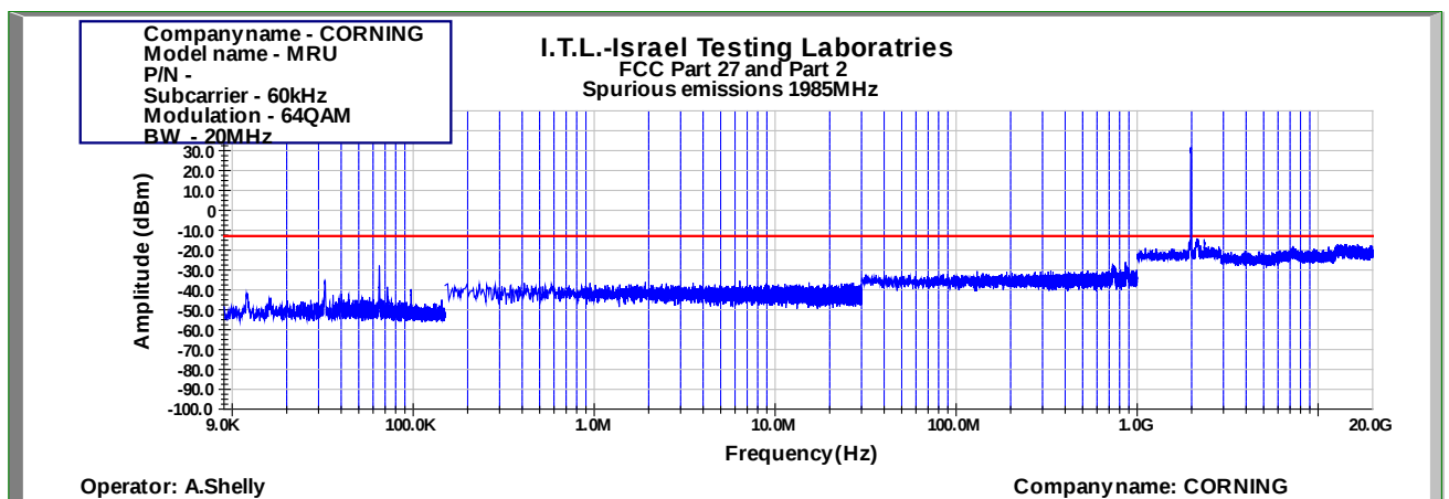
Figure 899: Spurious Emissions at Antenna Terminal 64QAM 20MHz B.W.; 1985.0MHz, 60kHz
