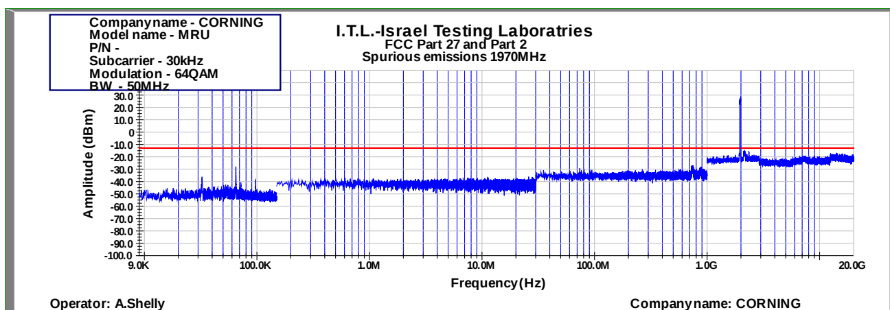
Figure 925: Spurious Emissions at Antenna Terminal 64QAM 50MHz B.W.; 1970.0MHz, 30kHz
