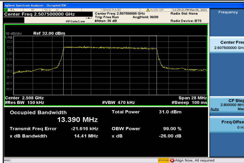
Band7-15MHz-QPSK-20825-75RB#0-13.390
