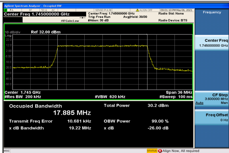
Band4-20MHz-16QAM-20300-100RB#0-17.885
