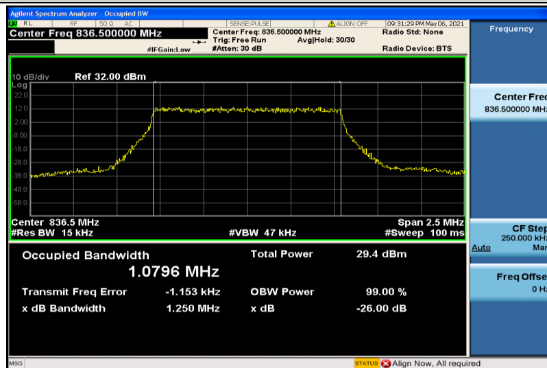
Band5-1.4MHz-QPSK-20525-6RB#0-1.0796
