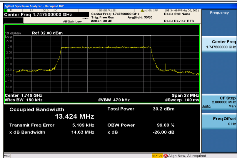
Band4-15MHz-16QAM-20325-75RB#0-13.424
