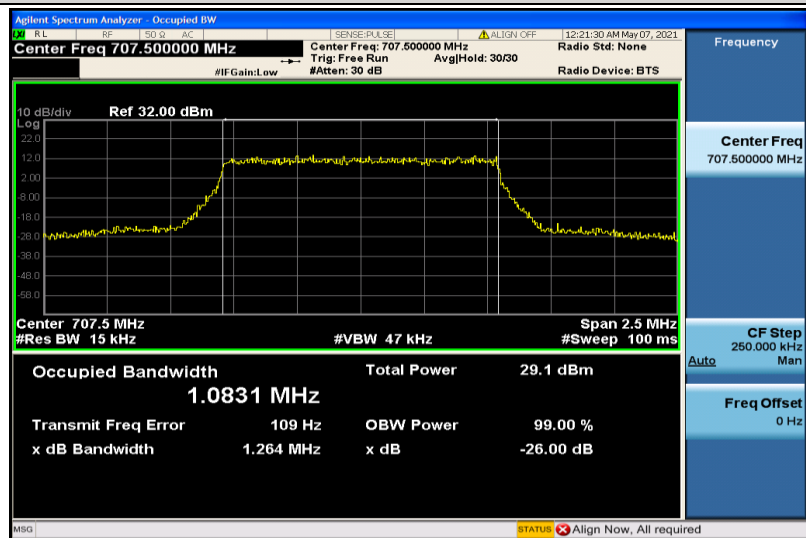
Band12-1.4MHz-16QAM-23095-6RB#0-1.0831
