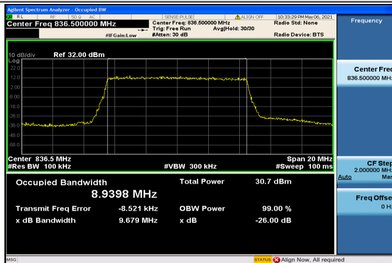
Band5-10MHz-QPSK-20525-50RB#0-8.9398
