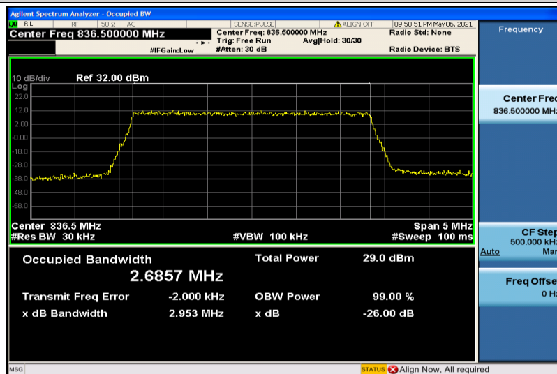
Band5-3MHz-16QAM-20525-15RB#0-2.6857
