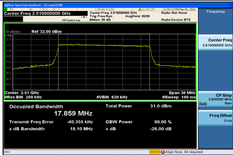
Band7-20MHz-QPSK-20850-100RB#0-17.859
