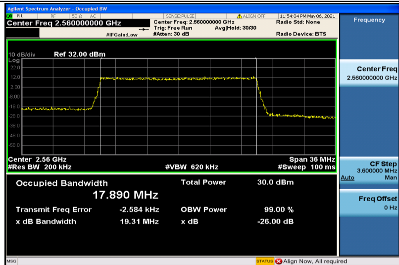
Band7-20MHz-16QAM-21350-100RB#0-17.890
