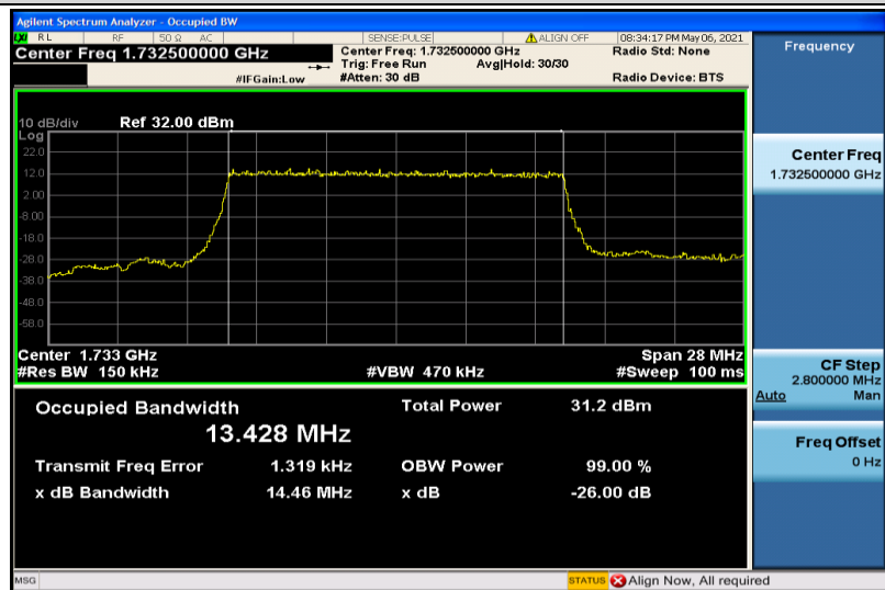
Band4-15MHz-QPSK-20175-75RB#0-13.428
