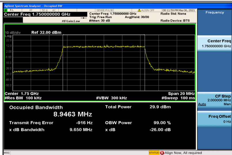
Band4-10MHz-16QAM-20350-50RB#0-8.9463
