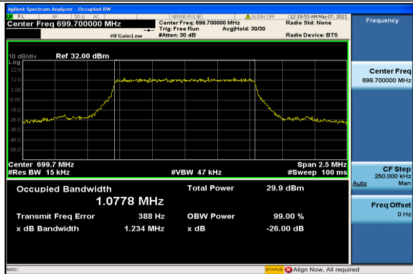
Band12-1.4MHz-QPSK-23017-6RB#0-1.0778
