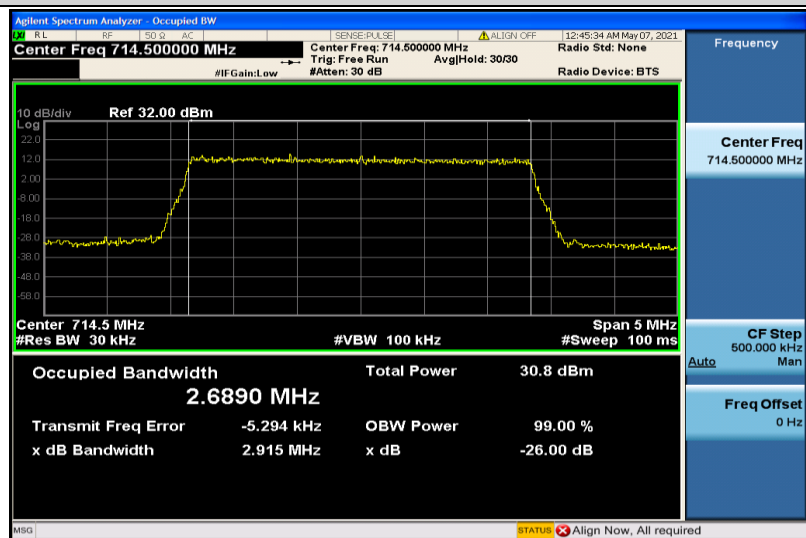
Band12-3MHz-QPSK-23165-15RB#0-2.6890
