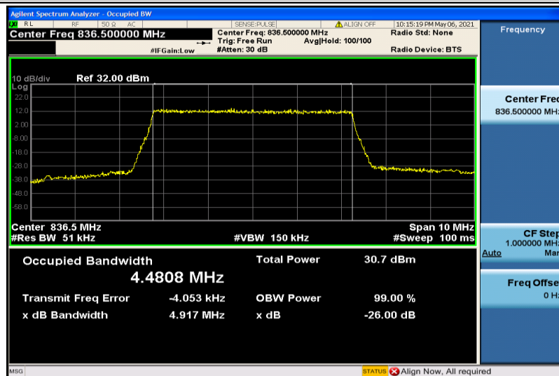
Band5-5MHz-QPSK-20525-25RB#0-4.4808
