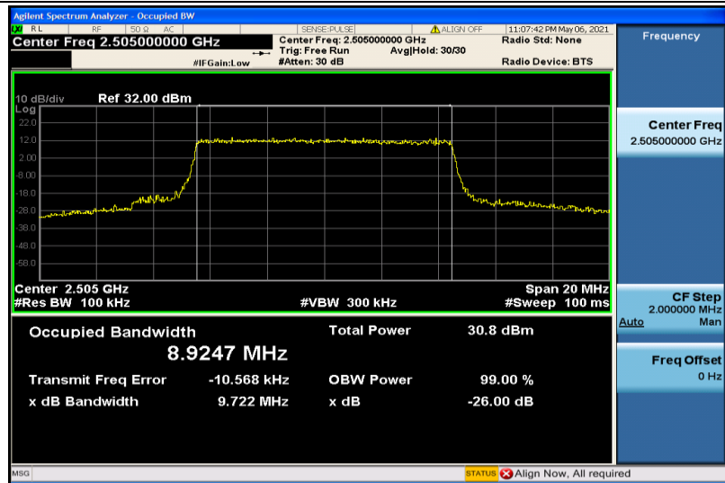
Band7-10MHz-QPSK-20800-50RB#0-8.9247
