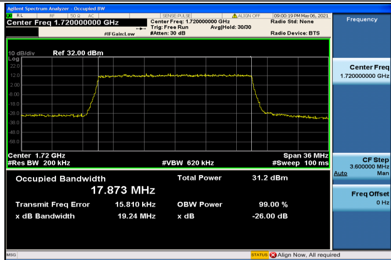
Band4-20MHz-QPSK-20050-100RB#0-17.873
