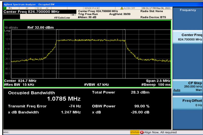
Band5-1.4MHz-16QAM-20407-6RB#0-1.0785
