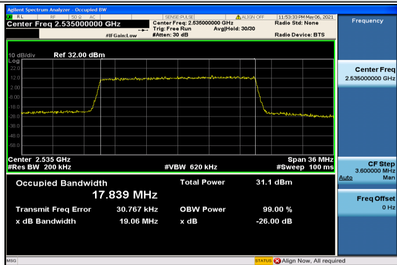
Band7-20MHz-QPSK-21100-100RB#0-17.839
