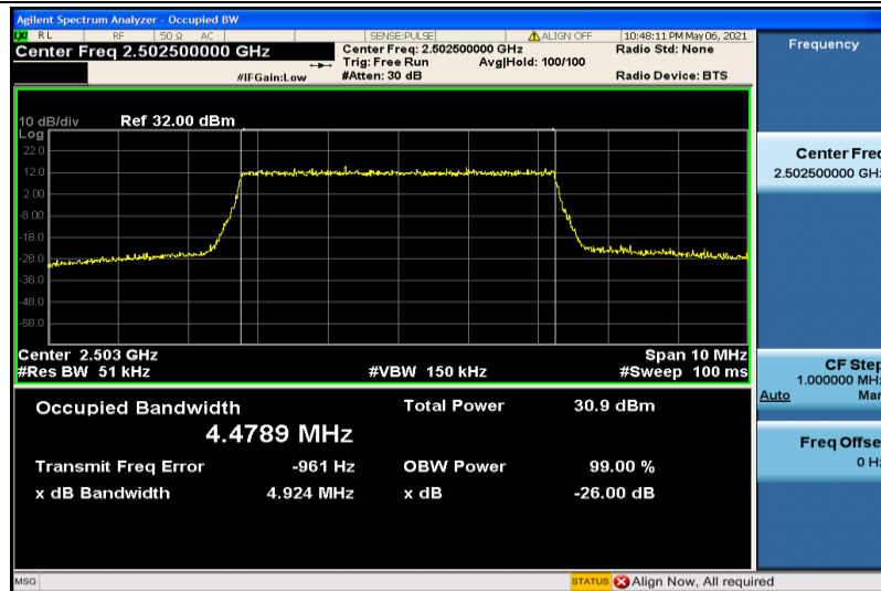
Band7-5MHz-QPSK-20775-25RB#0-4.4789
