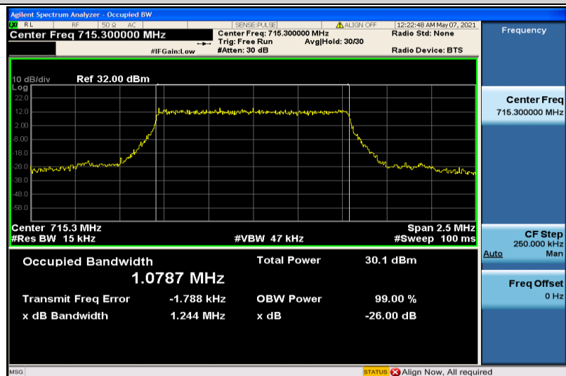
Band12-1.4MHz-QPSK-23173-6RB#0-1.0787
