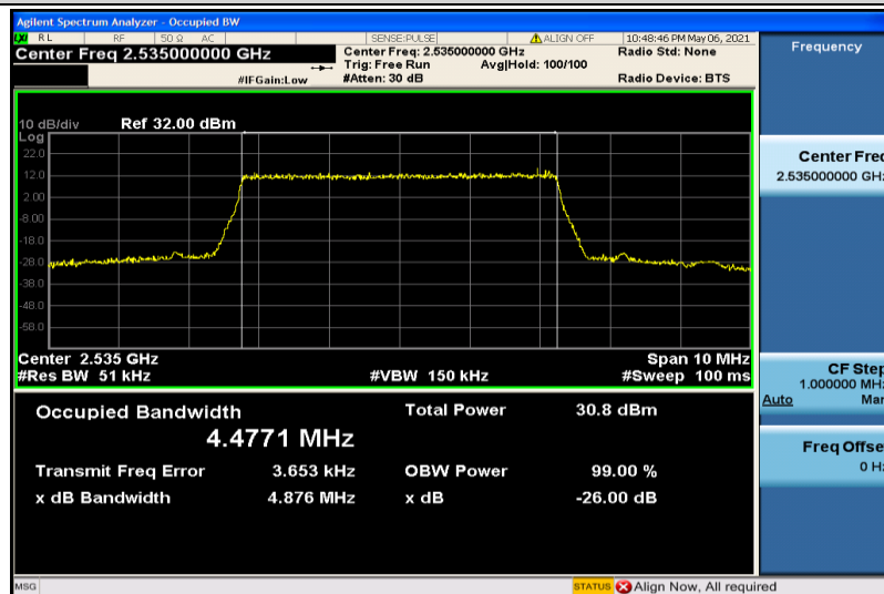
Band7-5MHz-QPSK-21100-25RB#0-4.4771
