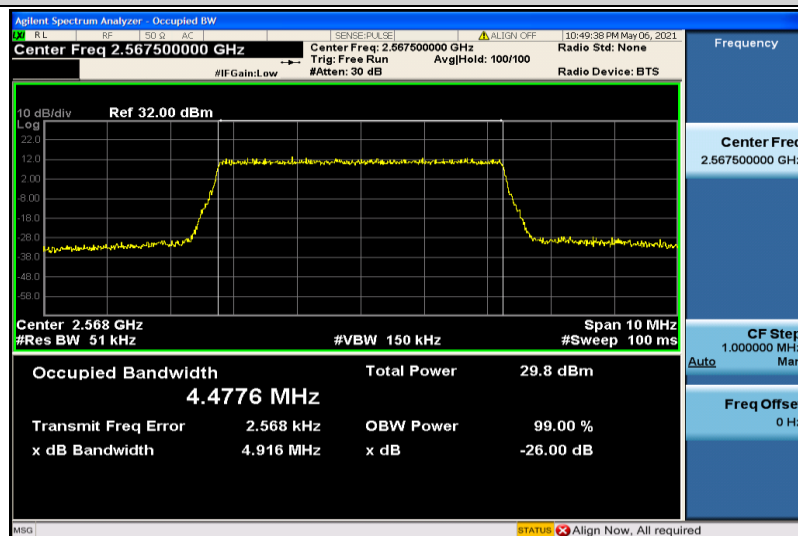
Band7-5MHz-16QAM-21425-25RB#0-4.4776
