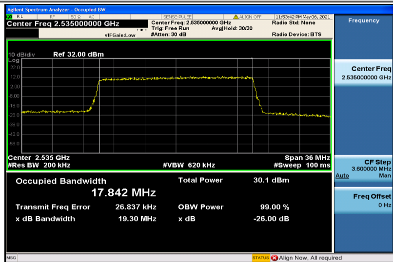
Band7-20MHz-16QAM-21100-100RB#0-17.842
