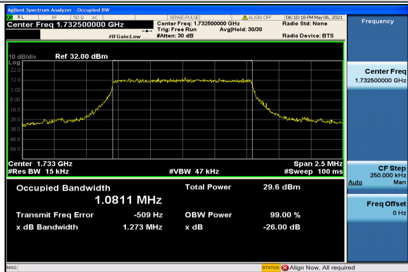
Band4-1.4MHz-QPSK-20175-6RB#0-1.0811
