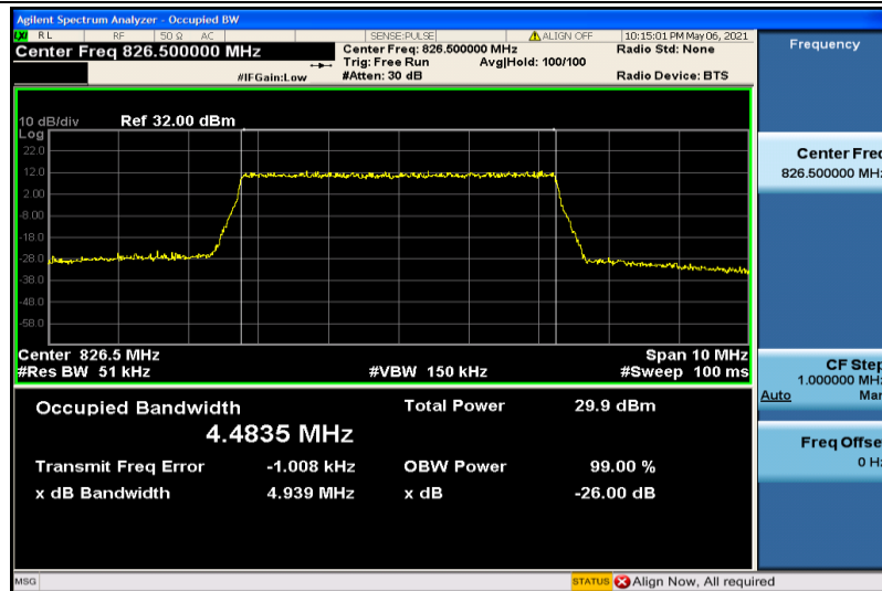
Band5-5MHz-16QAM-20425-25RB#0-4.4835
