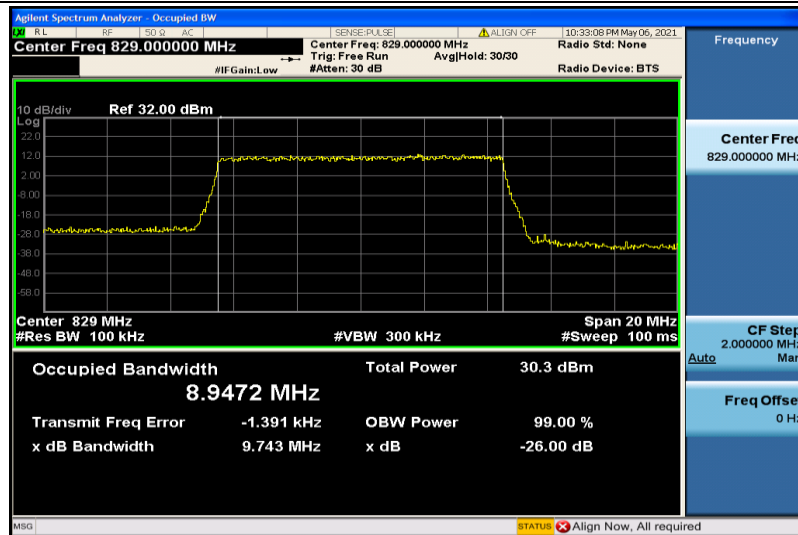
Band5-10MHz-QPSK-20450-50RB#0-8.9472
