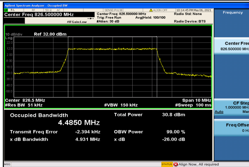
Band5-5MHz-QPSK-20425-25RB#0-4.4850
