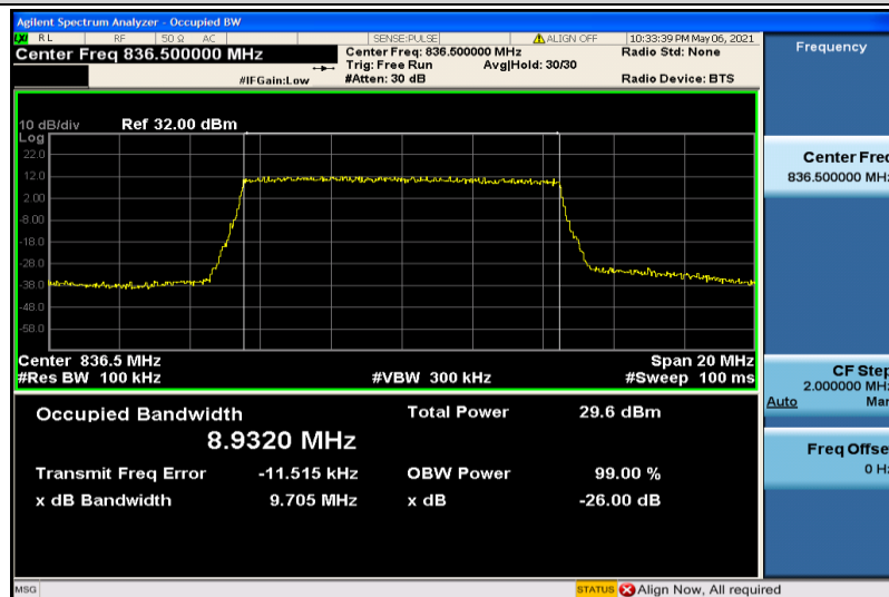
Band5-10MHz-16QAM-20525-50RB#0-8.9320
