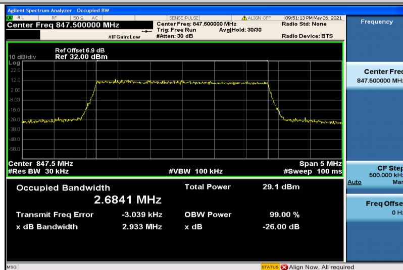
Band5-3MHz-16QAM-20635-15RB#0-2.6841
