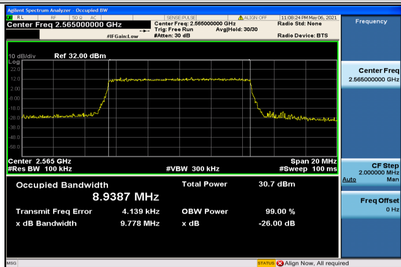
Band7-10MHz-QPSK-21400-50RB#0-8.9387
