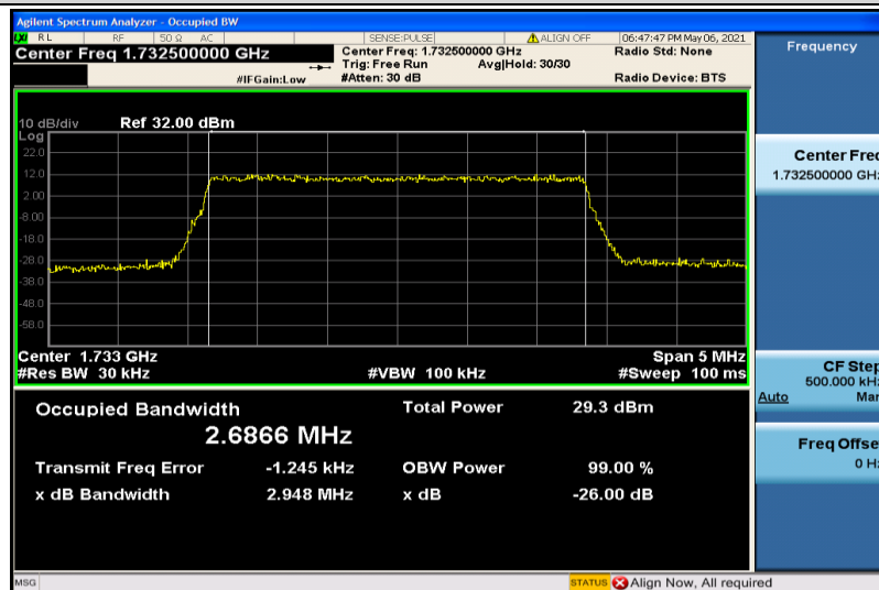
Band4-3MHz-QPSK-20175-15RB#0-2.6866
