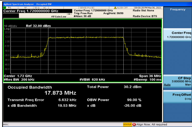
Band4-20MHz-16QAM-20050-100RB#0-17.873
