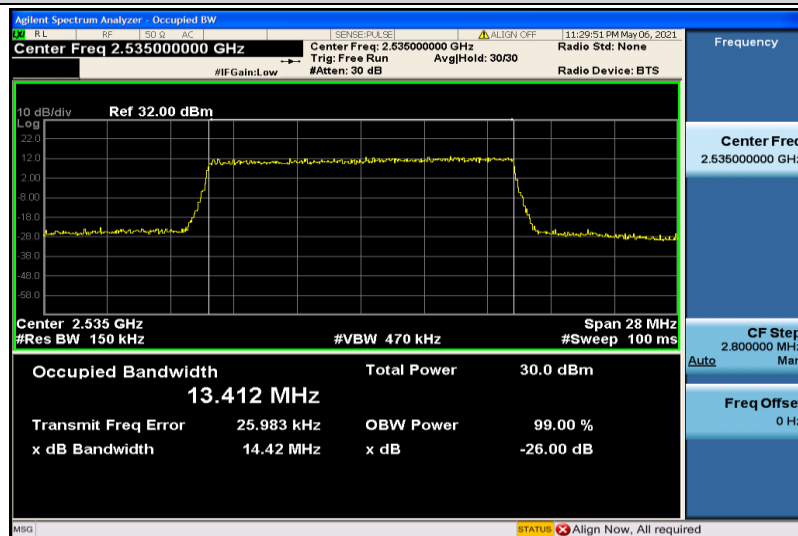
Band7-15MHz-16QAM-21100-75RB#0-13.412
