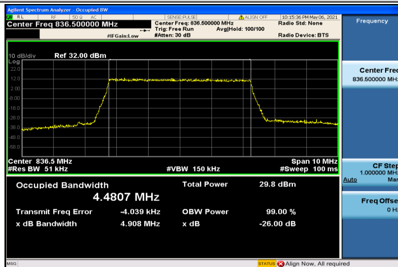
Band5-5MHz-16QAM-20525-25RB#0-4.4807
