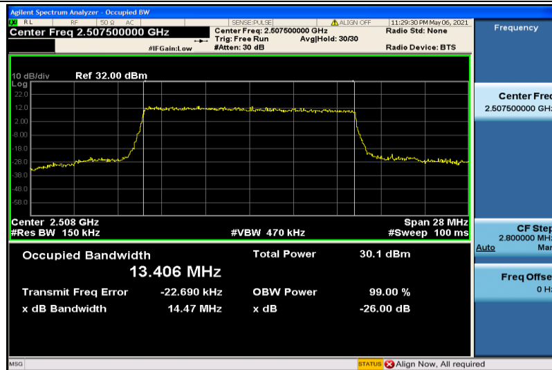
Band7-15MHz-16QAM-20825-75RB#0-13.406
