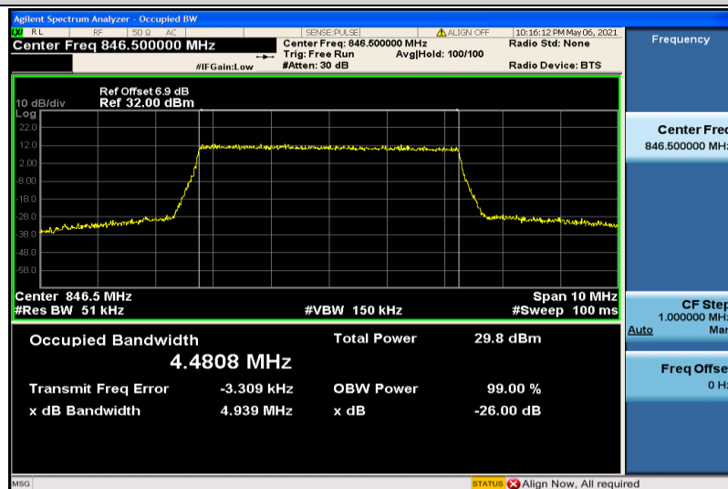
Band5-5MHz-16QAM-20625-25RB#0-4.4808
