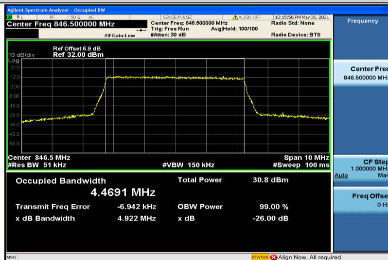
Band5-5MHz-QPSK-20625-25RB#0-4.4691
