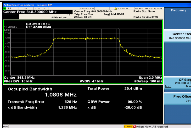
Band5-1.4MHz-QPSK-20643-6RB#0-1.0806
