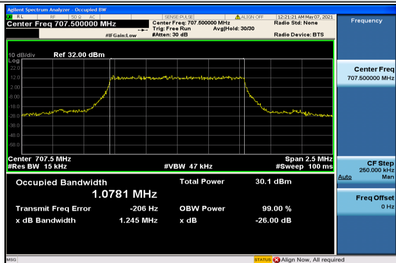
Band12-1.4MHz-QPSK-23095-6RB#0-1.0781
