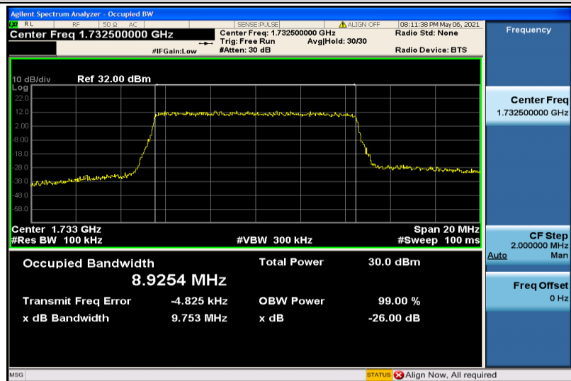
Band4-10MHz-16QAM-20175-50RB#0-8.9254
