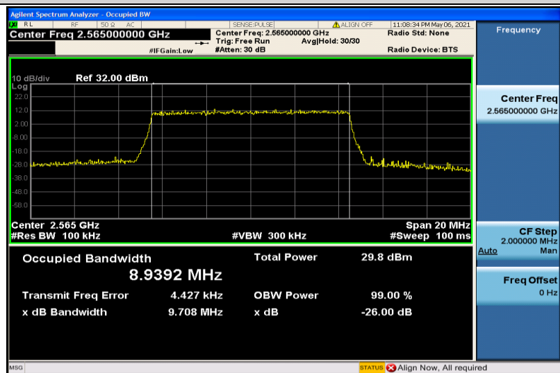
Band7-10MHz-16QAM-21400-50RB#0-8.9392
