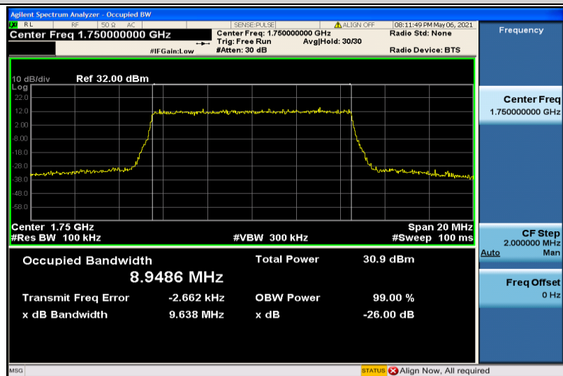
Band4-10MHz-QPSK-20350-50RB#0-8.9486
