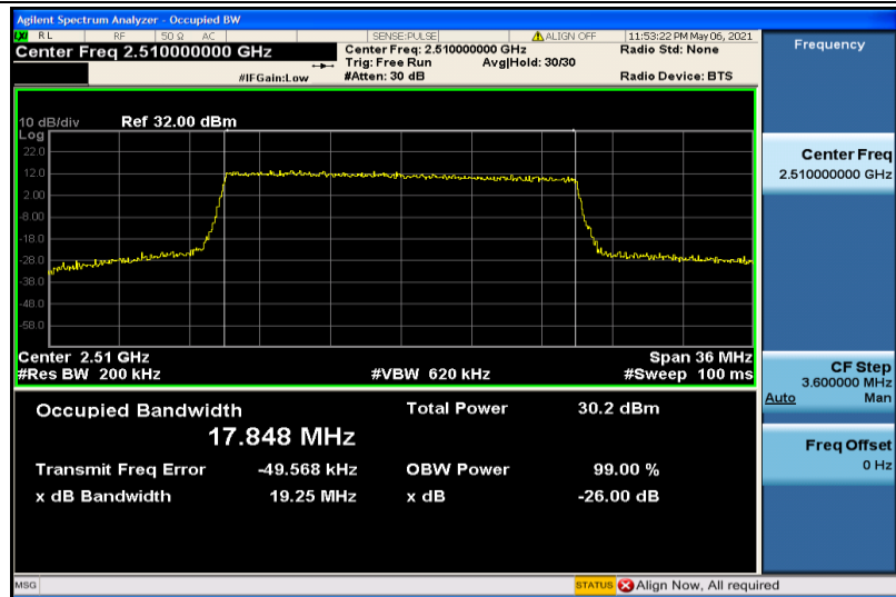
Band7-20MHz-16QAM-20850-100RB#0-17.848
