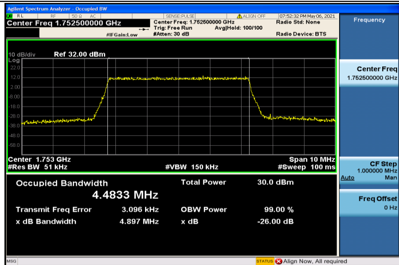
Band4-5MHz-16QAM-20375-25RB#0-4.4833
