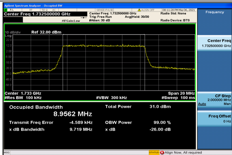
Band4-10MHz-QPSK-20175-50RB#0-8.9562
