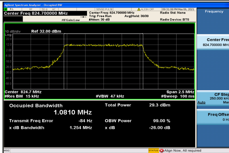
Band5-1.4MHz-QPSK-20407-6RB#0-1.0810
