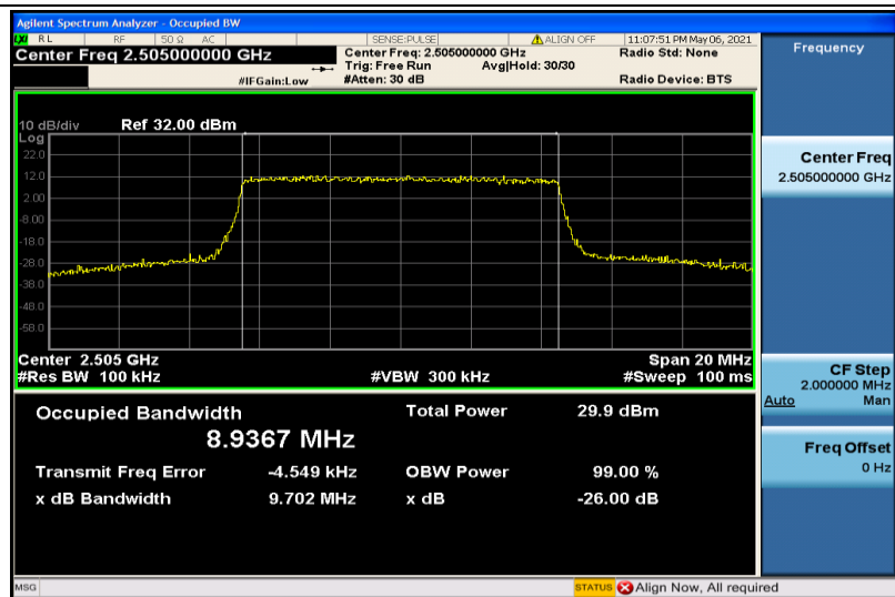
Band7-10MHz-16QAM-20800-50RB#0-8.9367
