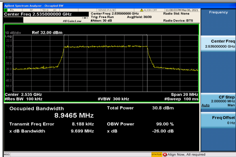
Band7-10MHz-QPSK-21100-50RB#0-8.9465
