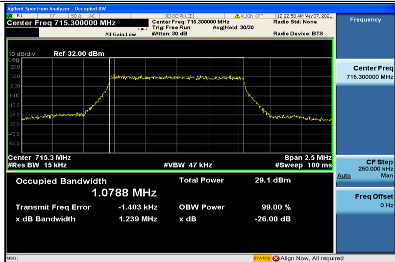
Band12-1.4MHz-16QAM-23173-6RB#0-1.0788
