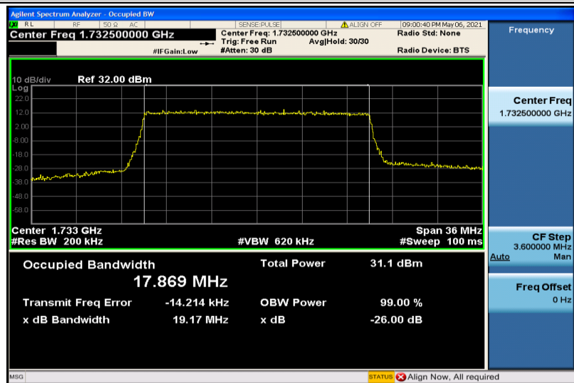
Band4-20MHz-QPSK-20175-100RB#0-17.869
