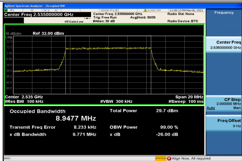
Band7-10MHz-16QAM-21100-50RB#0-8.9477
