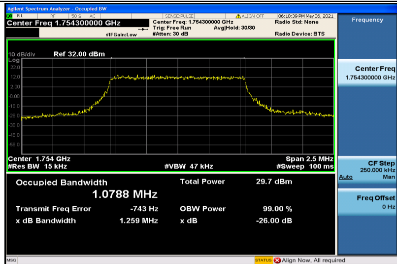
Band4-1.4MHz-QPSK-20393-6RB#0-1.0788
