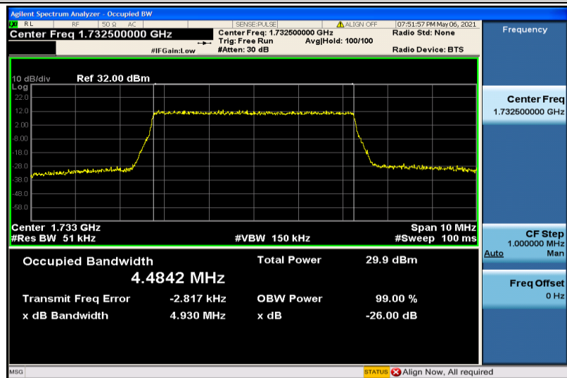
Band4-5MHz-16QAM-20175-25RB#0-4.4842
