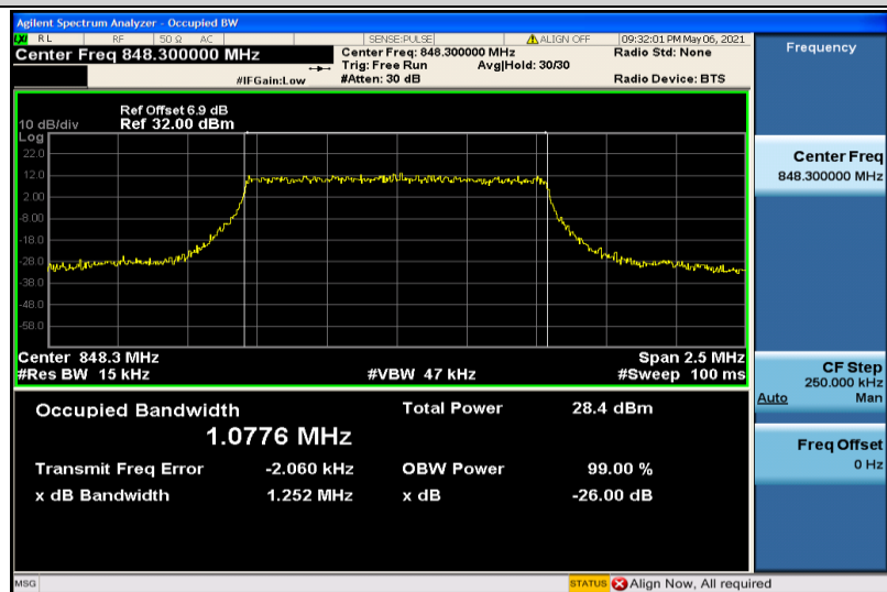
Band5-1.4MHz-16QAM-20643-6RB#0-1.0776
