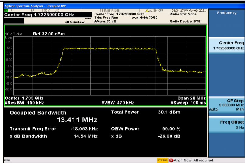
Band4-15MHz-16QAM-20175-75RB#0-13.411
