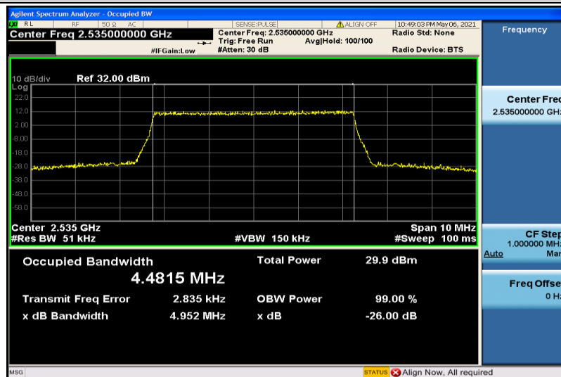
Band7-5MHz-16QAM-21100-25RB#0-4.4815
