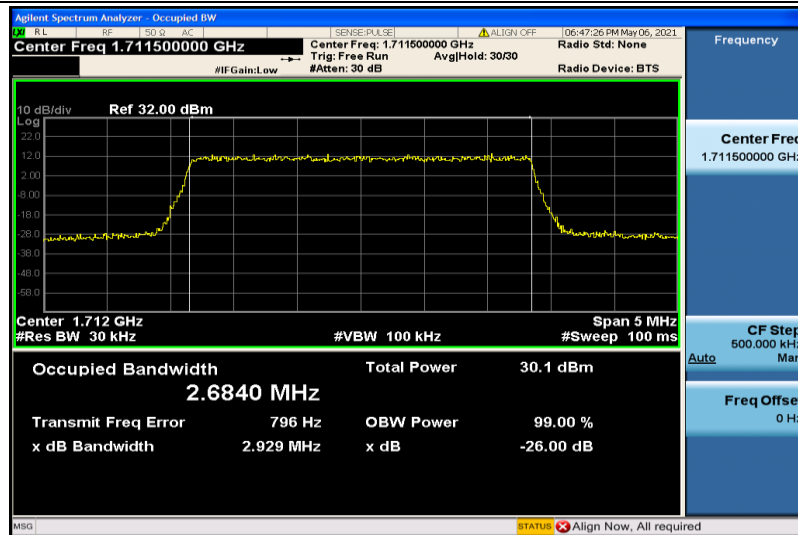
Band4-3MHz-QPSK-19965-15RB#0-2.6840
