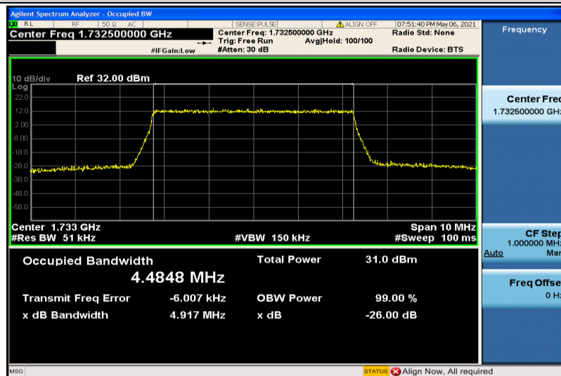
Band4-5MHz-QPSK-20175-25RB#0-4.4848
