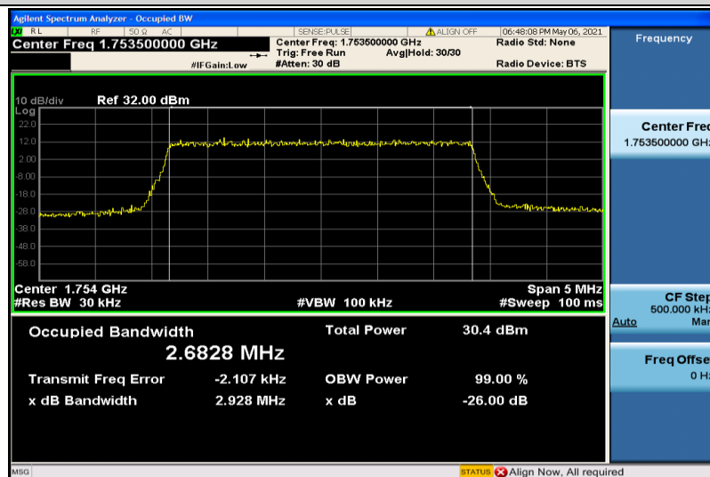
Band4-3MHz-QPSK-20385-15RB#0-2.6828
