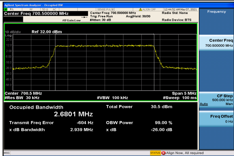
Band12-3MHz-QPSK-23025-15RB#0-2.6801
