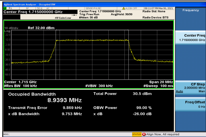
Band4-10MHz-QPSK-20000-50RB#0-8.9393
