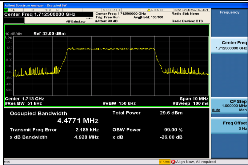
Band4-5MHz-16QAM-19975-25RB#0-4.4771
