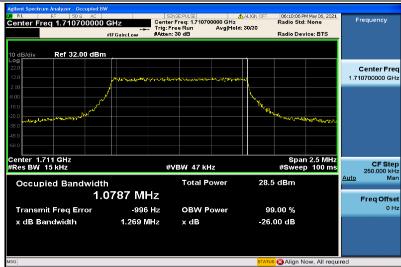
Band4-1.4MHz-16QAM-19957-6RB#0-1.0787
