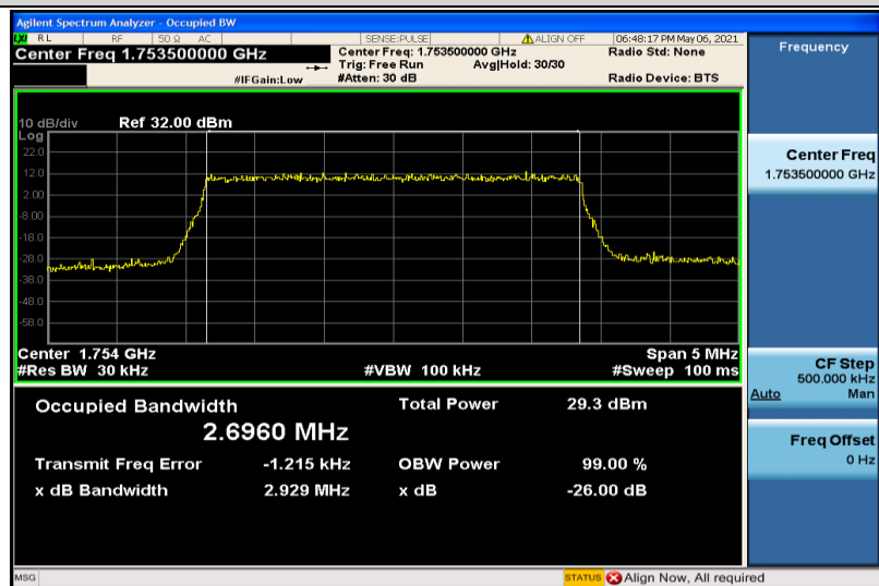
Band4-3MHz-16QAM-20385-15RB#0-2.6960
