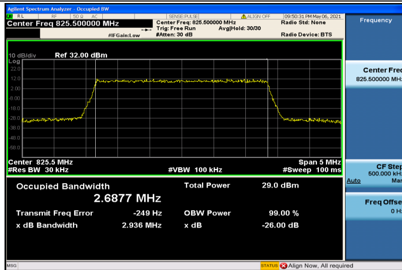
Band5-3MHz-16QAM-20415-15RB#0-2.6877
