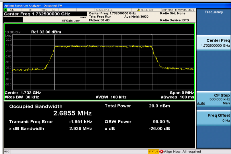
Band4-3MHz-16QAM-20175-15RB#0-2.6855
