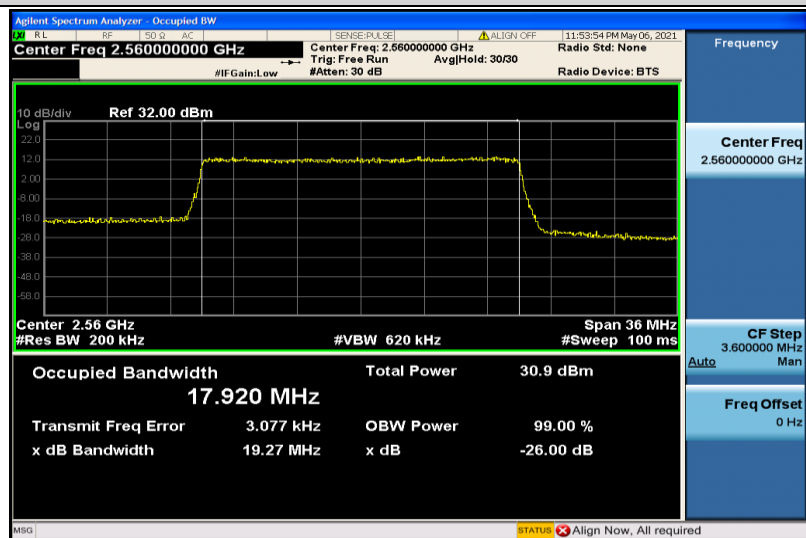
Band7-20MHz-QPSK-21350-100RB#0-17.920
