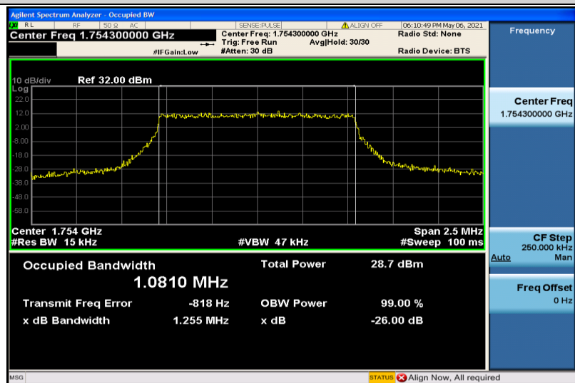
Band4-1.4MHz-16QAM-20393-6RB#0-1.0810
