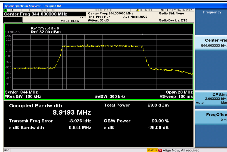
Band5-10MHz-16QAM-20600-50RB#0-8.9193
