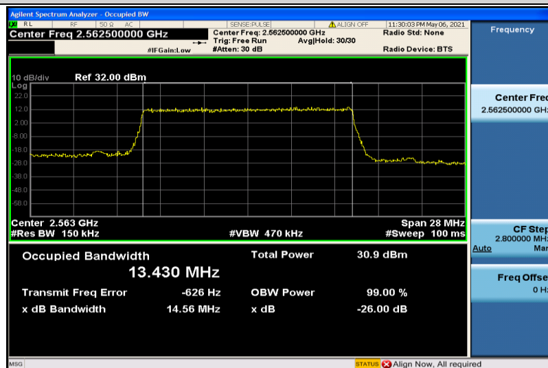
Band7-15MHz-QPSK-21375-75RB#0-13.430
