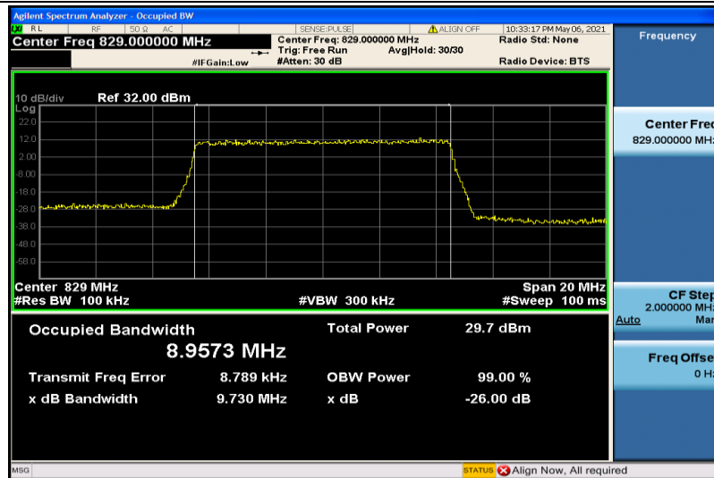
Band5-10MHz-16QAM-20450-50RB#0-8.9573
