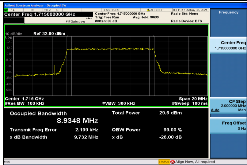
Band4-10MHz-16QAM-20000-50RB#0-8.9348
