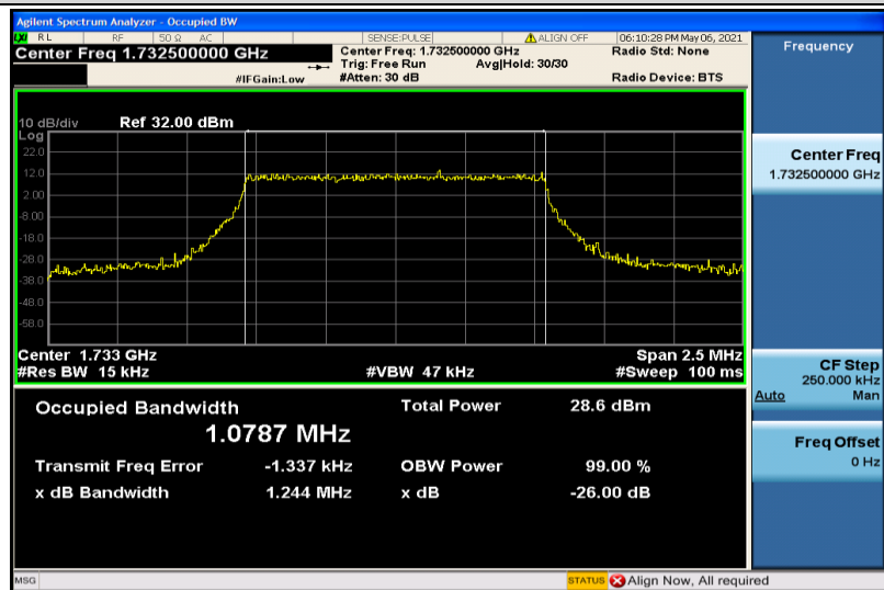
Band4-1.4MHz-16QAM-20175-6RB#0-1.0787
