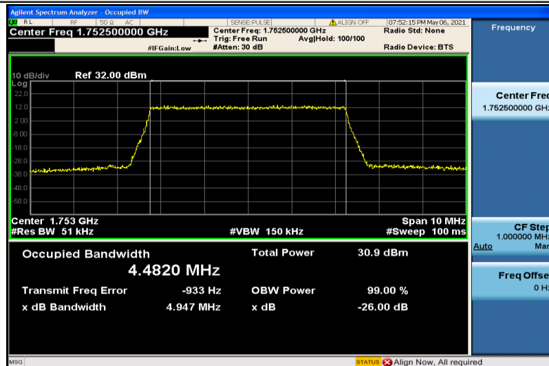
Band4-5MHz-QPSK-20375-25RB#0-4.4820
