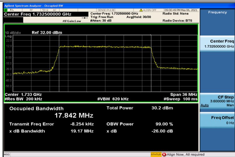
Band4-20MHz-16QAM-20175-100RB#0-17.842
