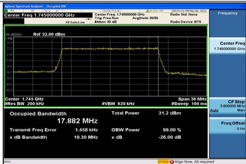
Band4-20MHz-QPSK-20300-100RB#0-17.882
