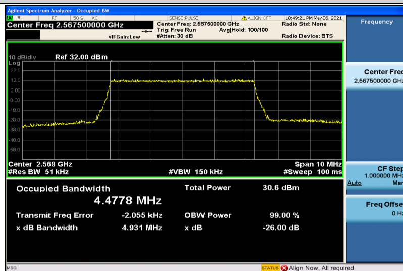
Band7-5MHz-QPSK-21425-25RB#0-4.4778
