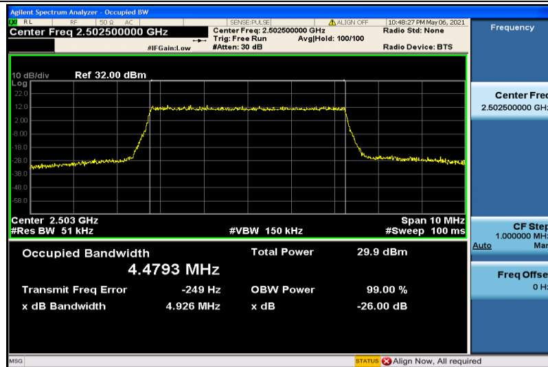
Band7-5MHz-16QAM-20775-25RB#0-4.4793
