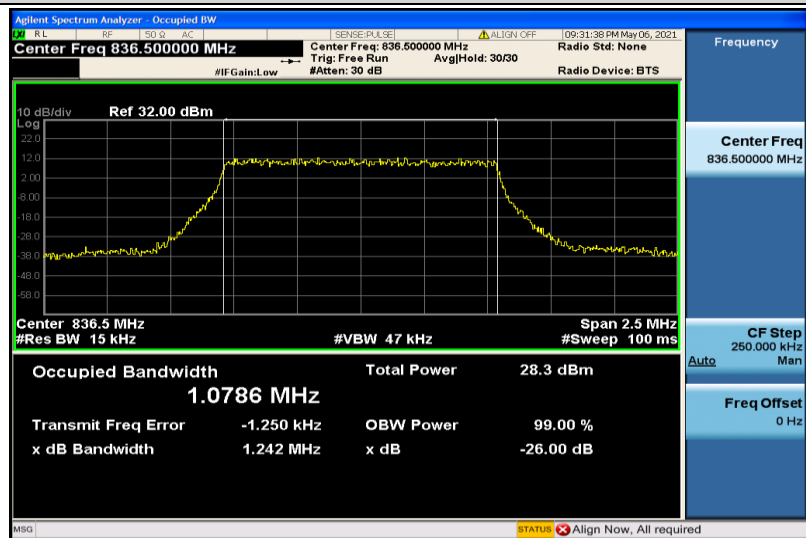
Band5-1.4MHz-16QAM-20525-6RB#0-1.0786
