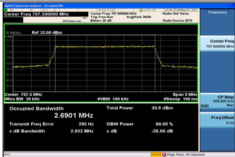
Band12-3MHz-QPSK-23095-15RB#0-2.6901
