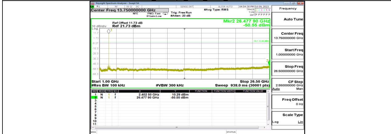
BLE_125kbps_Ant5_2402_1000~26500
