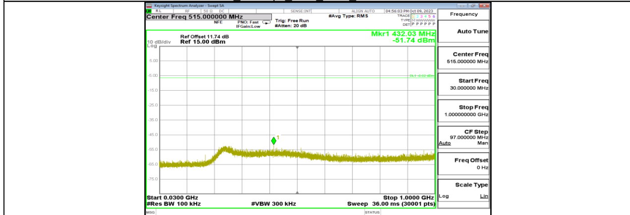
BLE_125kbps_Ant5_2440_0~Reference
