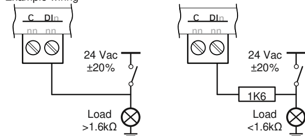
Example wiring
